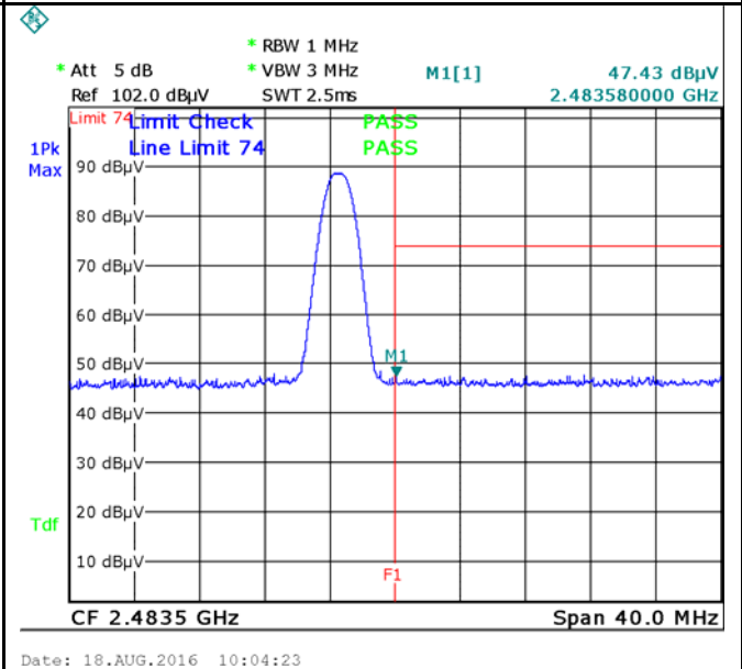
GFSK-Right Side-PK Note: F1 is frequency 2483.5MHz
