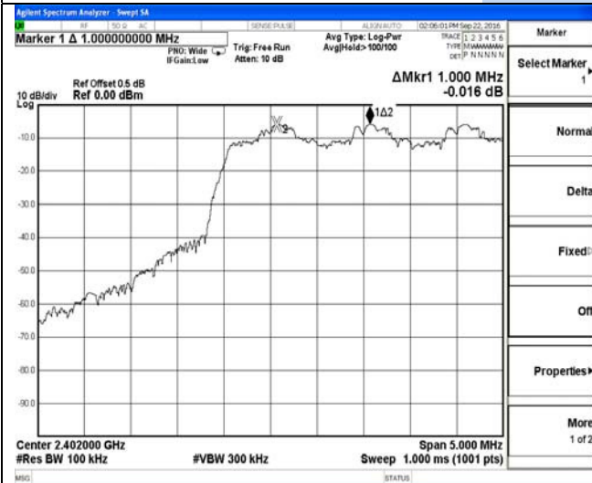
Frequency Separation \pi/4 -DQPSK-Low channel
