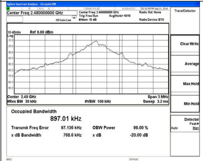
20dB Bandwidth GFSK-High channel
