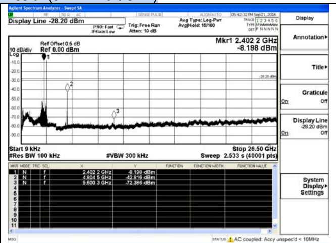
2DH1-Low channel
