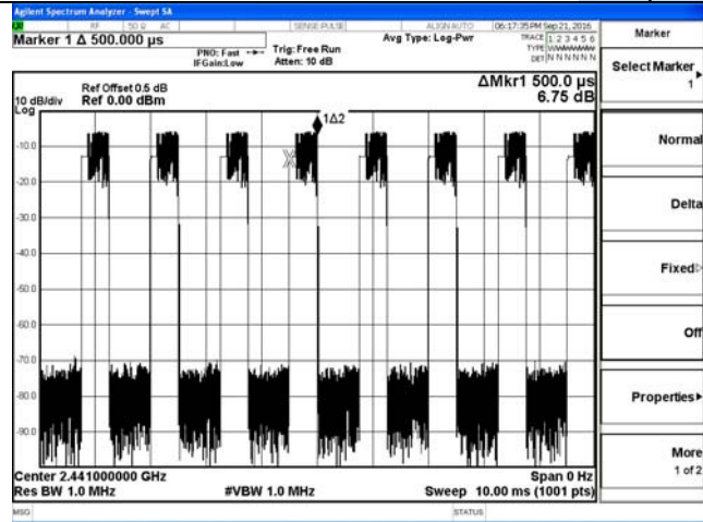
3DH1-2441MHz
