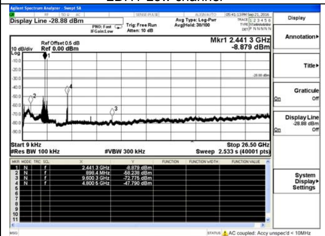
2DH1-Middle channel
