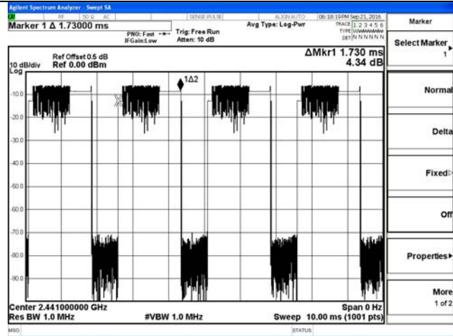
3DH3-2441MHz
