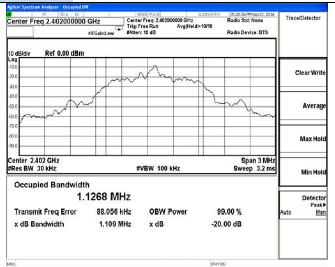
20dB Bandwidth \pi/4 -DQPSK-Low channel
