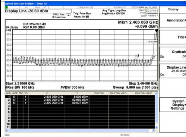
Hopping On-8-DPSK-Low channel
