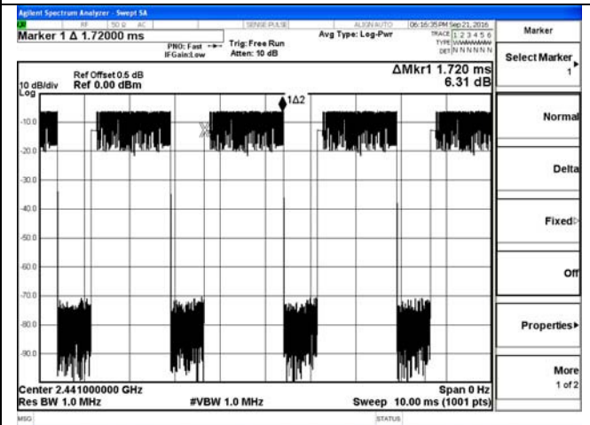
2DH3-2441MHz
