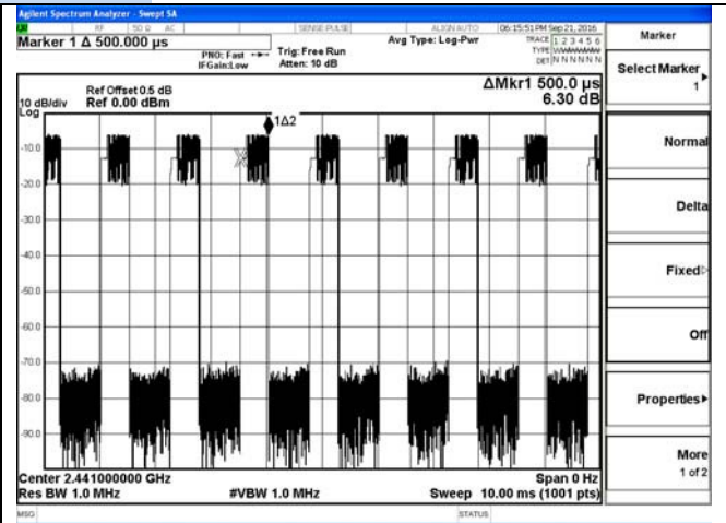
2DH1-2441MHz
