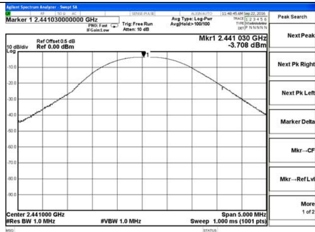
DH1-Middle channel
