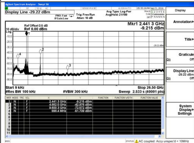
3DH1-Middle channel
