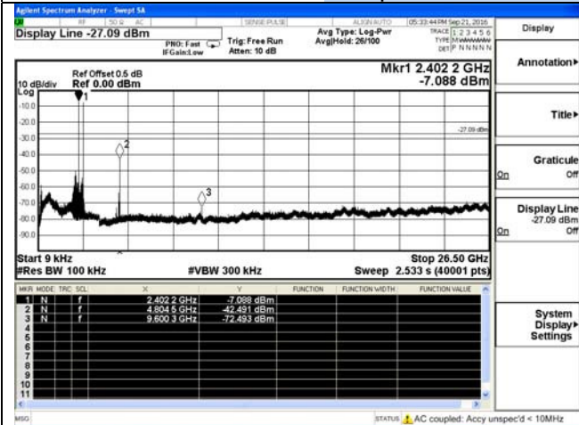
3DH1-Low channel
