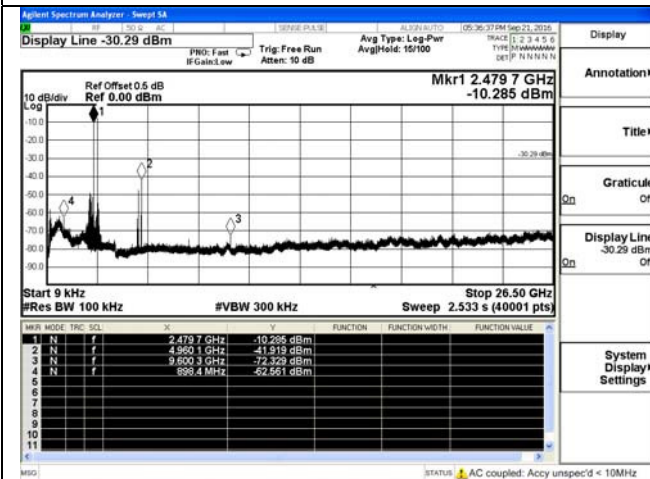
3DH1-High channel
