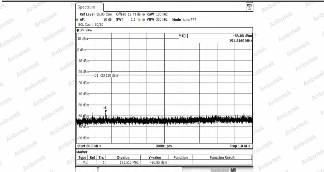
DH5-Ant1-2480-30~1000-PASS
