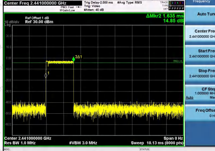
3DH3-Ant1-Hop-PASS
