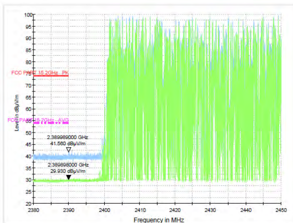
Test Mode: GFSK-Low Hopping-on Polarization: Vertical
