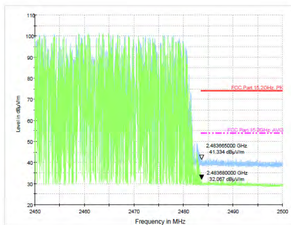
Test Mode: GFSK-High Hopping-on Polarization: Horizontal
