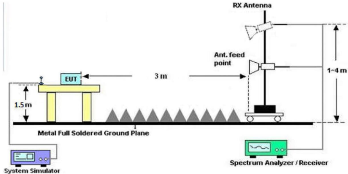
Figure 3. Above 1 GHz
