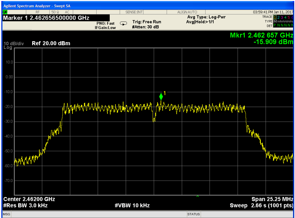
Channel 11:2.462 GHz:
