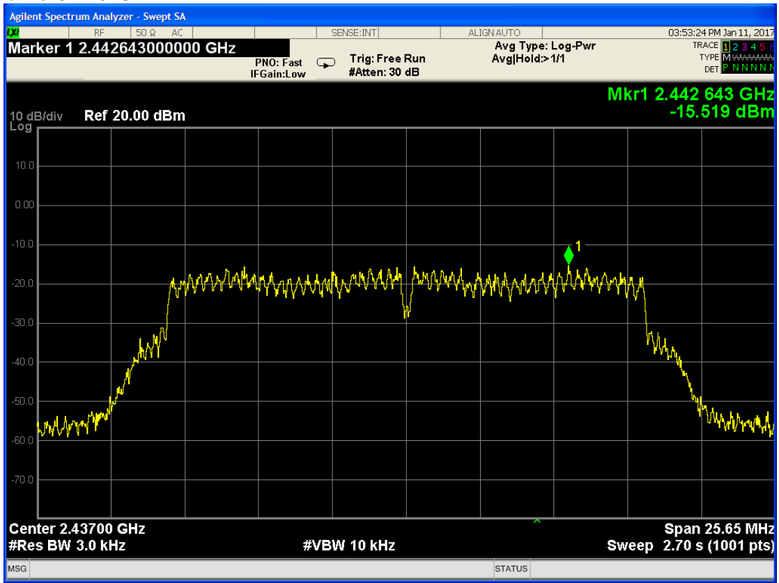
Channel 6:2.437GHz:
