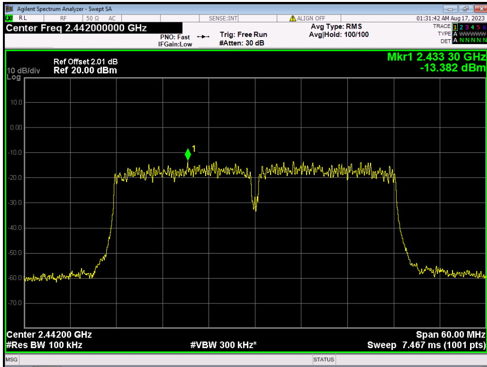
Channel 7: 2.442GHz:
