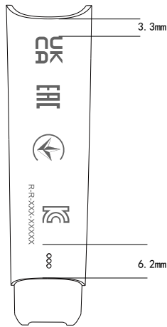
耳机支臂
