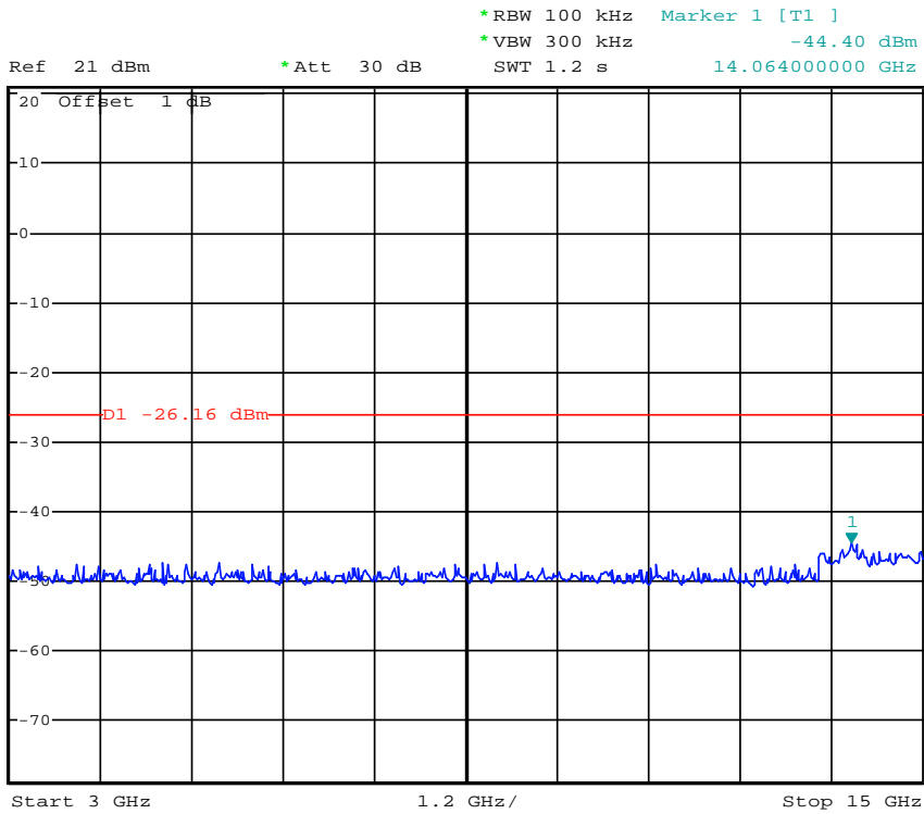
(Plot 4.6.4 C1: Channel 9: 2452MHz @ 802.11n(20MHz))
