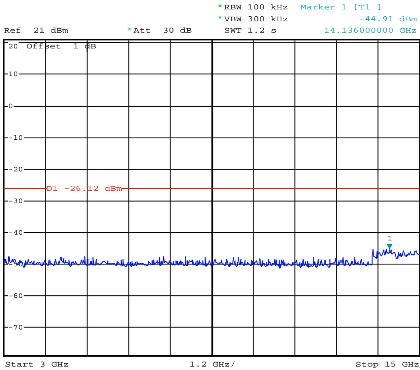
(Plot 4.6.4 A1: Channel 3: 2422MHz @ 802.11n(20MHz))
