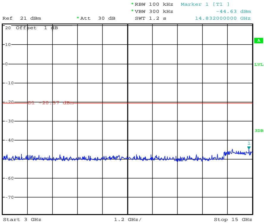
(Plot 4.6.3 A1: Channel 1: 2412MHz @ 802.11n(20MHz))
