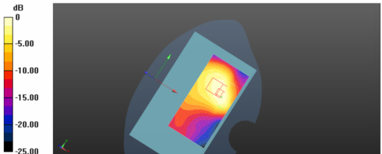
Figure 1: Body- worn Back-802.11b -Channel 1-2412MHz(1Mbps)
