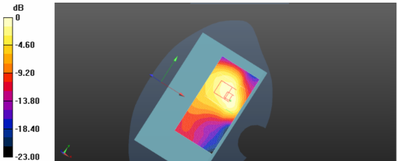
Plot 2: Body- worn Back-802.11b-Channel 6-2437MHz(1Mbps)
