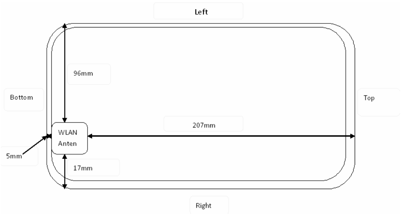
Position of the antennas
