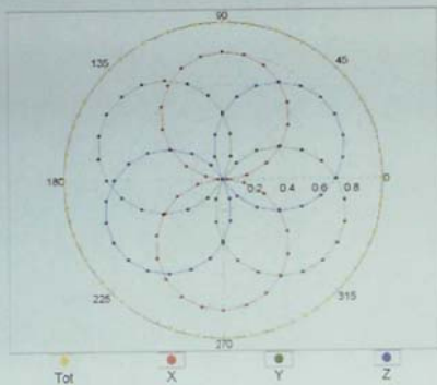
f=600 MHz,TEM
