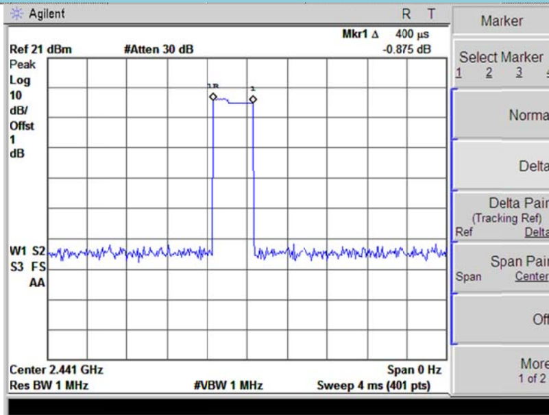
3-DH1
