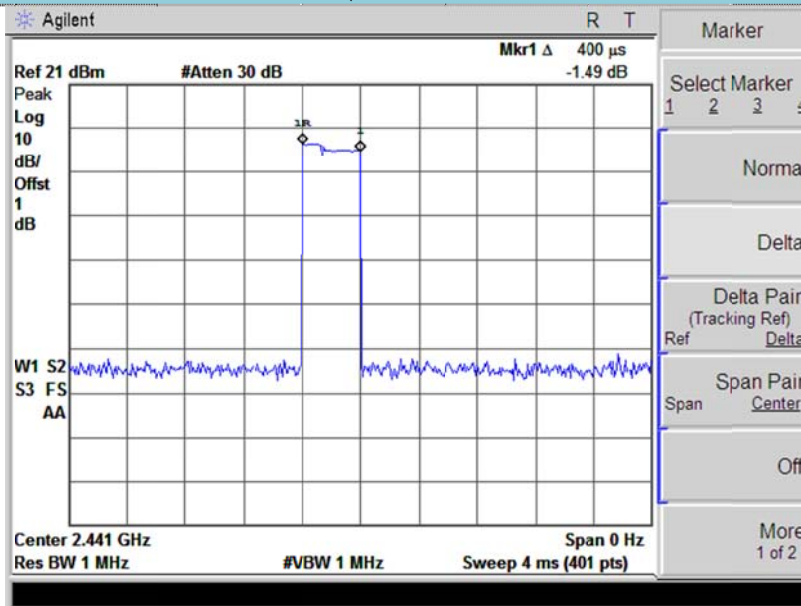
2-DH1
