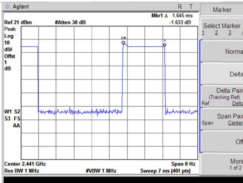
2-DH3
