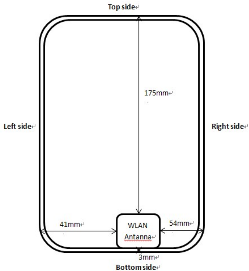
Figure 2: The antenna positions of the DUT
