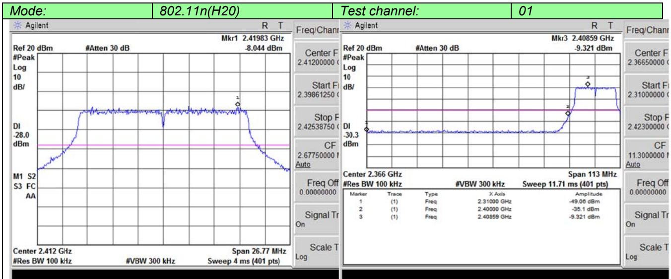
100kHz PSD Reference Level
