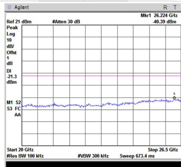
20GHz~26.5GHz
