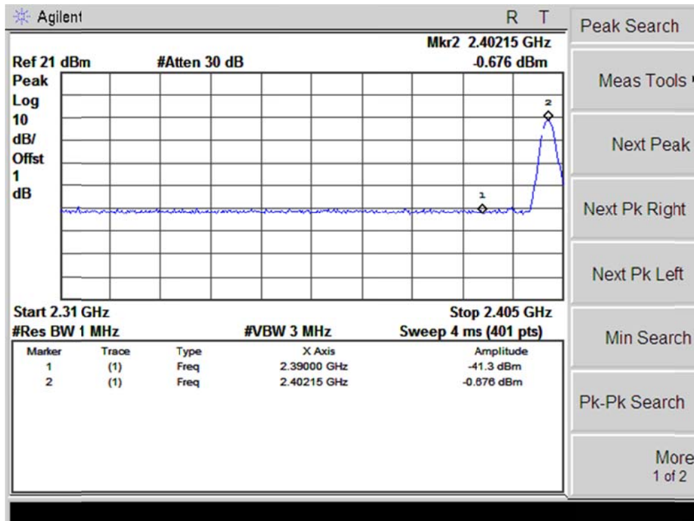
(Plot 4.5.3 A1:Channel 1: 2402MHz)
