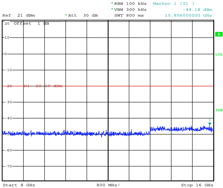
(Plot 4.9.1.C2: Channel 78: 2480MHz @ GFSK)
