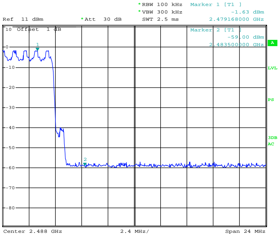
(Plot 4.5.2.2 C: Channel 78: 2480MHz @ 8DPSK)
