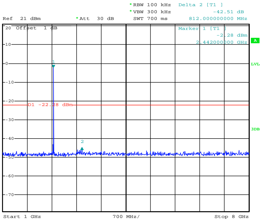
(Plot 4.9.3.B1: Channel 39: 2441MHz @ \pi/4 DQPSK)
