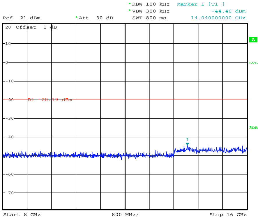
(Plot 4.9.1.A2: Channel 00: 2402MHz @ GFSK)
