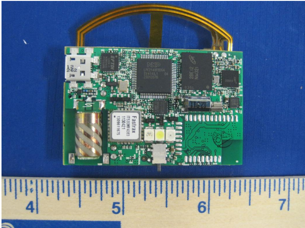
Main Board-Top
