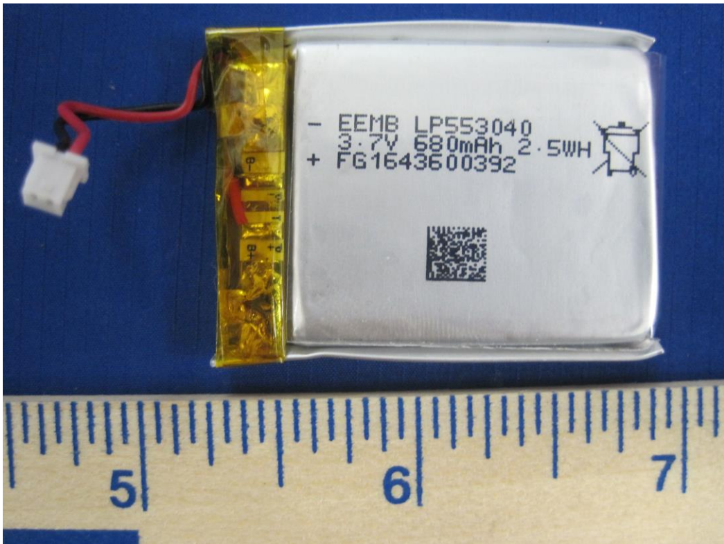
Battery
