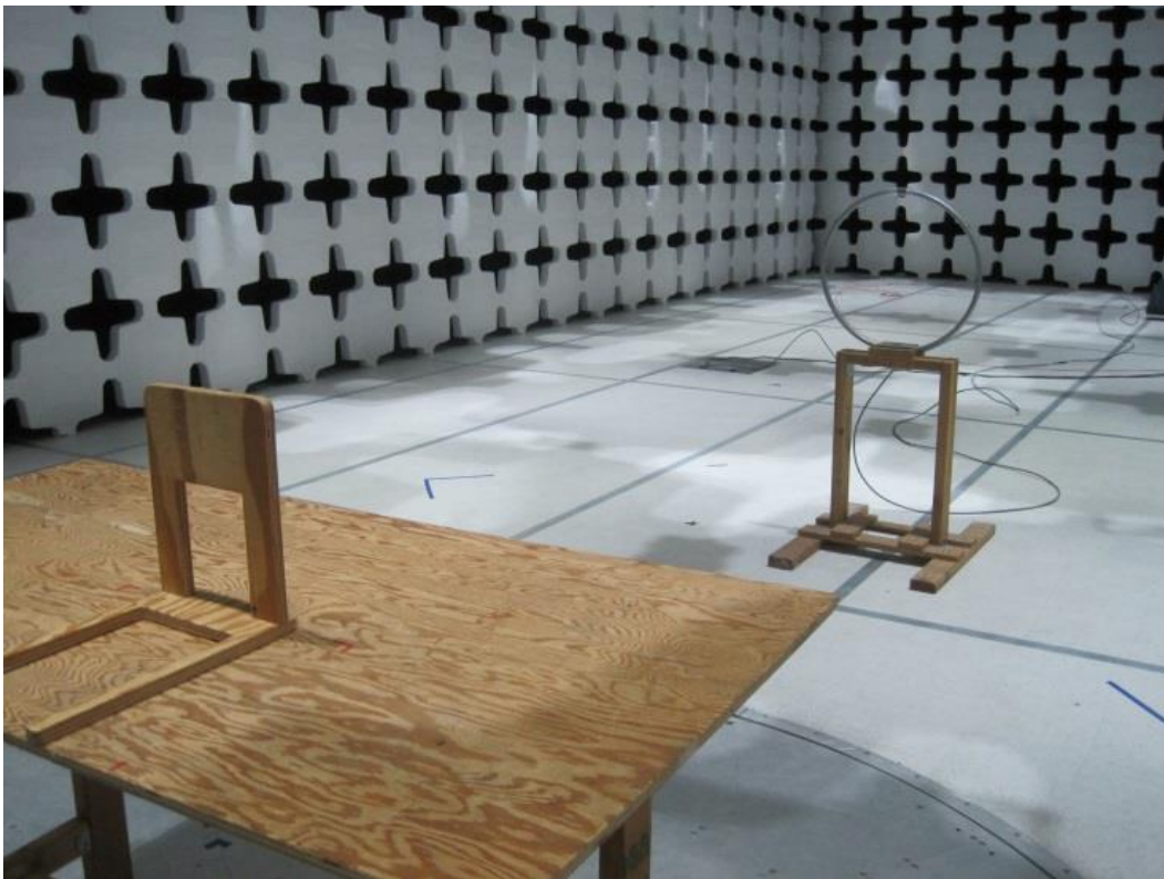
Radiated Emission Test setup (<30MHz) - Rear
