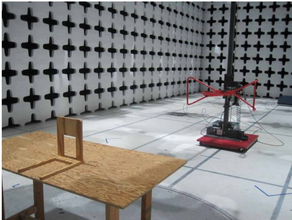
Radiated Emission Test setup (<1GHz) - Front
