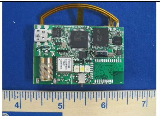
Main Board-Top
