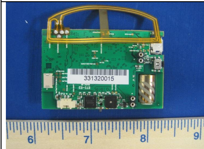
Main Board-Bottom
