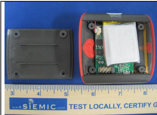
Cover Open
