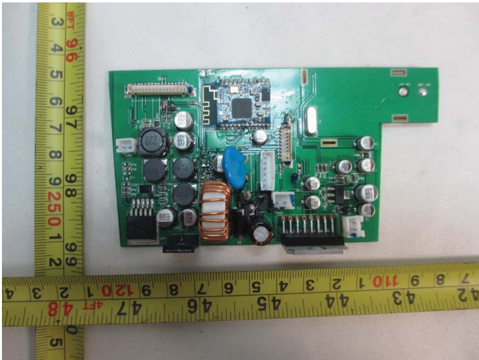
Power Board and Bluetooth Module Front
