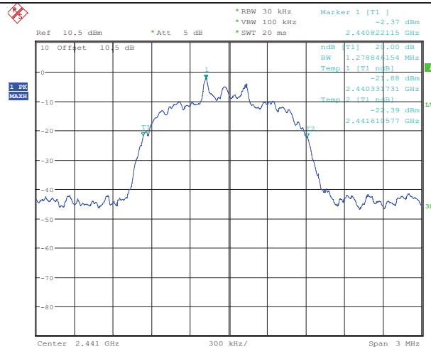
8-DPSK Tx Mode CH39
