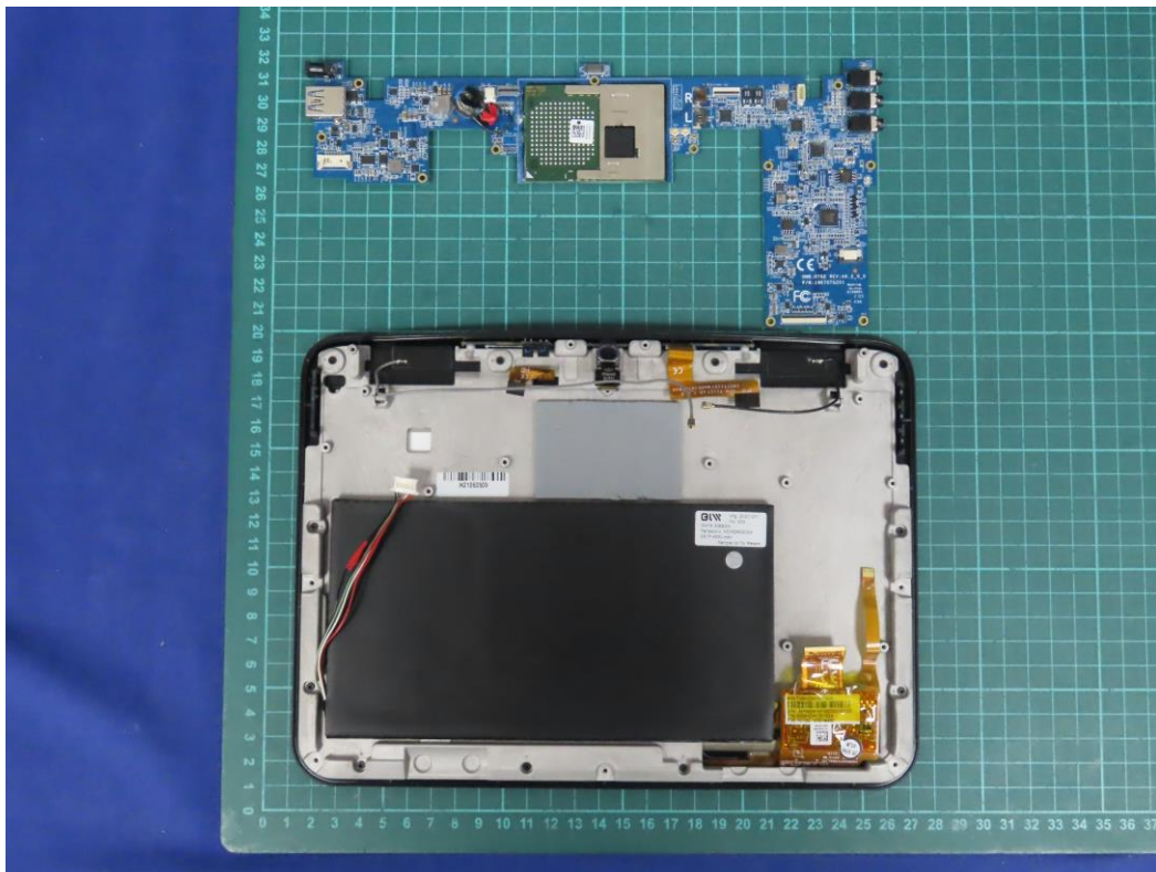
(11) EUT Photo
