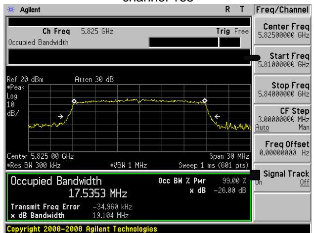
(802.11n20) -26dB&99% Bandwidth plot on channel 165
