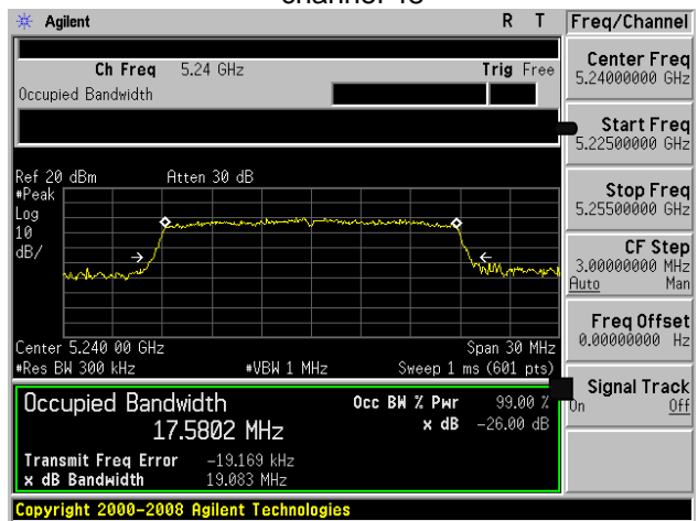
(802.11n20) -26dB&99% Bandwidth plot on channel 48
