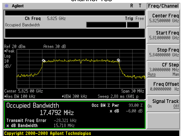
(802.11n20) -6dB Bandwidth plot on channel 165
