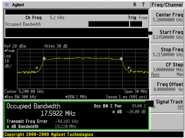
(802.11n20) -26dB&99% Bandwidth plot on channel 40
