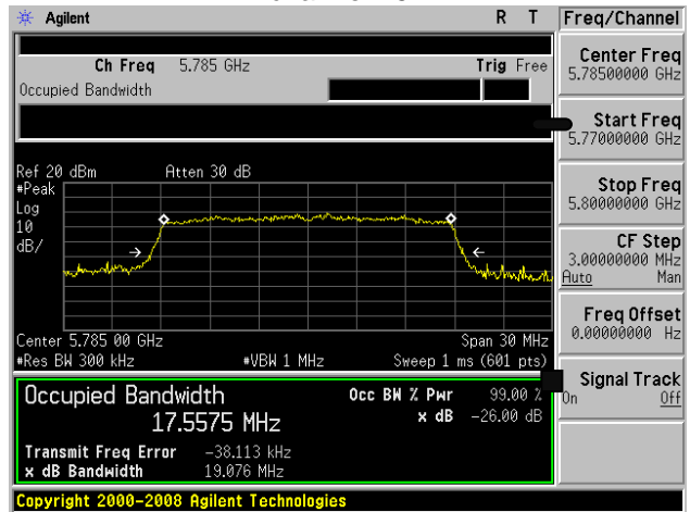
(802.11n20) -26dB&99% Bandwidth plot on channel 157
