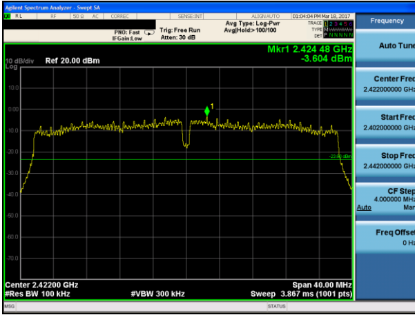
802.11 n40 on channel 3
