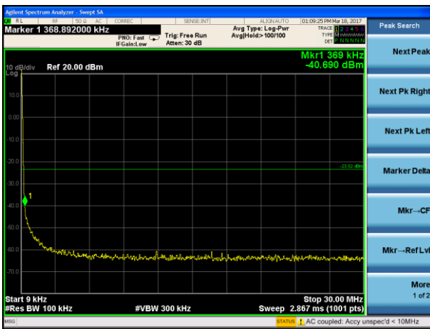
802.11 n40 on channel 6
