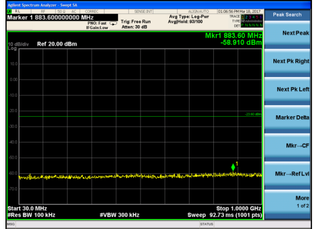
802.11 n40 on channel 3
