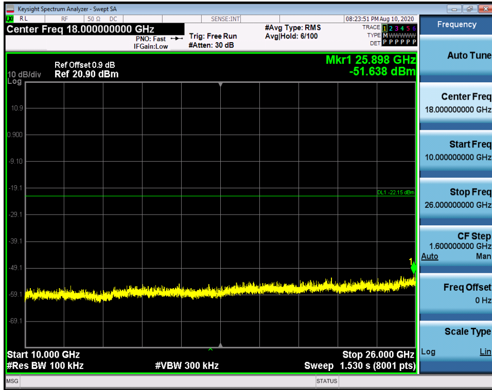
RF Conducted Spurious Emissions_11N40SISO_2422_Ant1
