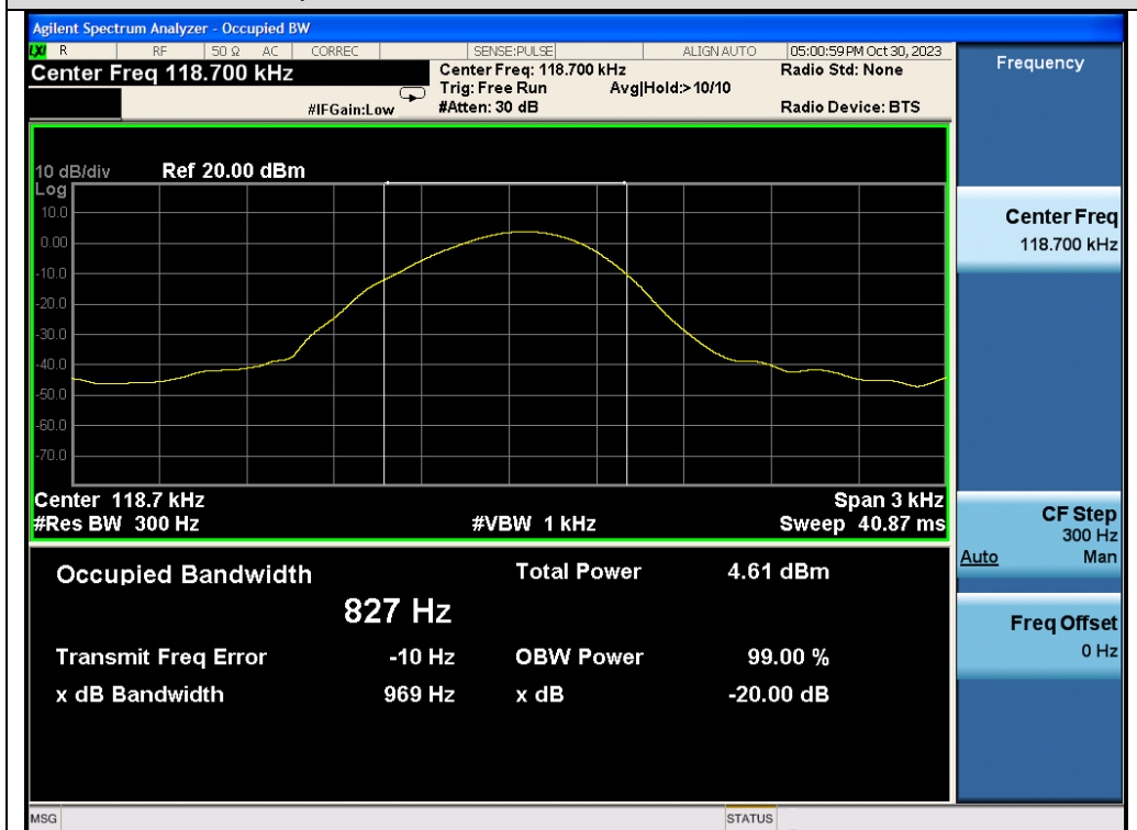
Test_Graph_ASK_Coil ANT_ 118.7kHz _ -20dB Bandwidth
