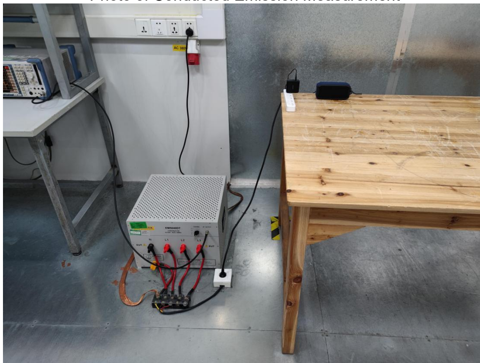
FCC ID: 2AANZRSEA1 Photo of Conducted Emission Measurement
