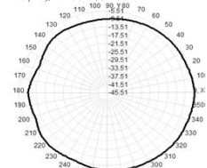
Total(H-XY), Max: -6.03dBi, C/D: 6.88
