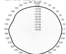
Total(H-XY), Max: -5.51dBi, C/D: 6.82
