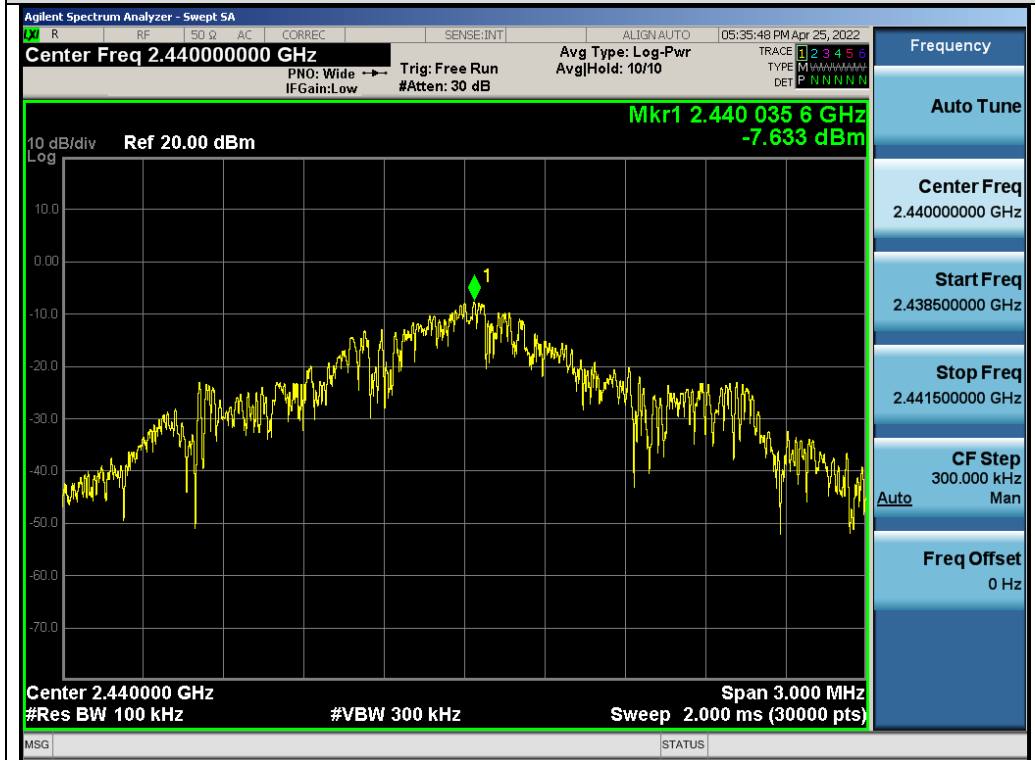
Test_Graph_2.4GHz_ANT1_2440_GFSK_Reference Level
