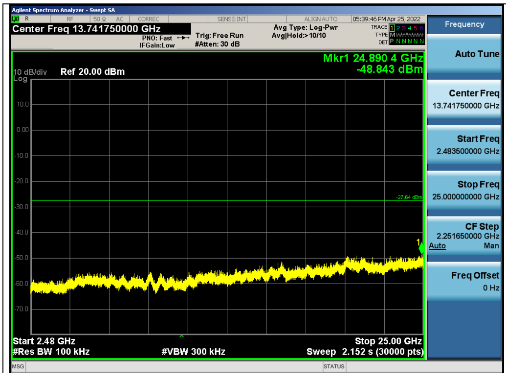
Test_Graph_2.4GHz_ANT1_2402_GFSK_Higher Band Emissions
