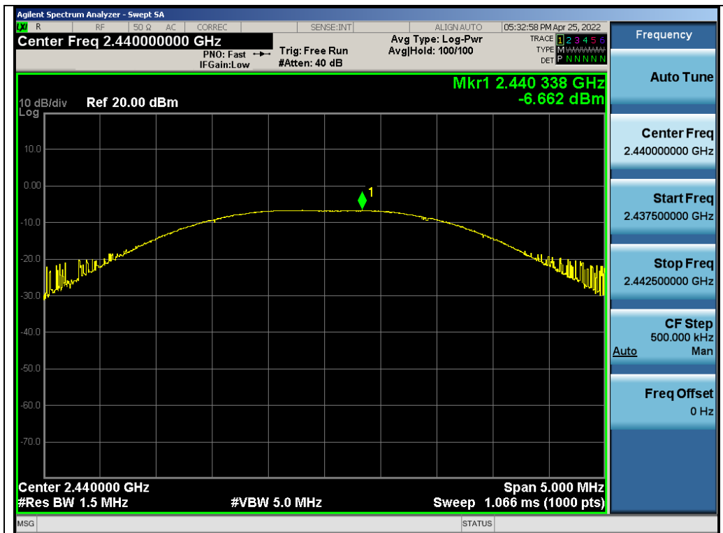
Test_Graph_2.4GHz_ANT1_2440_GFSK_Peak Power
