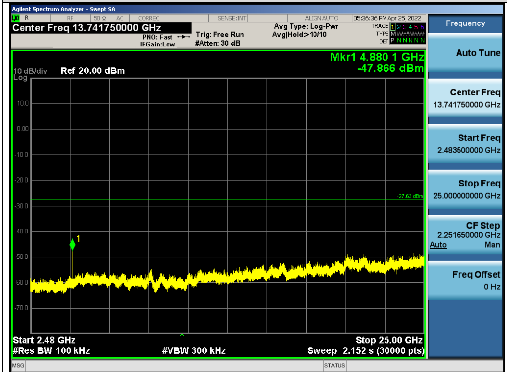
Test_Graph_2.4GHz_ANT1_2440_GFSK_Higher Band Emissions
