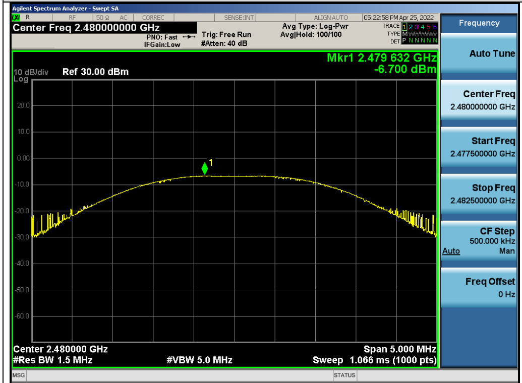
Test_Graph_2.4GHz_ANT1_2480_GFSK_Peak Power
