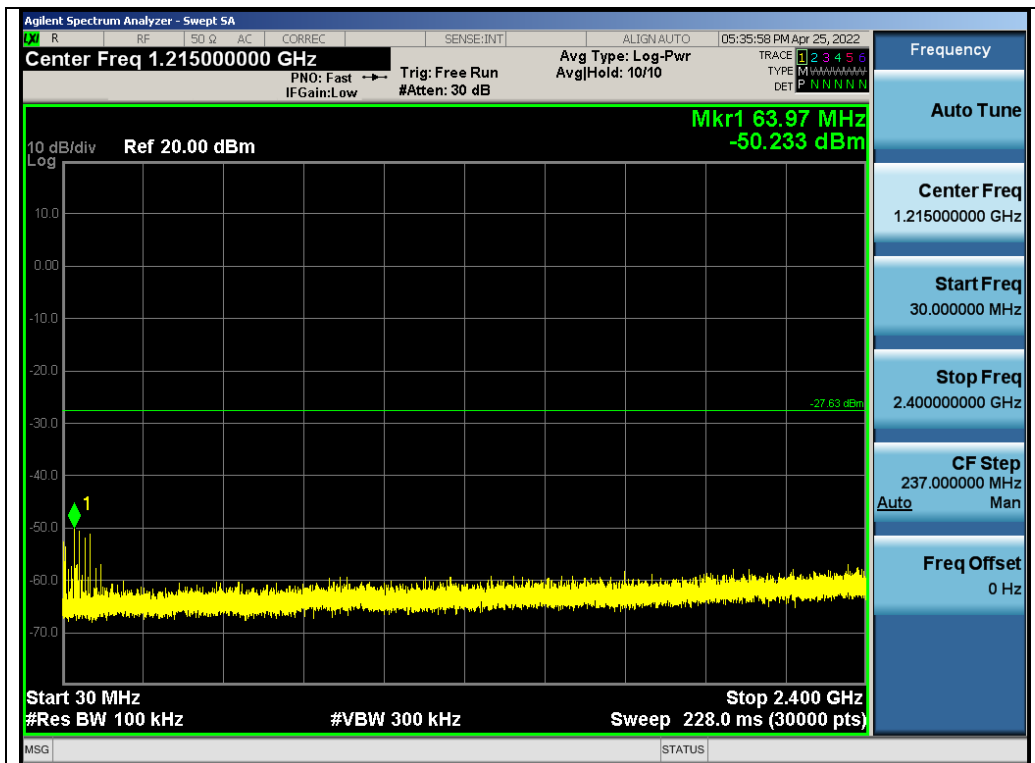
Test_Graph_2.4GHz_ANT1_2440_GFSK_Lower Band Emissions
