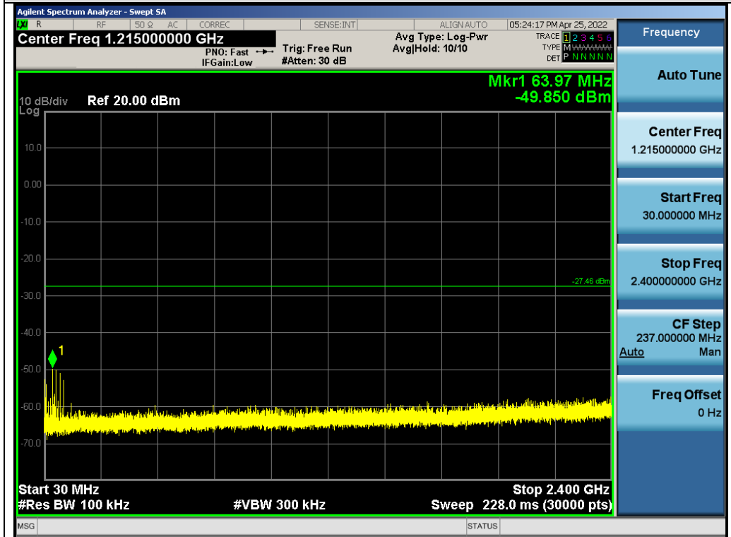
Test_Graph_2.4GHz_ANT1_2480_GFSK_Lower Band Emissions
