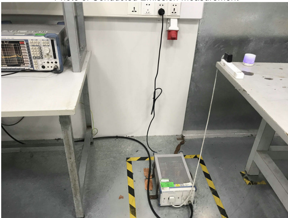
FCC ID: 2AANZLEDXC Photo of Conducted Emission Measurement
