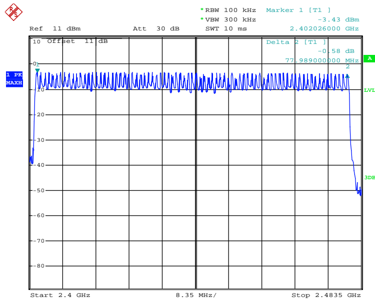
Number of hopping channels( \pi/4 -DQPSK)
