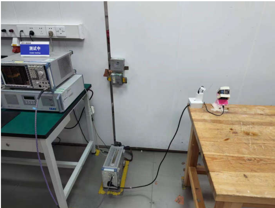
Conducted Emissions-2
