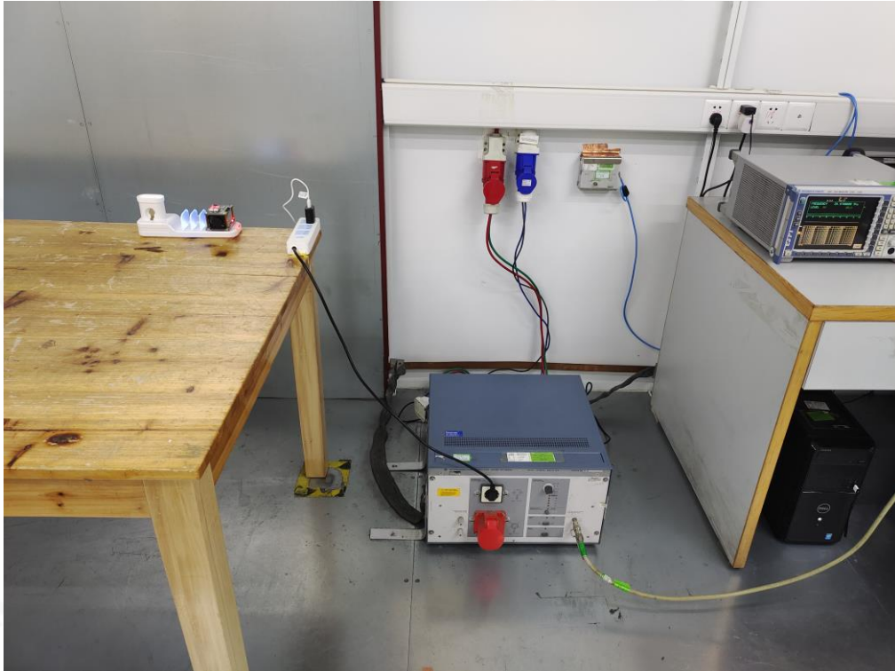
RF HEALTH ASSESSMENT TEST PHOTOS Position E
