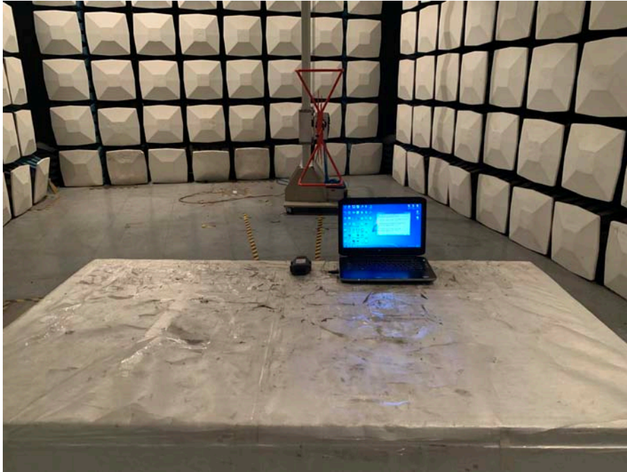
Radiated Disturbance Test Setup Front View (Below 1GHz)
