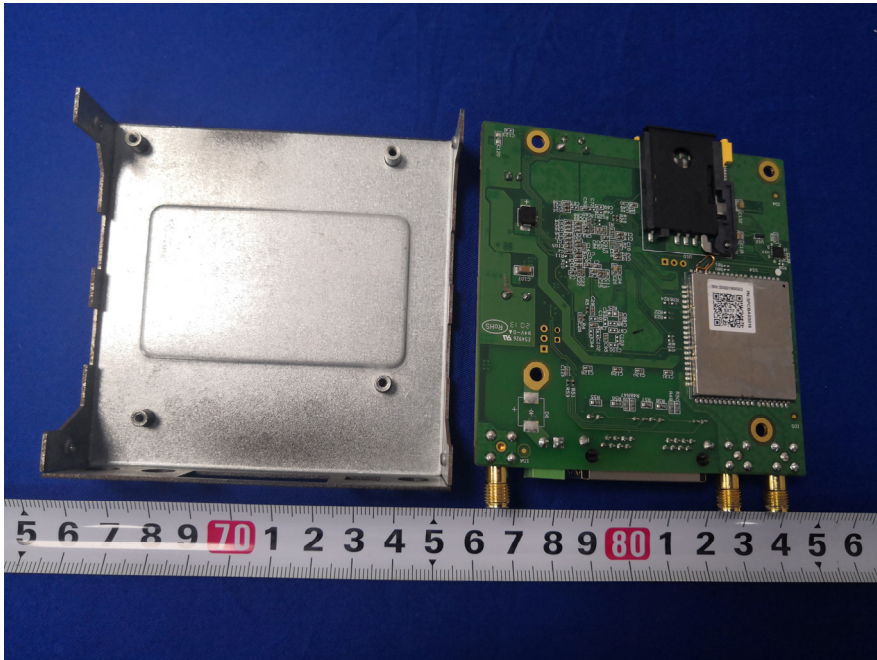
Uncovered 2 View
