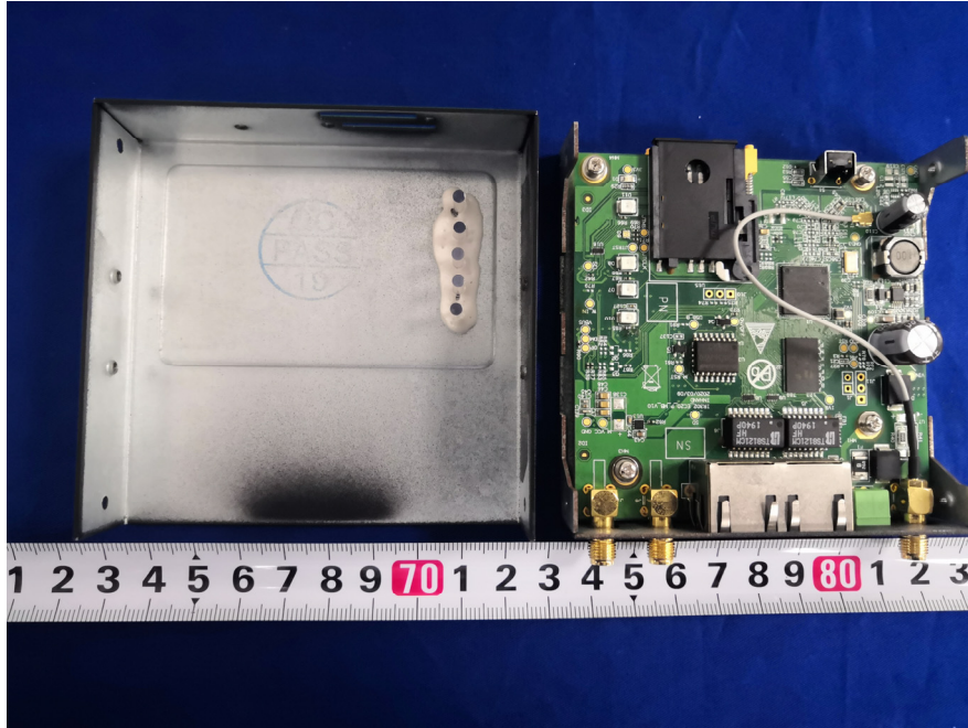
Uncovered 1 View
