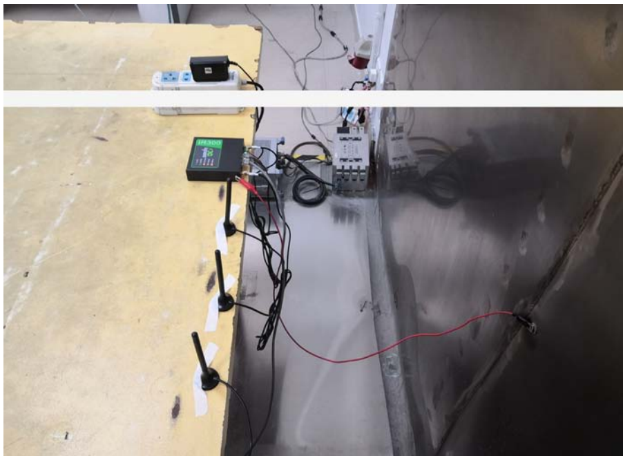
Conducted Emissions Test Setup Side View
