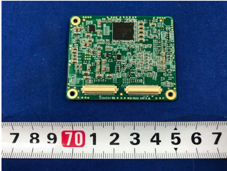
Sub Board 3 Bottom View
