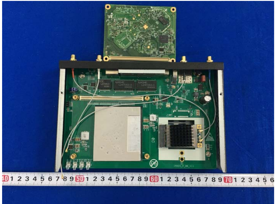
Uncovered View 3
