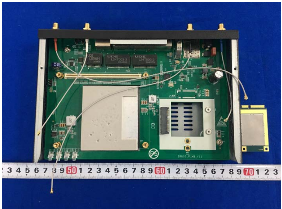
Uncovered View 4
