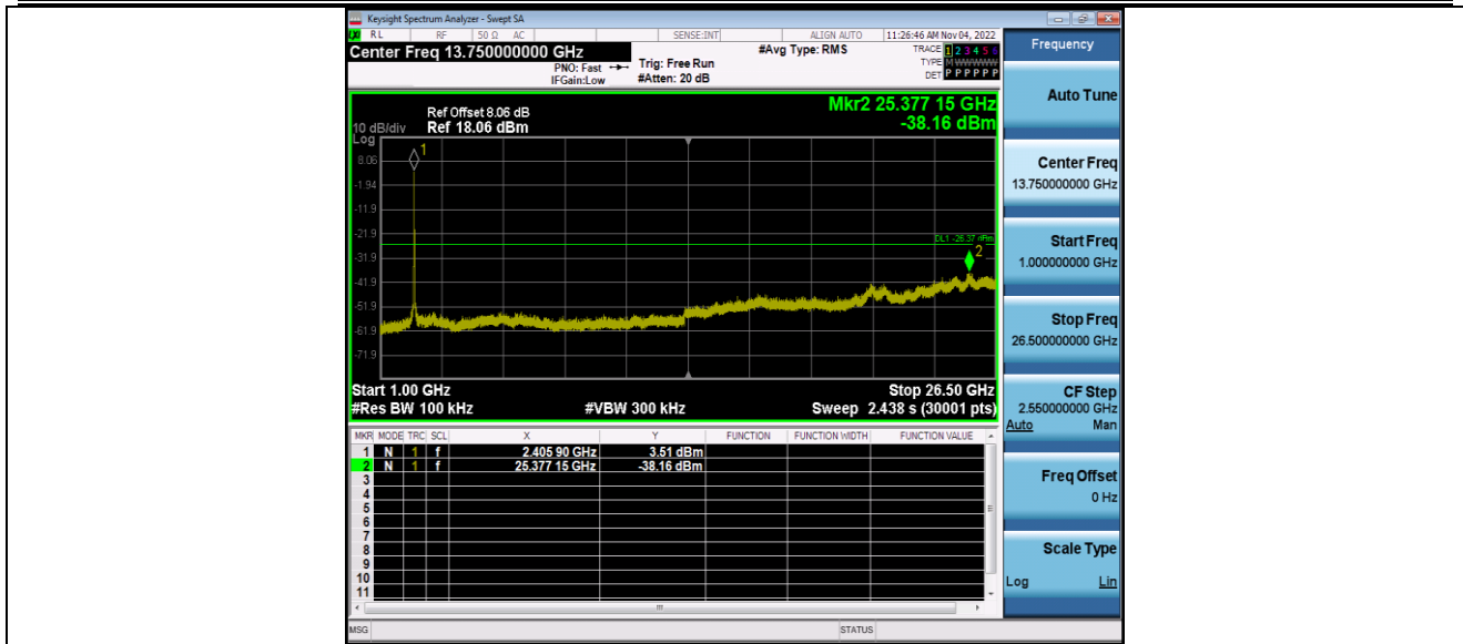
11G-CDD_Ant2_2412_0~Reference
