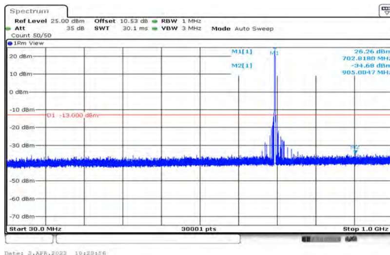
Band85-10MHz-16QAM-134092-1-0-Low-30-1000--34.68-PASS
