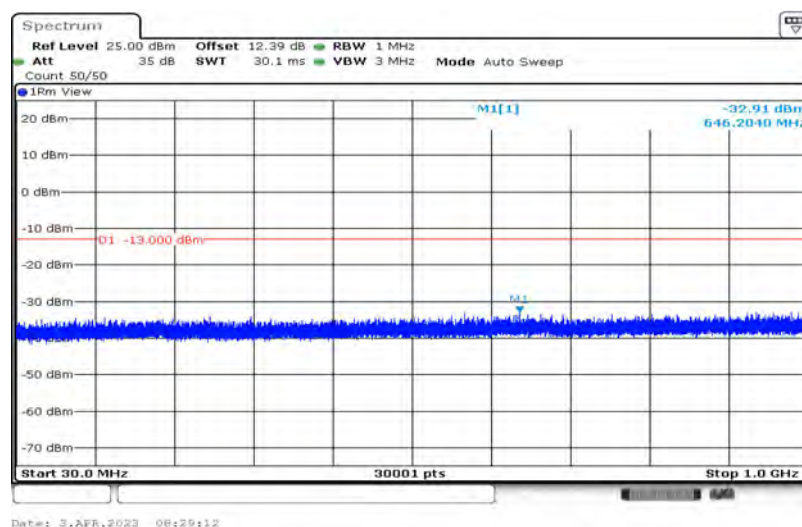
Band66-5MHz-16QAM-132322-1-0-Low-30-1000--32.91-PASS
