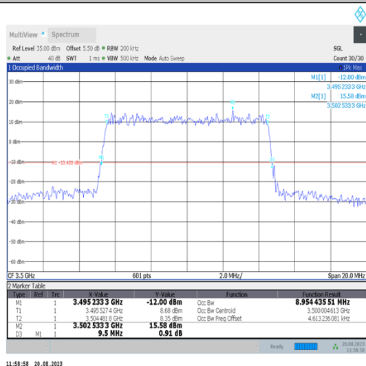
Band42-10MHz-16QAM-42590-50RB#0-PASS
