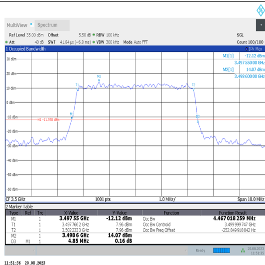
Band42-5MHz-16QAM-42590-25RB#0-PASS
