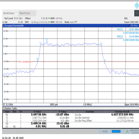
Band42-5MHz-QPSK-42590-25RB#0-PASS
