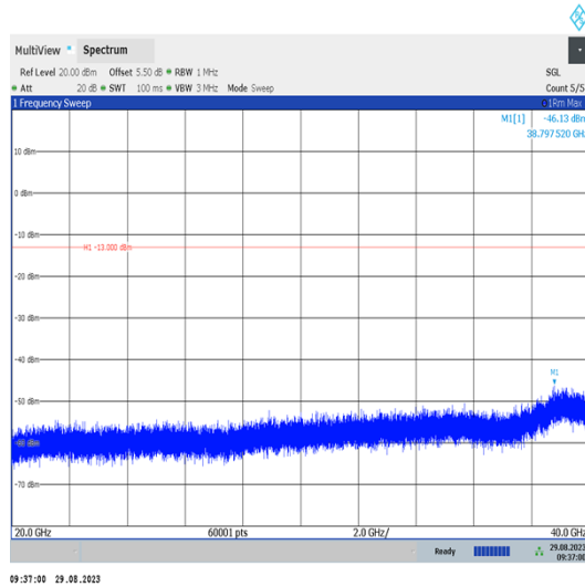
Band42_20MHz_QPSK_42990_1RB#0_20000~40000_20000~40000
