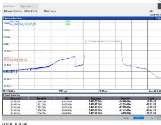
Band41-5MHz-QPSK-39675-25RB#0
