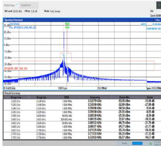
Band43_5MHz_QPSK_43615_1RB#0
