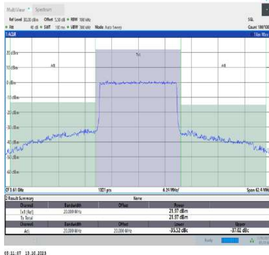
43(3600-3700)-20MHz-QPSK-43690-100RB#0-PASS
