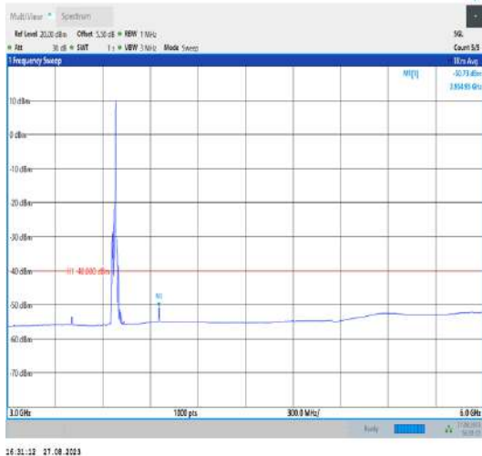
Band43_20MHz_QPSK_44490_1RB#0_3000~6000_30 00~6000
