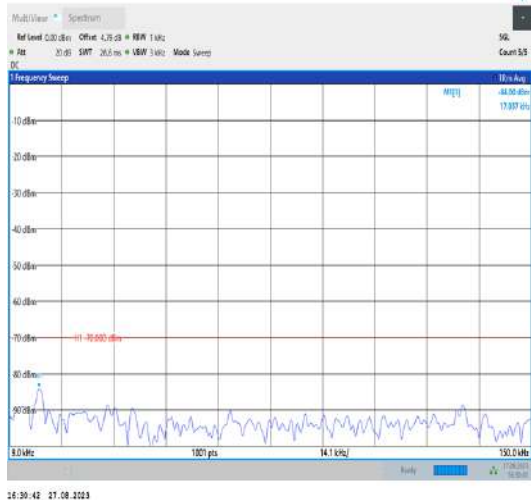
Band43_20MHz_QPSK_44490_1RB#0_0.009~0.15_0.09~0.15
