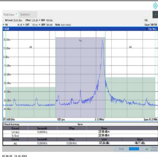
43(3600-3700)-10MHz-QPSK-43640-1RB#49-PASS
