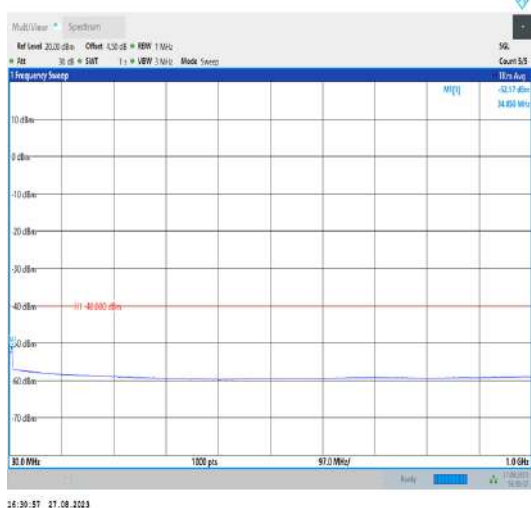
Band43_20MHz_QPSK_44490_1RB#0_30~1000_30~10
