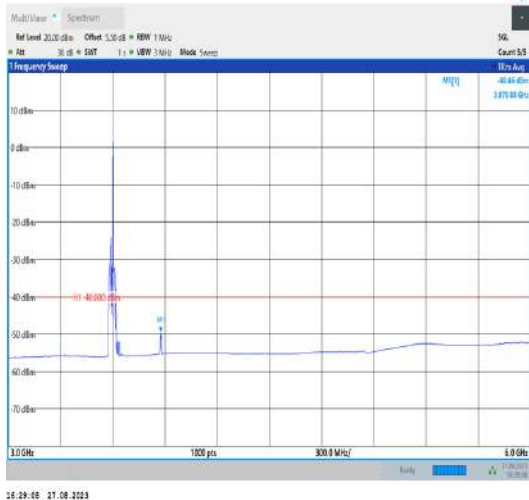
Band43_20MHz_QPSK_43690_1RB#0_3000~6000_3000~6000
