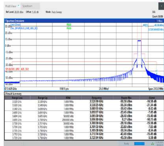
Band43_5MHz_QPSK_44565_25RB#0
