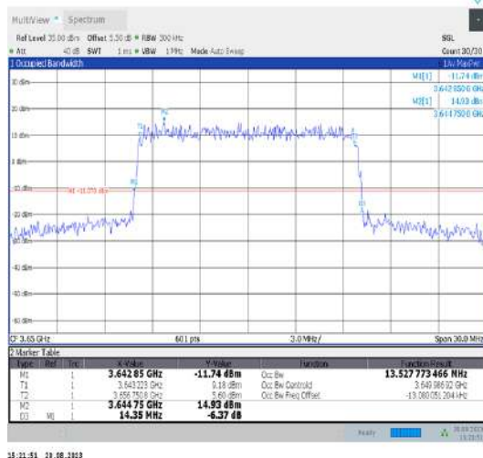
Band43-15MHz-QPSK-44090-75RB#0-PASS
