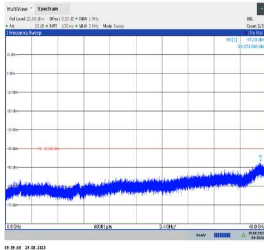
Band43_20MHz_QPSK_43690_1RB#0_6000~40000_6000~40000
