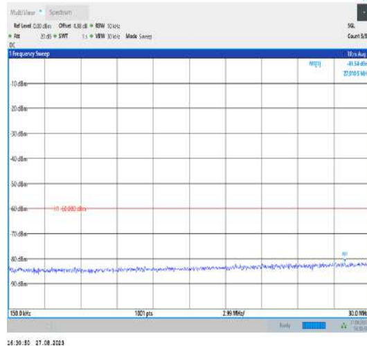
Band43_20MHz_QPSK_44490_1RB#0_0.15~30_0.15~30
