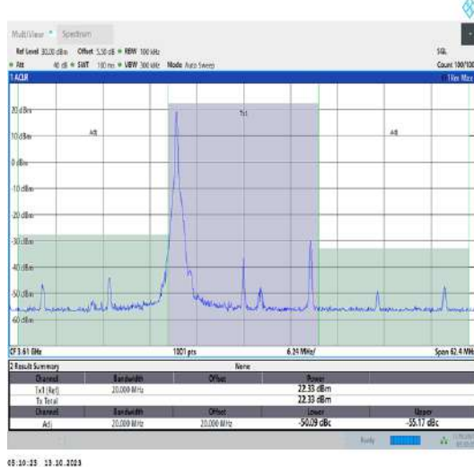
43(3600-3700)-20MHz-QPSK-43690-1RB#0-PASS
