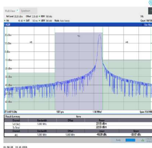
43(3600-3700)-5MHz-QPSK-44565-1RB#24-PASS
