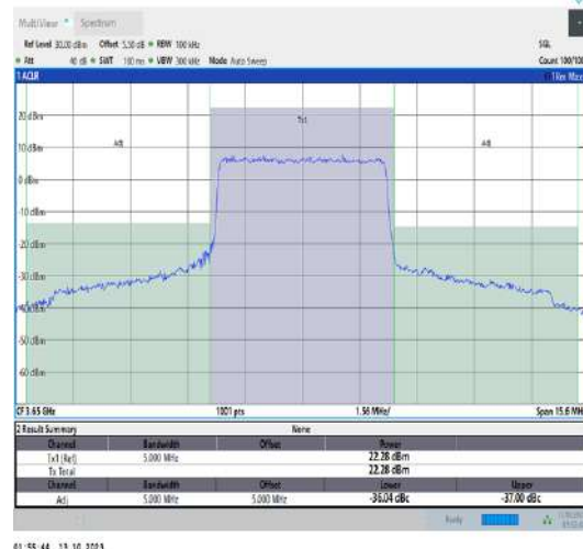
43(3600-3700)-5MHz-QPSK-44090-25RB#0-PASS
