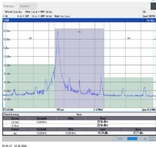
43(3600-3700)-10MHz-QPSK-44090-1RB#0-PASS
