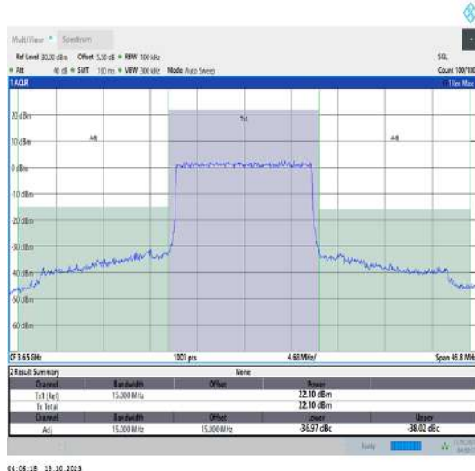
43(3600-3700)-15MHz-QPSK-44090-75RB#0-PASS
