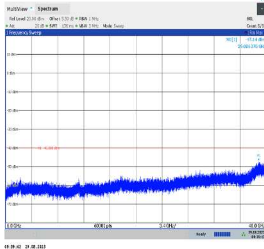
Band43_20MHz_QPSK_44490_1RB#0_6000~40000_600 0~40000
