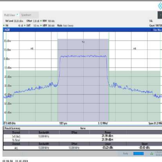
43(3600-3700)-10MHz-QPSK-43640-50RB#0-PASS
