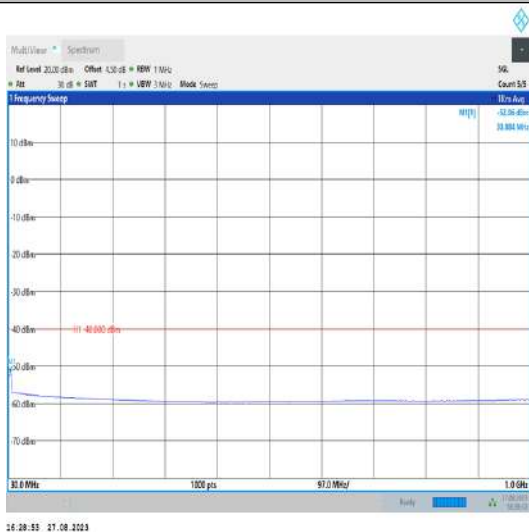
Band43_20MHz_QPSK_43690_1RB#0_30~1000_30~1 000
