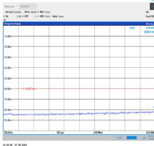
Band43_20MHz_QPSK_44090_1RB#0_0.15~30_0.15~30
