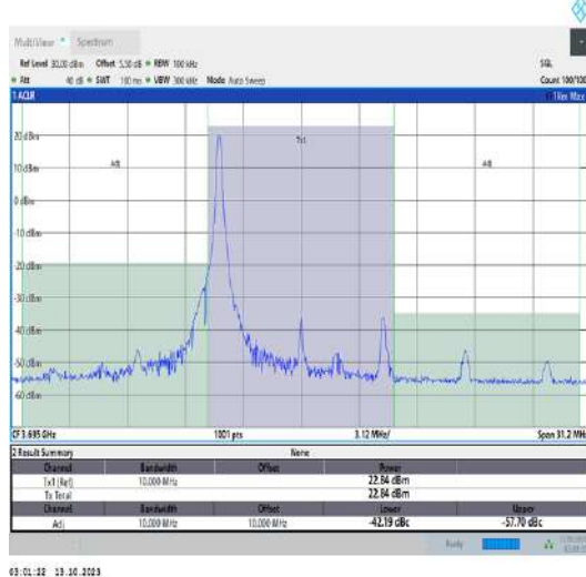
43(3600-3700)-10MHz-QPSK-44540-1RB#0-PASS
