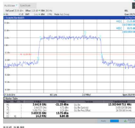
Band43-15MHz-16QAM-44090-75RB#0-PASS
