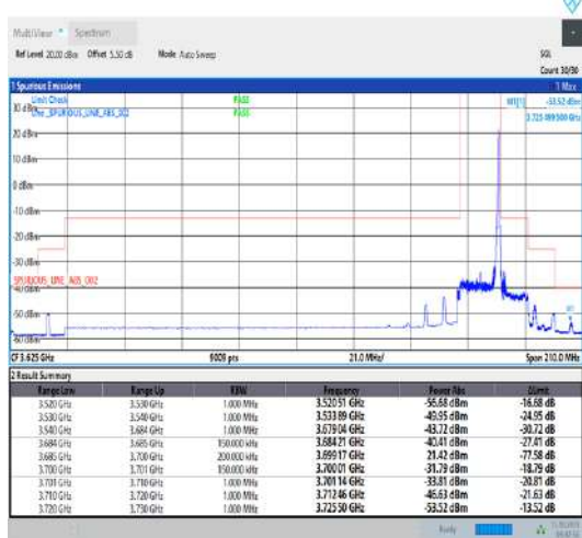
Band43_15MHz_QPSK_44515_1RB#74
