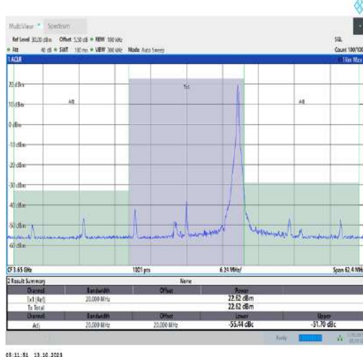
43(3600-3700)-20MHz-QPSK-44090-1RB#99-PASS
