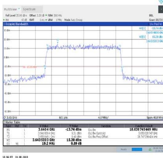
Band43-20MHz-QPSK-44090-100RB#0-PASS
