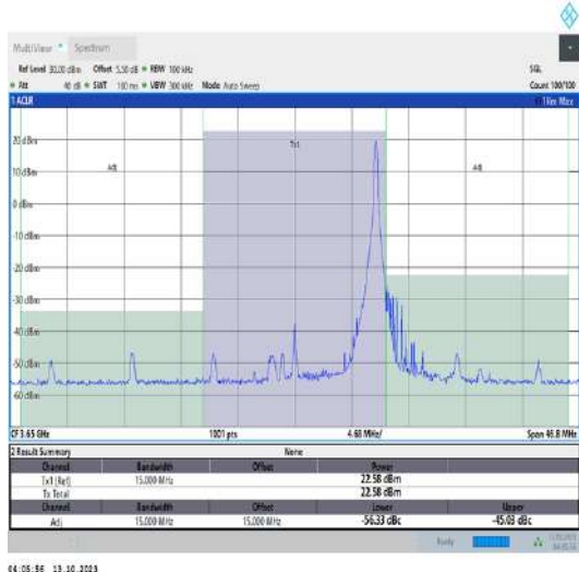
43(3600-3700)-15MHz-QPSK-44090-1RB#74-PASS
