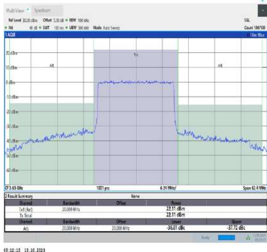
43(3600-3700)-20MHz-QPSK-44090-100RB#0-PASS
