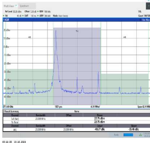
43(3600-3700)-20MHz-QPSK-44490-1RB#0-PASS
