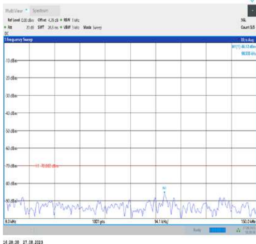
Band43_20MHz_QPSK_43690_1RB#0_0.009~0.15_0.0 09~0.15
