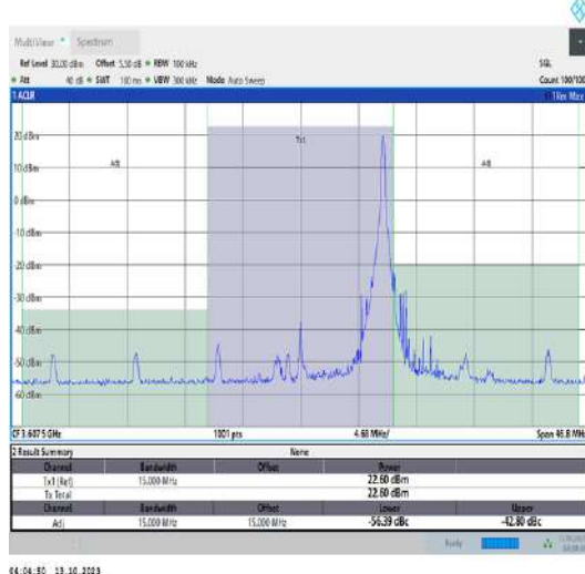
43(3600-3700)-15MHz-QPSK-43665-1RB#74-PASS
