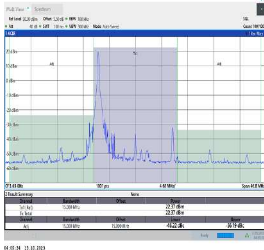
43(3600-3700)-15MHz-QPSK-44090-1RB#0-PASS
