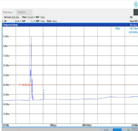
Band43_20MHz_QPSK_44090_1RB#0_3000~6000_30~6000
