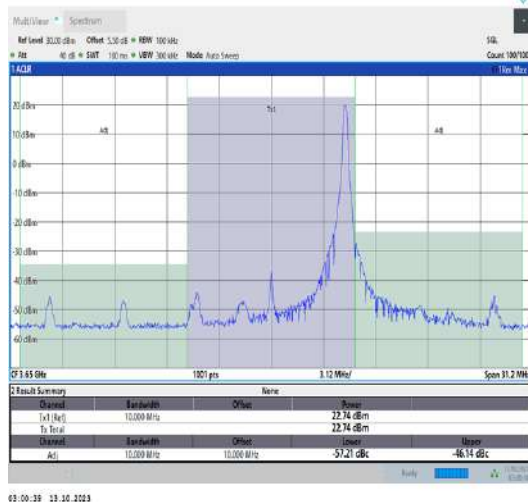
43(3600-3700)-10MHz-QPSK-44090-1RB#49-PASS
