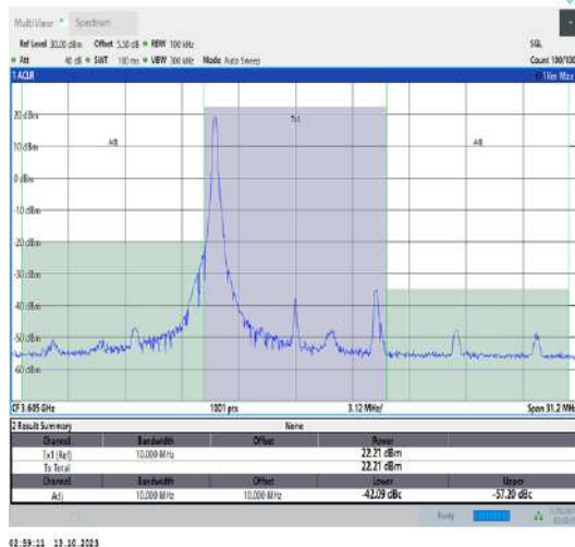
43(3600-3700)-10MHz-QPSK-43640-1RB#0-PASS
