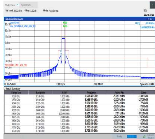
Band43_5MHz_QPSK_43615_25RB#0
