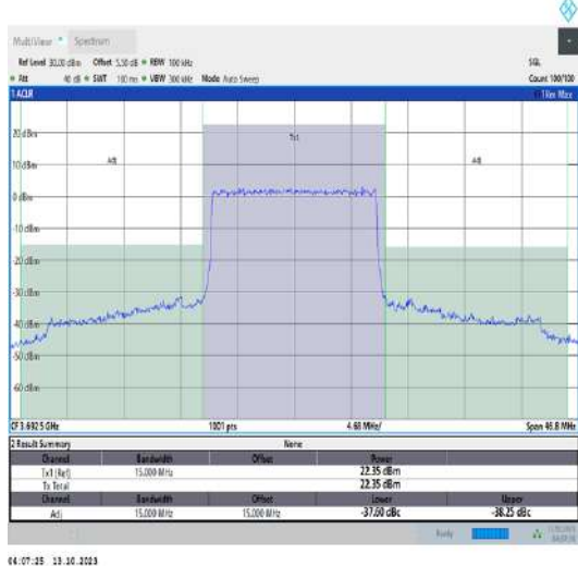
43(3600-3700)-15MHz-QPSK-44515-75RB#0-PASS
