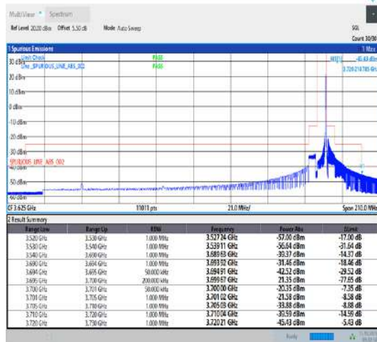
Band43_5MHz_QPSK_44565_1RB#24
