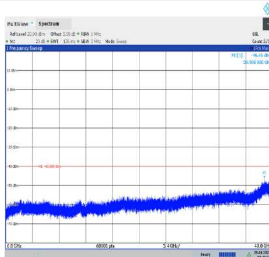
Band43_20MHz_QPSK_44090_1RB#0_6000~40000_6000~40000
