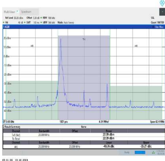
43(3600-3700)-20MHz-QPSK-44090-1RB#0-PASS
