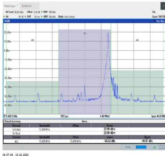
43(3600-3700)-15MHz-QPSK-44515-1RB#74-PASS
