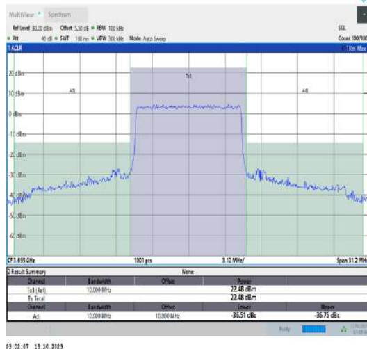
43(3600-3700)-10MHz-QPSK-44540-50RB#0-PASS
