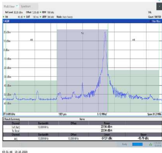
43(3600-3700)-10MHz-QPSK-44540-1RB#49-PASS
