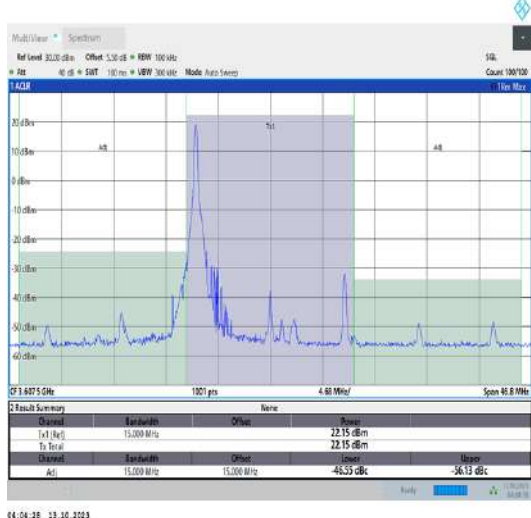
43(3600-3700)-15MHz-QPSK-43665-1RB#0-PASS
