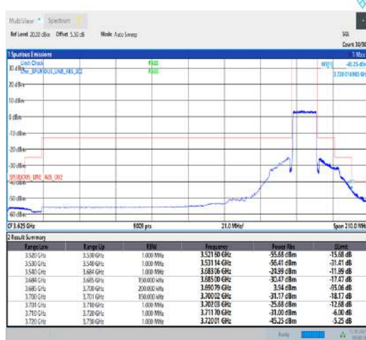
Band43_15MHz_QPSK_44515_75RB#0
