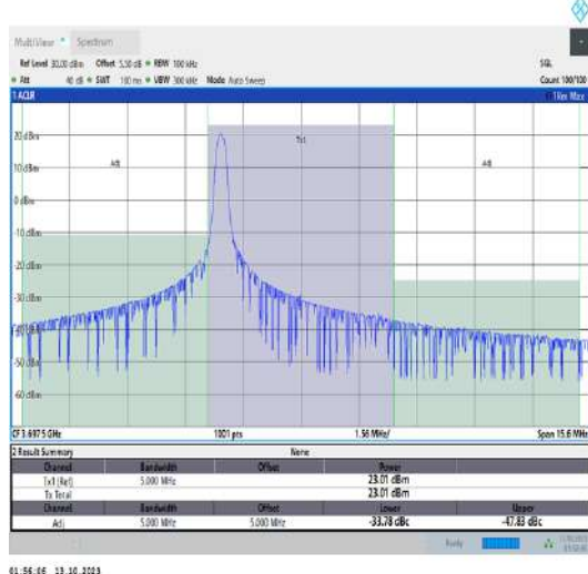
43(3600-3700)-5MHz-QPSK-44565-1RB#0-PASS
