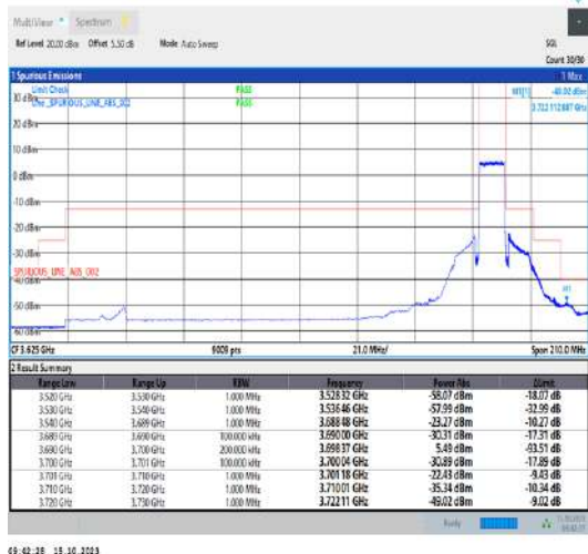
Band43_15MHz_QPSK_43665_1RB#0
