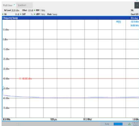
Band43_20MHz_QPSK_44090_1RB#0_30~1000_30~1000
