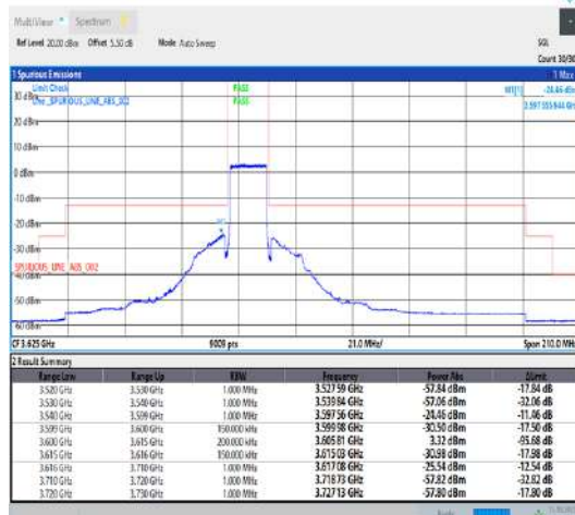
Band43_15MHz_QPSK_43665_75RB#0
