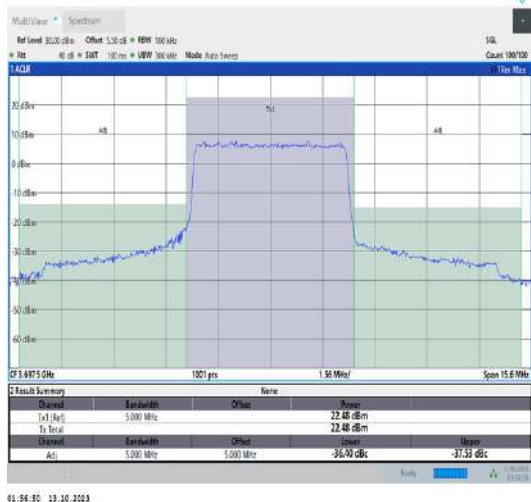
43(3600-3700)-5MHz-QPSK-44565-25RB#0-PASS
