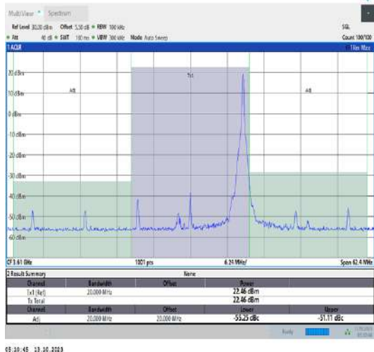
43(3600-3700)-20MHz-QPSK-43690-1RB#99-PASS
