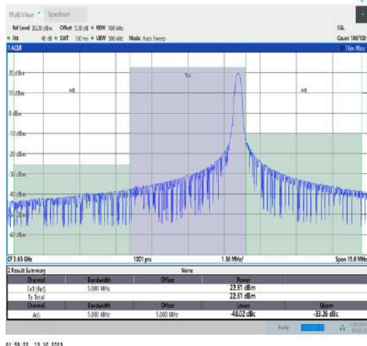
43(3600-3700)-5MHz-QPSK-44090-1RB#24-PASS
