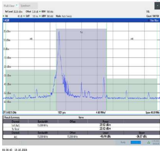
43(3600-3700)-15MHz-QPSK-44515-1RB#0-PASS
