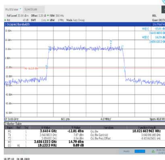
Band43-20MHz-16QAM-44090-100RB#0-PASS
