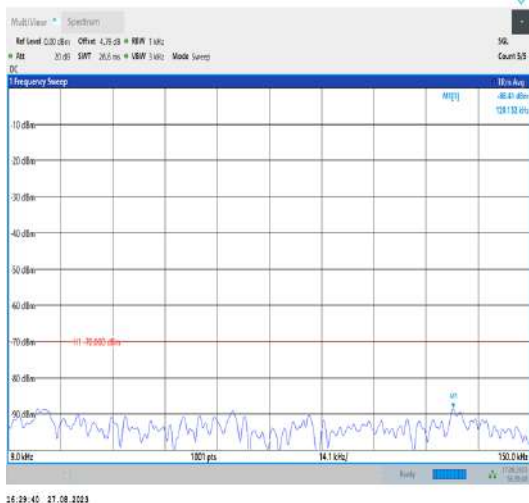
Band43_20MHz_QPSK_44090_1RB#0_0.009~0.15_0.009~0.15
