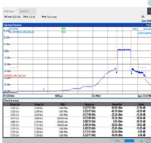
Band43_20MHz_QPSK_44490_100RB#0
