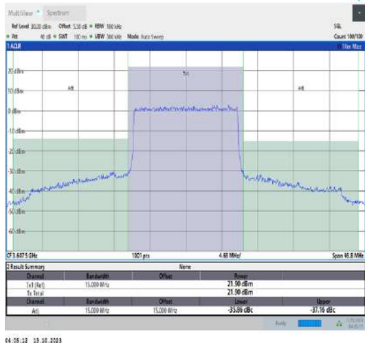
43(3600-3700)-15MHz-QPSK-43665-75RB#0-PASS
