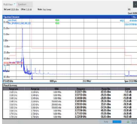
Band42_15MHz_QPSK_43165_1RB#0
