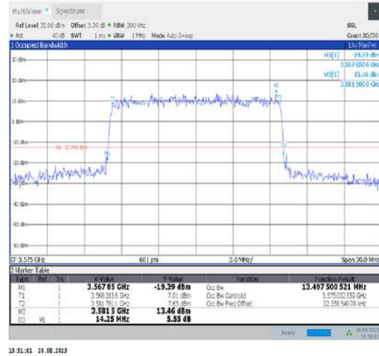
Band42-15MHz-16QAM-43340-75RB#0-PASS
