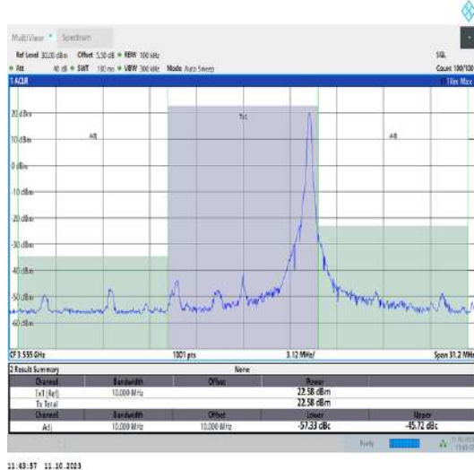
42(3550-3600)-10MHz-QPSK-43140-1RB#49-PASS
