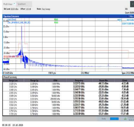
Band42_5MHz_QPSK_43115_1RB#0
