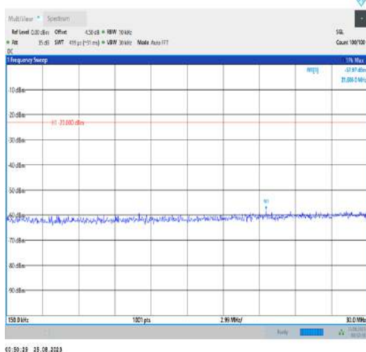
Band42_20MHz_QPSK_43340_1RB#0_0.15~30_0.15~30
