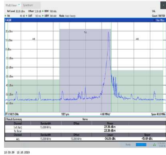
42(3550-3600)-15MHz-QPSK-43515-1RB#74-PASS
