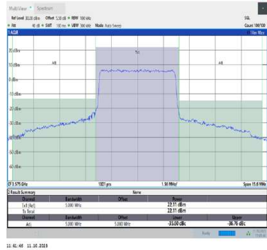
42(3550-3600)-5MHz-QPSK-43340-25RB#0-PASS
