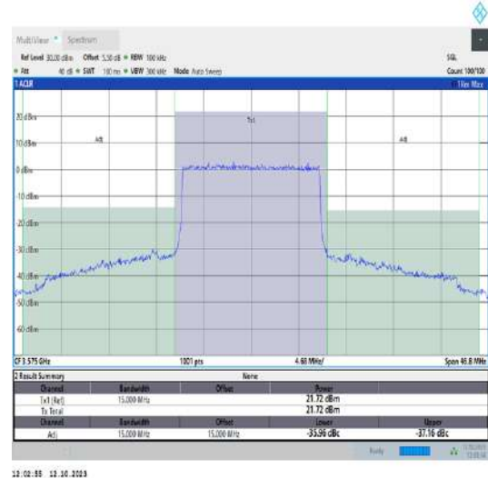
42(3550-3600)-15MHz-QPSK-43340-75RB#0-PASS
