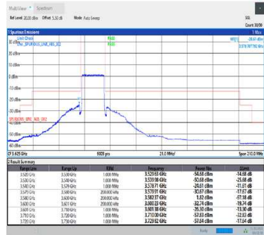
Band42_20MHz_QPSK_43490_100RB#0
