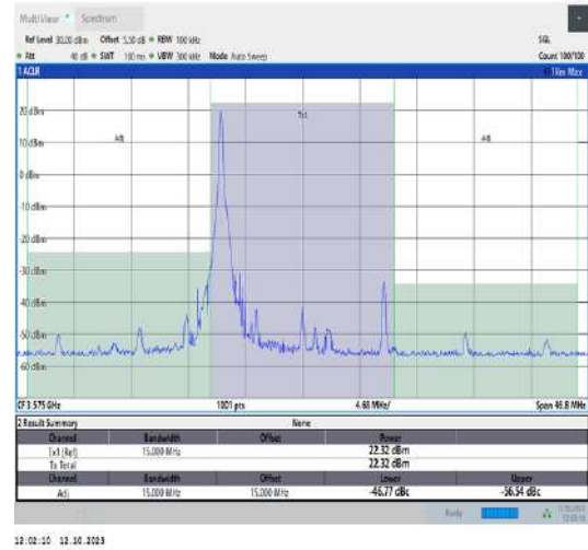
42(3550-3600)-15MHz-QPSK-43340-1RB#0-PASS
