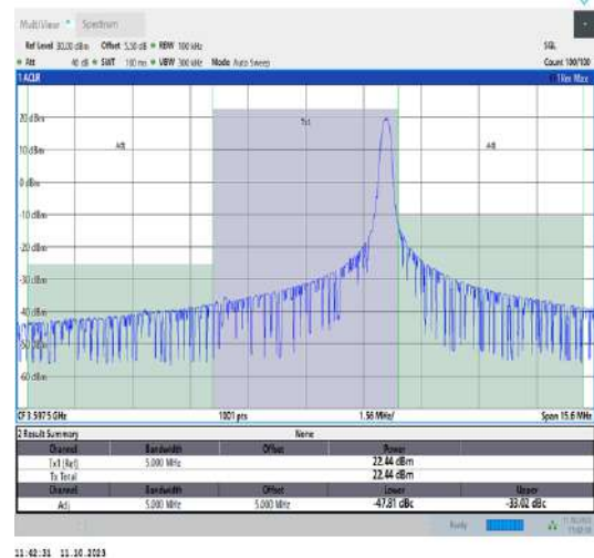
42(3550-3600)-5MHz-QPSK-43565-1RB#24-PASS
