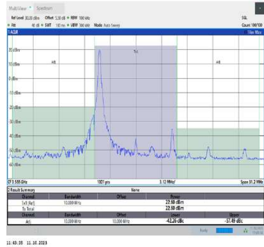
42(3550-3600)-10MHz-QPSK-43140-1RB#0-PASS
