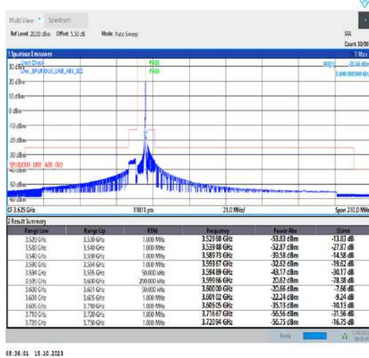
Band42_5MHz_QPSK_43565_1RB#24
