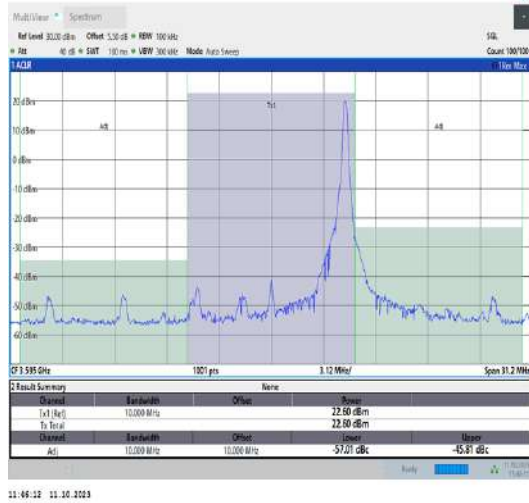
42(3550-3600)-10MHz-QPSK-43540-1RB#49-PASS
