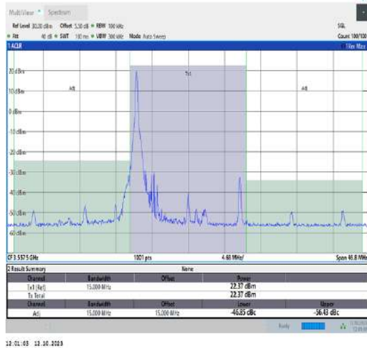
42(3550-3600)-15MHz-QPSK-43165-1RB#0-PASS
