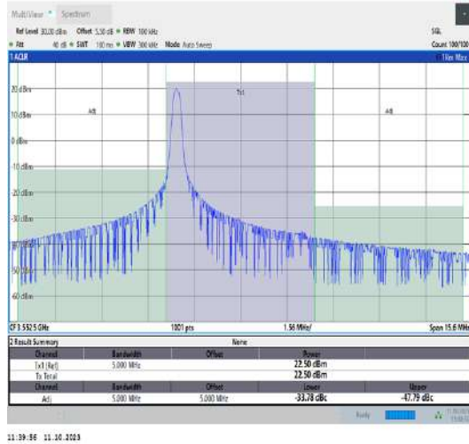
42(3550-3600)-5MHz-QPSK-43115-1RB#0-PASS
