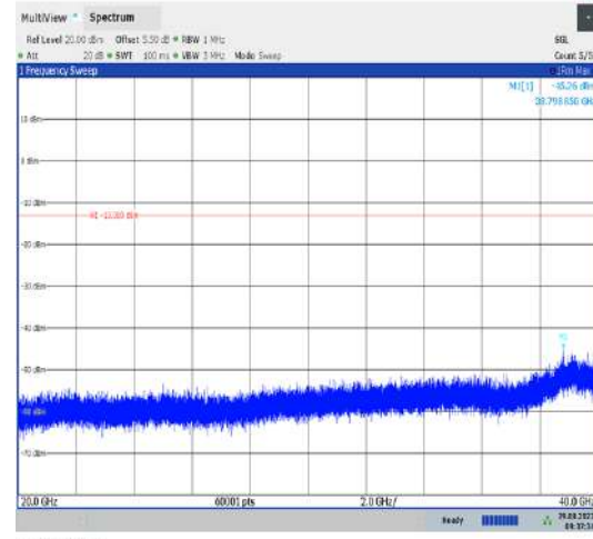
Band42_20MHz_QPSK_43340_1RB#0_20000~40000_20000~40000
