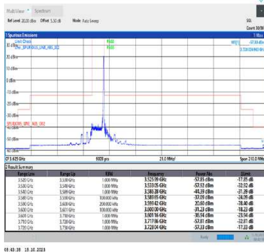
Band42_10MHz_QPSK_43540_1RB#49
