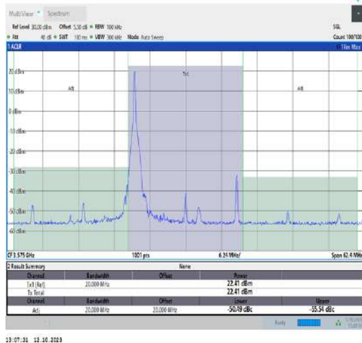
42(3550-3600)-20MHz-QPSK-43340-1RB#0-PASS
