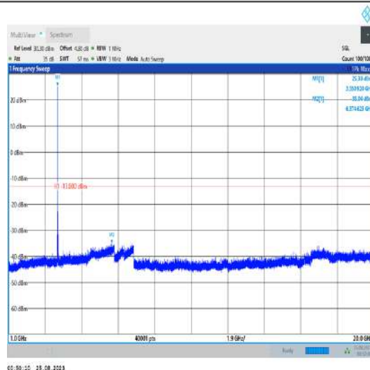
Band42_20MHz_QPSK_43190_1RB#0_1000~20000_1 000~20000
