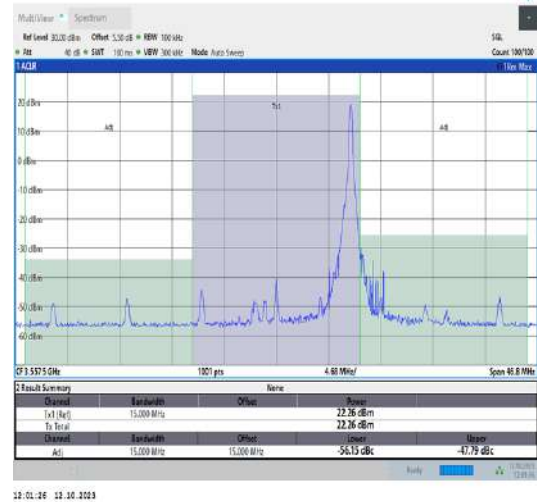
42(3550-3600)-15MHz-QPSK-43165-1RB#74-PASS
