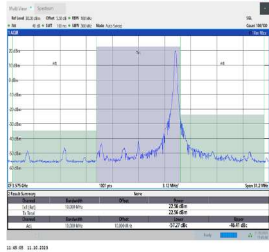
42(3550-3600)-10MHz-QPSK-43340-1RB#49-PASS
