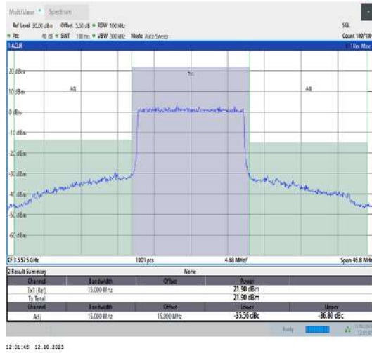
42(3550-3600)-15MHz-QPSK-43165-75RB#0-PASS
