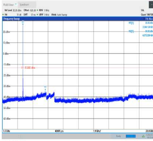
Band42_20MHz_QPSK_43340_1RB#0_1000~20000_1000~20000
