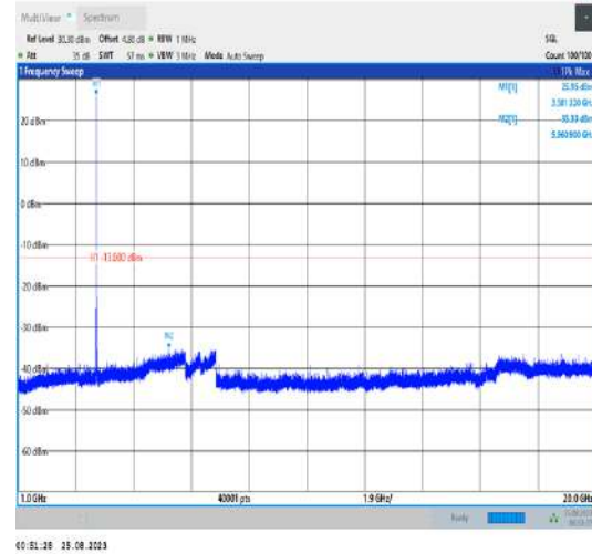
Band42_20MHz_QPSK_43490_1RB#0_1000~20000_1000~20000
