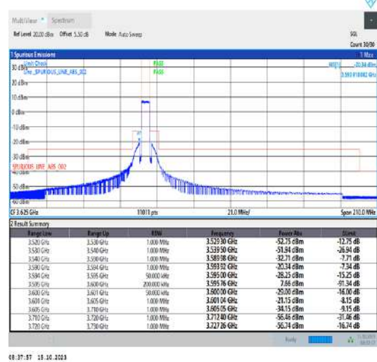
Band42_5MHz_QPSK_43565_25RB#0
