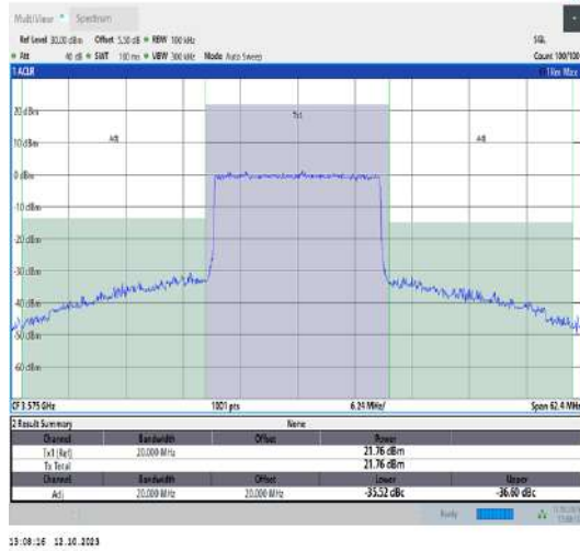
42(3550-3600)-20MHz-QPSK-43340-100RB#0-PASS
