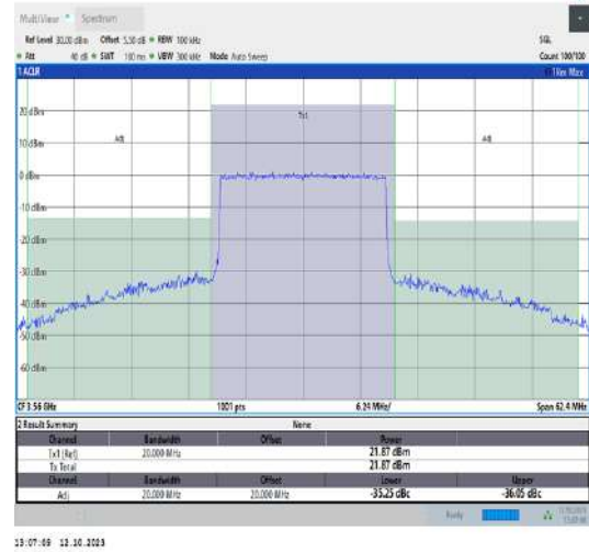
42(3550-3600)-20MHz-QPSK-43190-100RB#0-PASS
