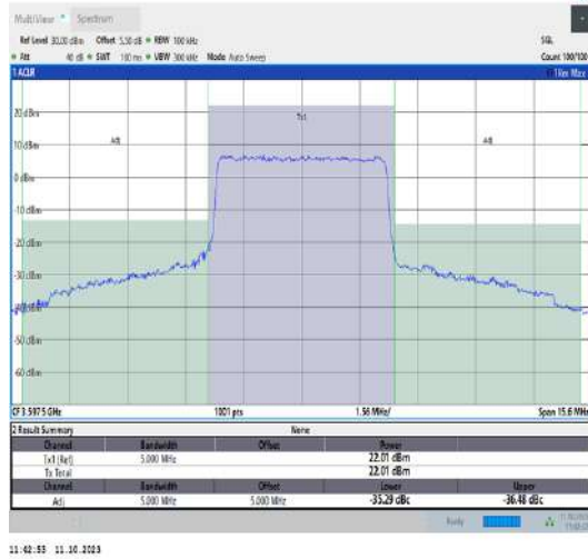
42(3550-3600)-5MHz-QPSK-43565-25RB#0-PASS
