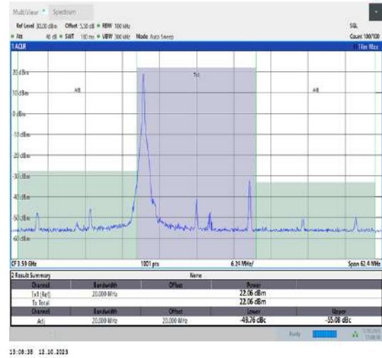
42(3550-3600)-20MHz-QPSK-43490-1RB#0-PASS
