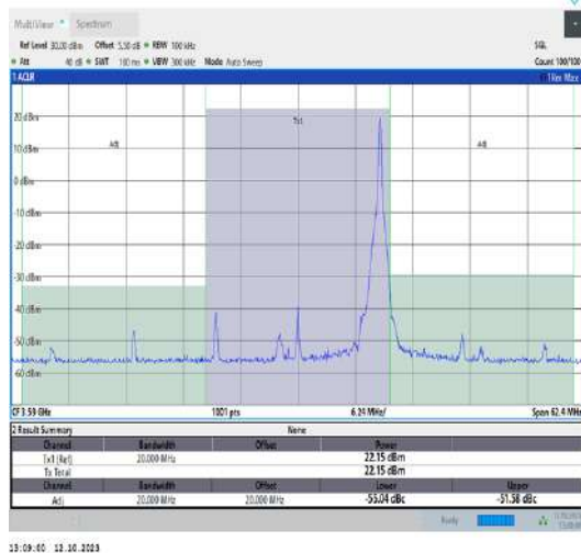
42(3550-3600)-20MHz-QPSK-43490-1RB#99-PASS
