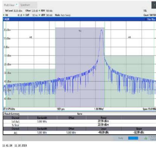
42(3550-3600)-5MHz-QPSK-43340-1RB#24-PASS
