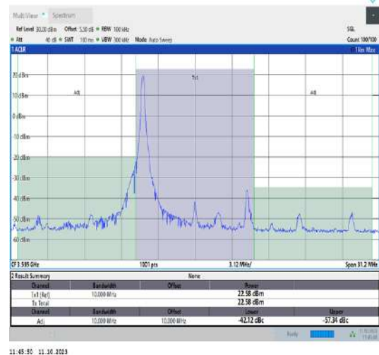
42(3550-3600)-10MHz-QPSK-43540-1RB#0-PASS
