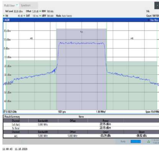
42(3550-3600)-5MHz-QPSK-43115-25RB#0-PASS
