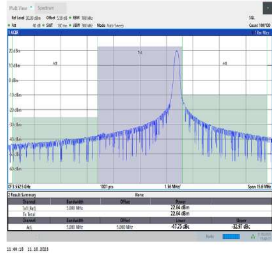
42(3550-3600)-5MHz-QPSK-43115-1RB#24-PASS
