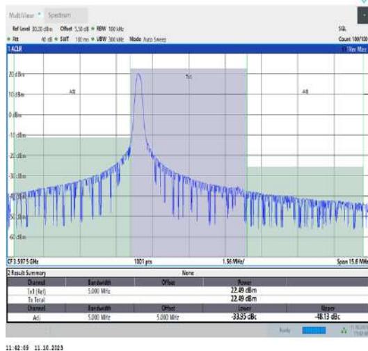
42(3550-3600)-5MHz-QPSK-43565-1RB#0-PASS
