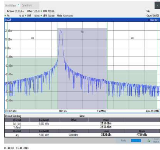
42(3550-3600)-5MHz-QPSK-43340-1RB#0-PASS
