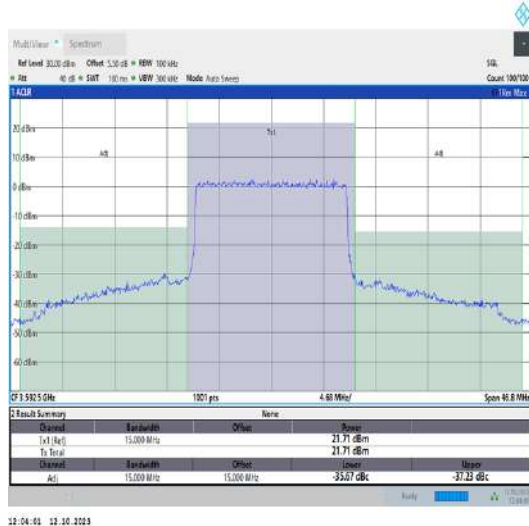
42(3550-3600)-15MHz-QPSK-43515-75RB#0-PASS
