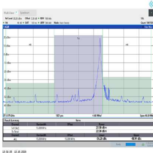
42(3550-3600)-15MHz-QPSK-43340-1RB#74-PASS
