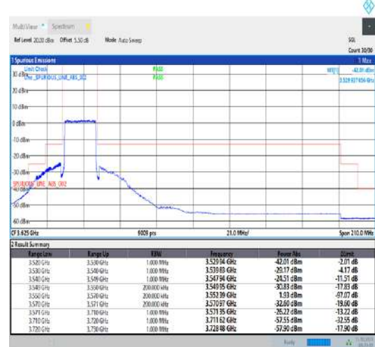
Band42_20MHz_QPSK_43490_100RB#0
