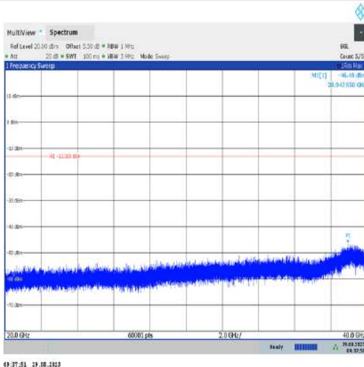
Band42_20MHz_QPSK_43490_1RB#0_20000~40000_20000~40000
