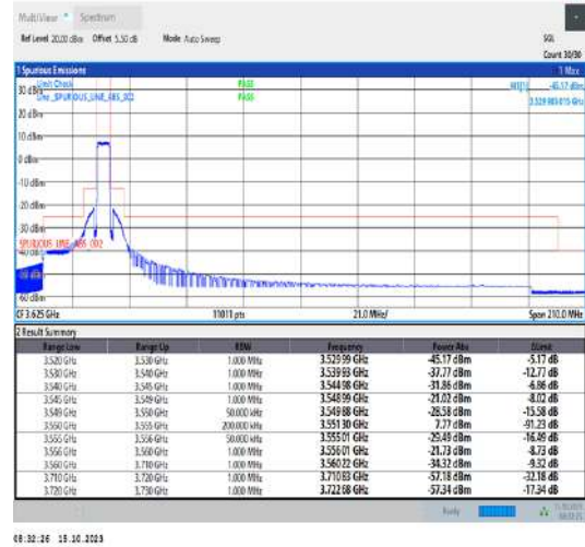
Band42_5MHz_QPSK_43115_25RB#0
