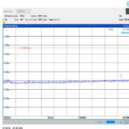
Band42_20MHz_QPSK_43190_1RB#0_0.15~30_0.15~ 30
