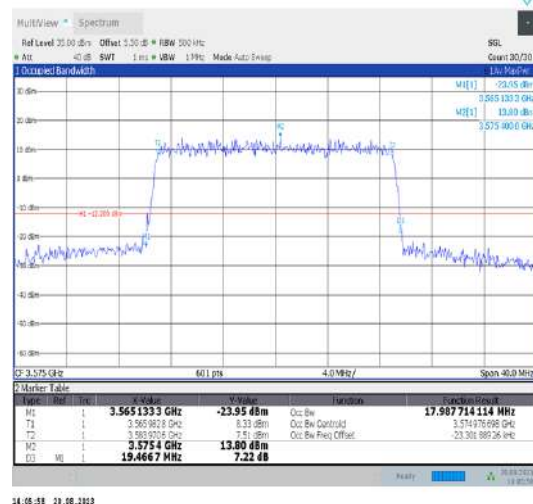
Band42-20MHz-16QAM-43340-100RB#0-PASS
