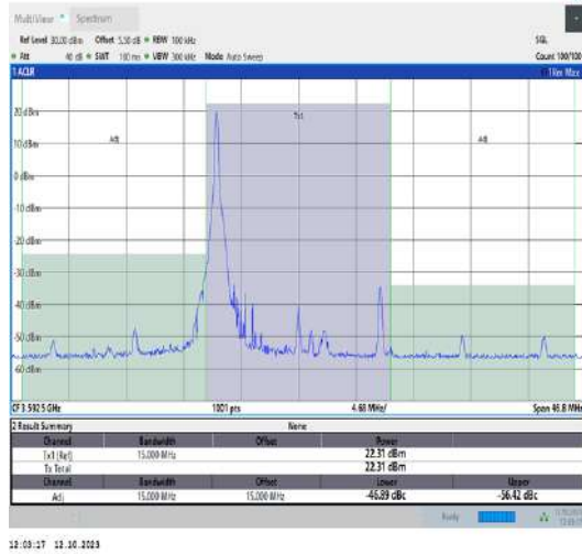
42(3550-3600)-15MHz-QPSK-43515-1RB#0-PASS
