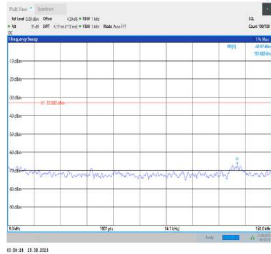
Band42_20MHz_QPSK_43340_1RB#0_0.009~0.15_0.09~0.15
