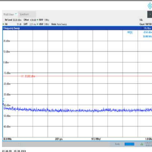
Band42_20MHz_QPSK_43190_1RB#0_30~1000_30~100 0
