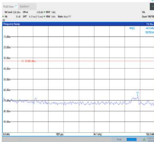
Band42_20MHz_QPSK_43490_1RB#0_0.009~0.15_0.009~0.15
