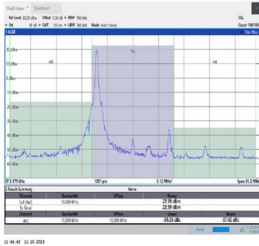
42(3550-3600)-10MHz-QPSK-43340-1RB#0-PASS
