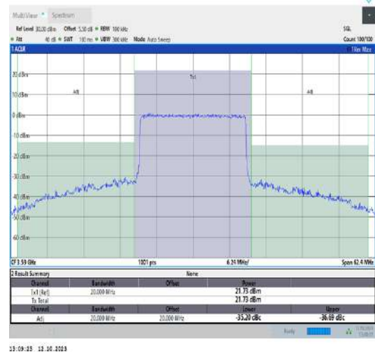
42(3550-3600)-20MHz-QPSK-43490-100RB#0-PASS
