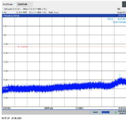
Band42_20MHz_QPSK_43190_1RB#0_20000~40000_20000~40000
