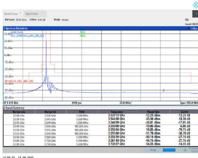
Band48-5MHz-QPSK-55265-25RB#0
