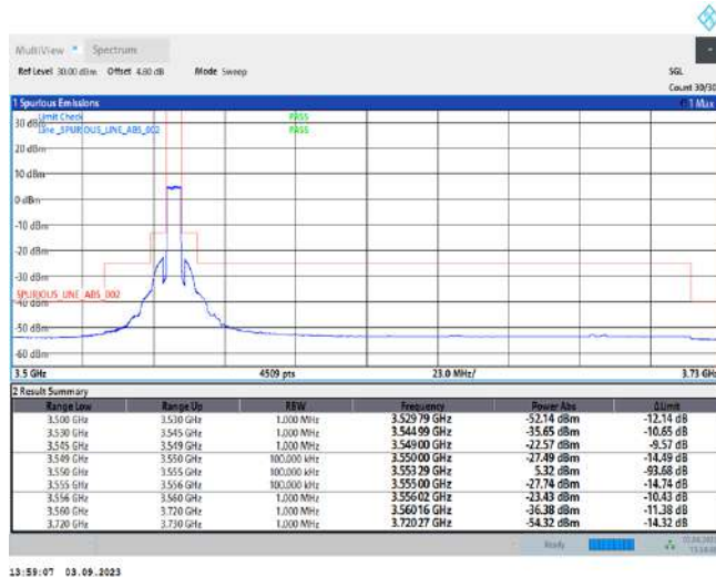
Band48-5MHz-QPSK-55265-25RB#0
