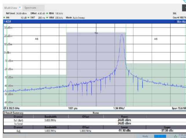
Band48-5MHz-QPSK-55265-1RB#24
