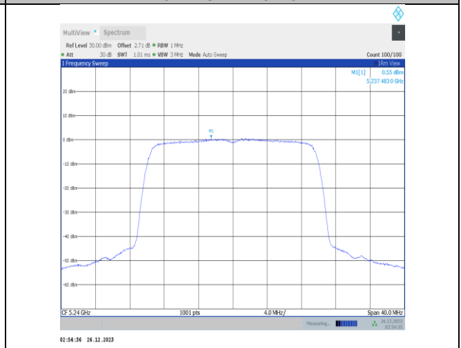
11x20MIMO-Ant4-5240-PASS
