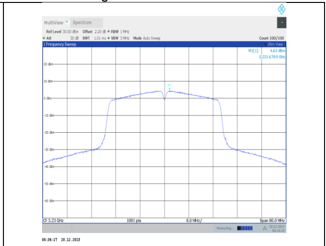
11n40SISO-Ant3-5230-PASS
