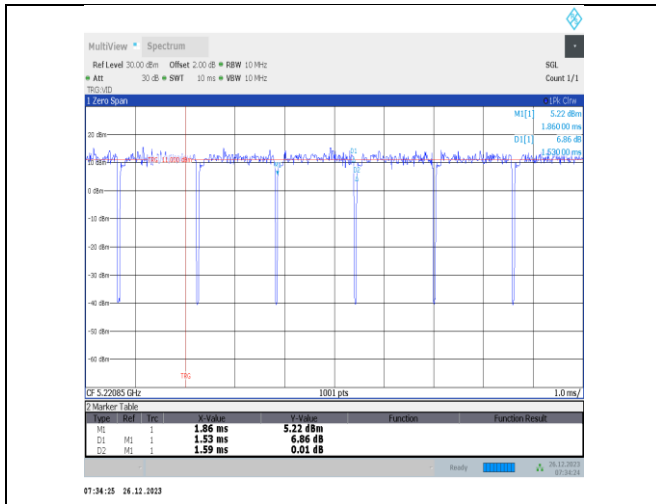
NTNV-11ax20MIMO-Ant1-5220-26Tone-RU4
