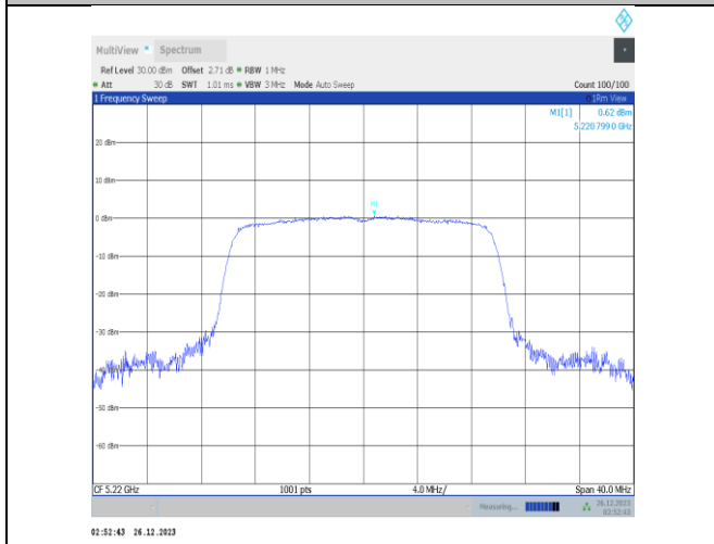
11ax20MIMO-Ant3-5220-PASS
