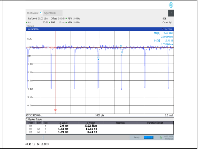
08:41:11 26.12.2023 NTVN-11ax20MIMO-Ant4-5240-26Tone-RU8
