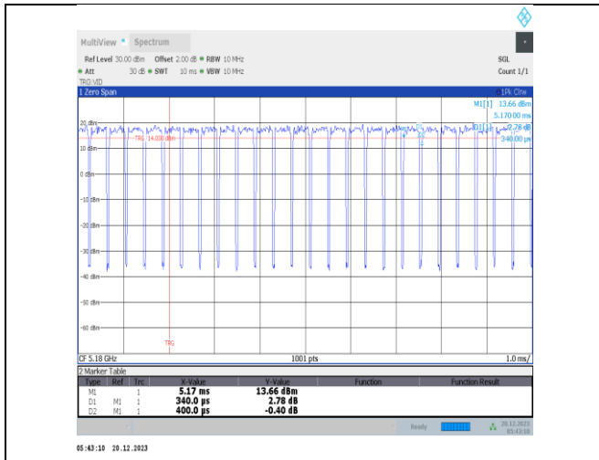
NTNV-11ax20MIMO-Ant1-5180
