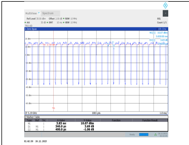
NTNV-11ax40MIMO-Ant3-5190
