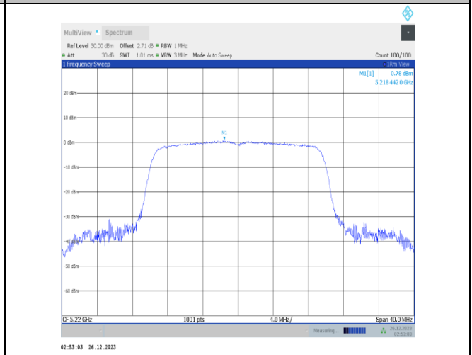
11ax20MIMO-Ant4-5220-PASS
