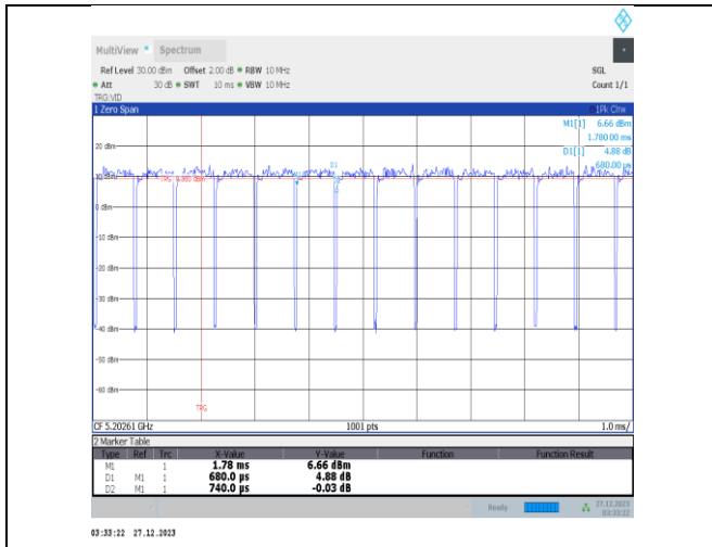
NTVN-11ax80MIMO-Ant2-5210-484Tone-RU65
