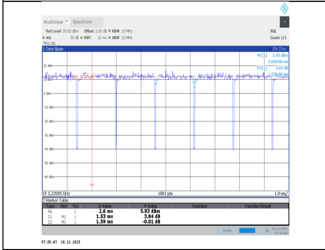
NTNV-11ax20MIMO-Ant3-5220-26Tone-RU4
