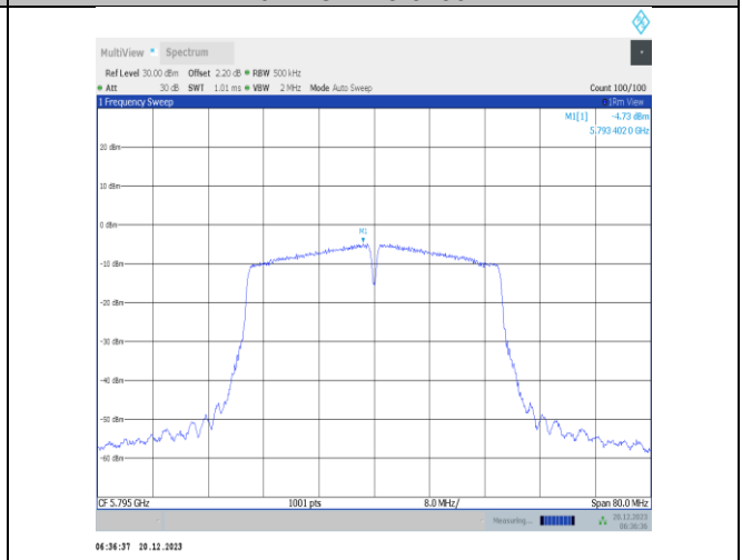
11n40SISO-Ant3-5795-PASS
