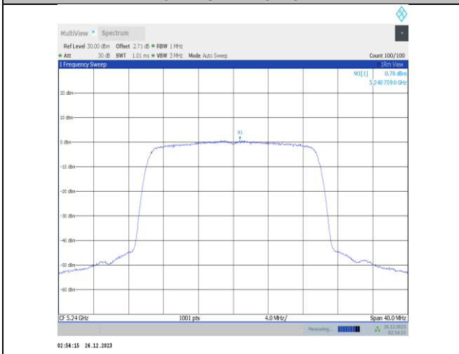
11x20MIMO-Ant3-5240-PASS
