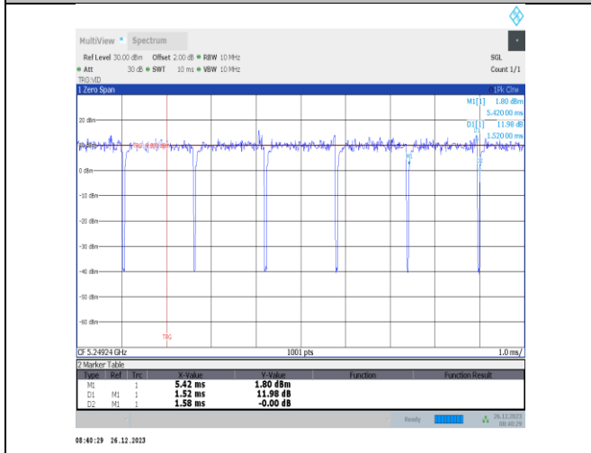
08:40:29 26.12.2023 NTVN-11ax20MIMO-Ant3-5240-26Tone-RU8
