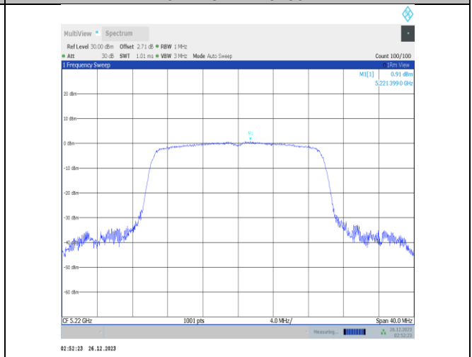
11ax20MIMO-Ant2-5220-PASS
