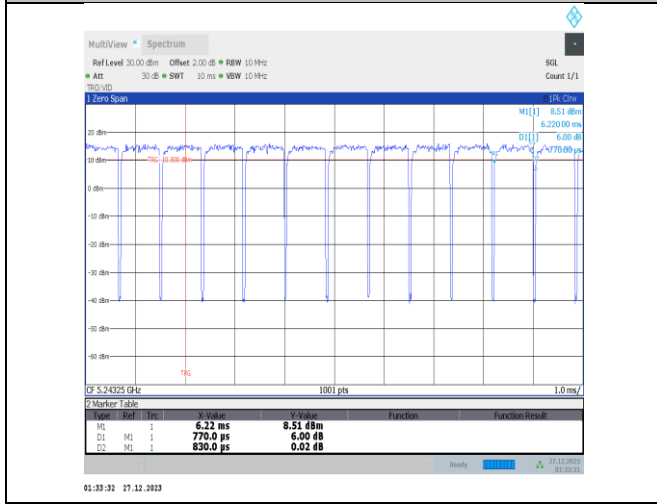
NTNV-11ax20MIMO-Ant1-5240-106Tone-RU54
