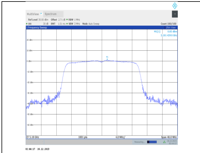
11ax20MIMO-Ant3-5180-PASS
