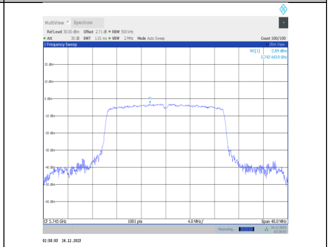
11x20MIMO-Ant2-5745-PASS
