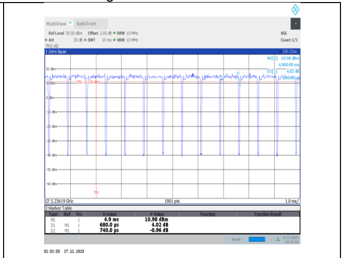
NTVN-11ax40MIMO-Ant2-5230-242Tone-RU62
