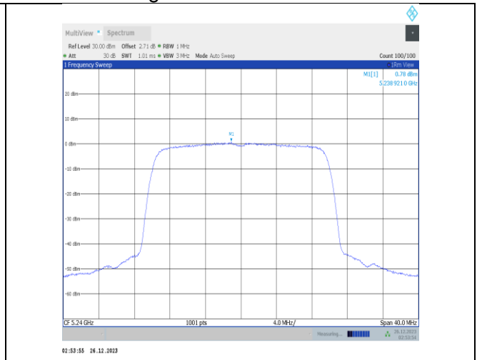
11x20MIMO-Ant2-5240-PASS
