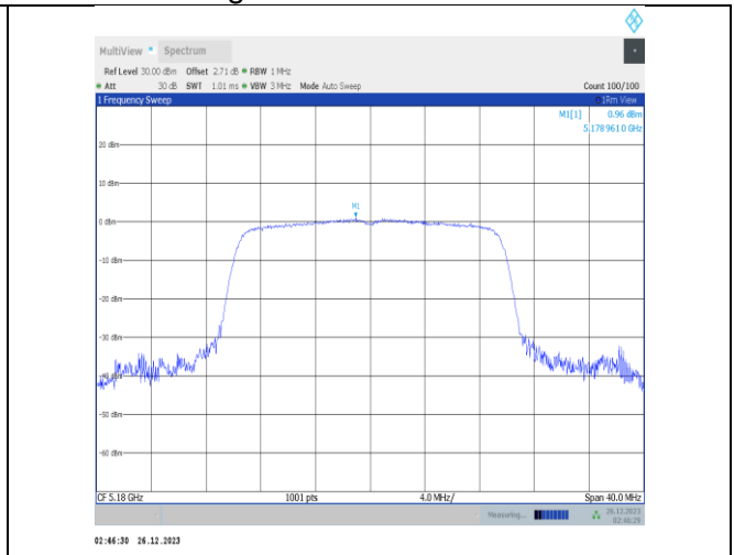
11ax20MIMO-Ant4-5180-PASS
