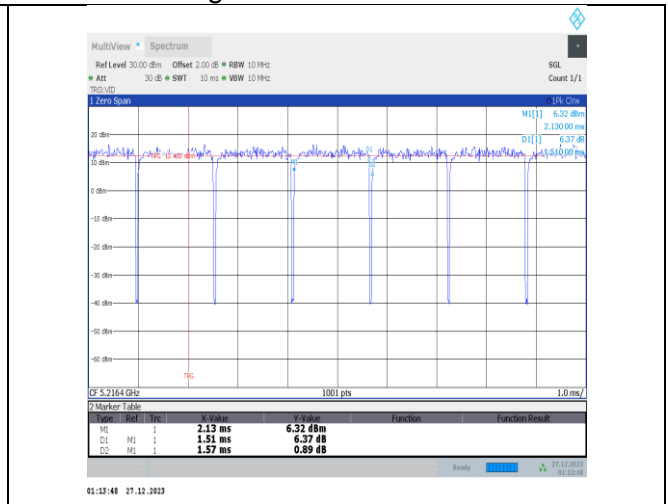
NTNV-11ax20MIMO-Ant1-5220-52Tone-RU38
