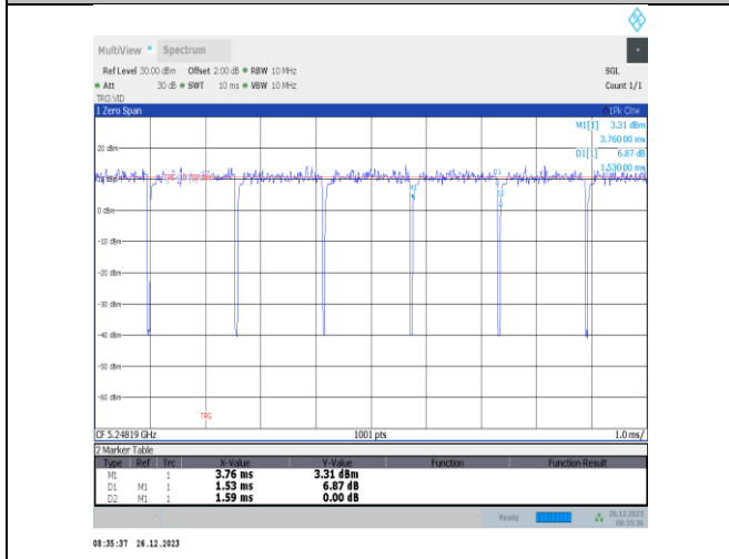
NTNV-11ax20MIMO-Ant1-5240-26Tone-RU8
