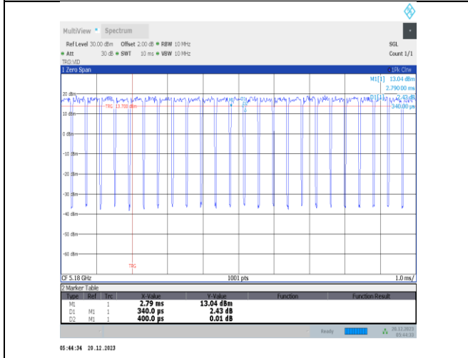
NTNV-11ax20MIMO-Ant3-5180
