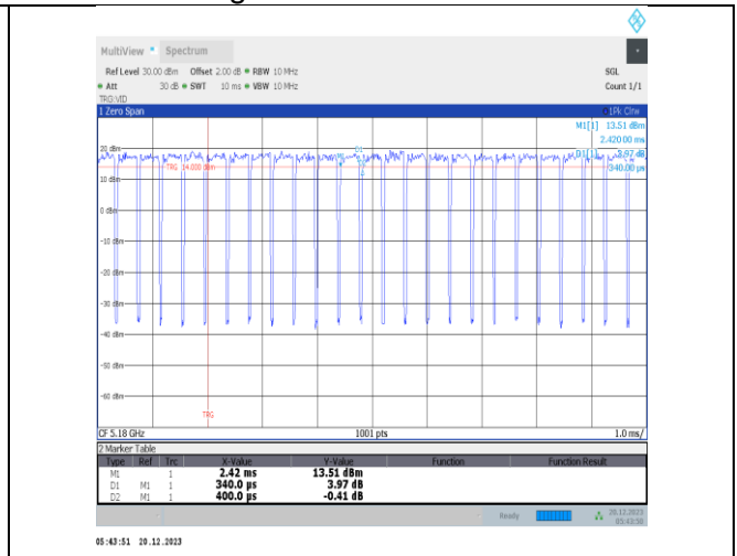
NTNV-11ax20MIMO-Ant2-5180
