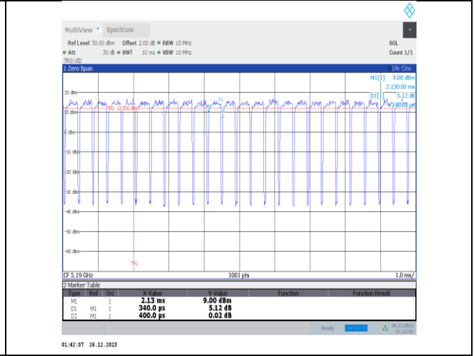
NTNV-11ax40MIMO-Ant2-5190
