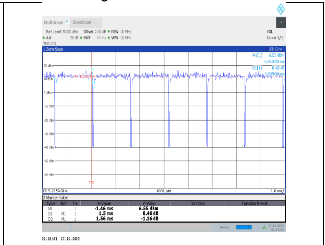
NTNV-11ax20MIMO-Ant4-5220-52Tone-RU38
