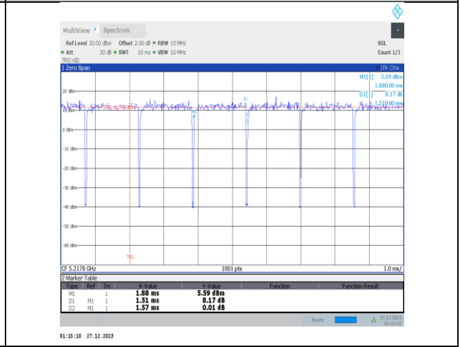
NTNV-11ax20MIMO-Ant3-5220-52Tone-RU38
