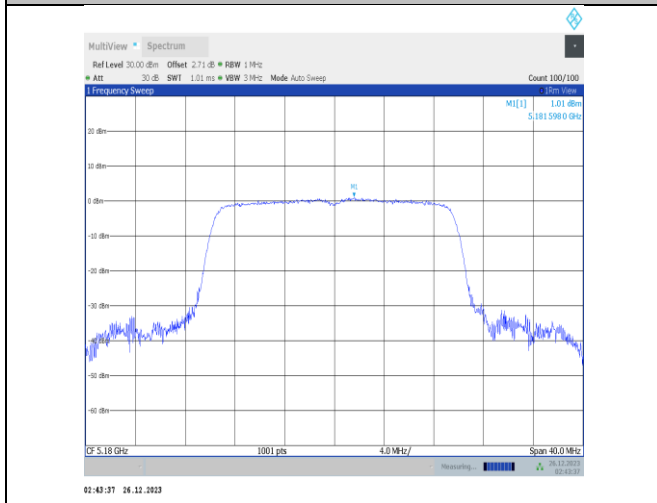
11ax20MIMO-Ant1-5180-PASS
