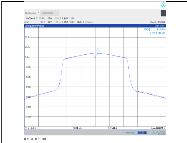
11n40SISO-Ant3-5190-PASS
