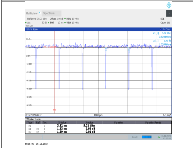
NTNV-11ax20MIMO-Ant2-5220-26Tone-RU4
