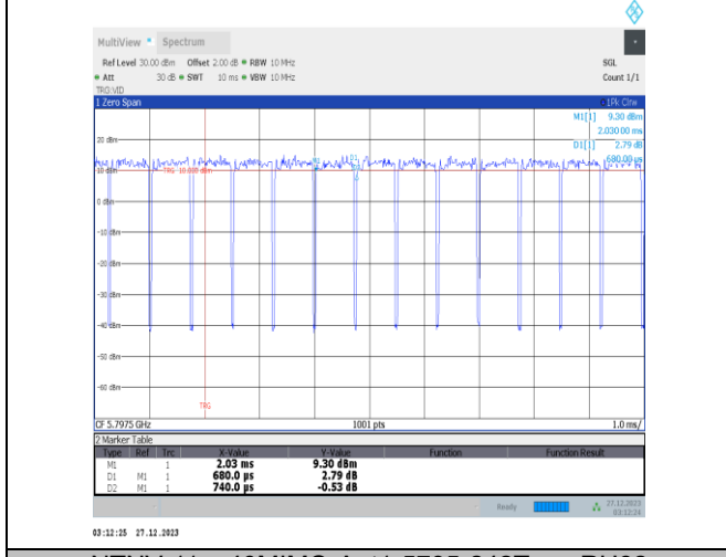
NTVN-11ax40MIMO-Ant1-5795-242Tone-RU62
