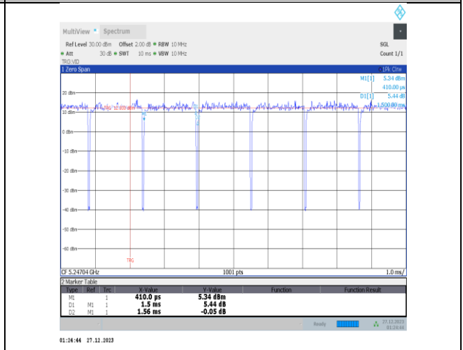
NTNV-11ax20MIMO-Ant1-5240-52Tone-RU40
