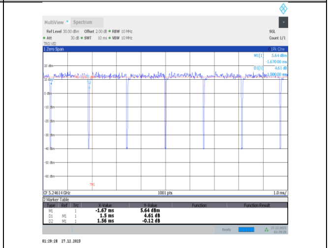
01:29:28 27.12.2023 NTVN-11ax20MIMO-Ant3-5240-52Tone-RU40
