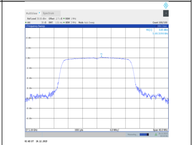
11ax20MIMO-Ant2-5180-PASS
