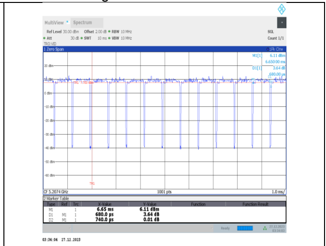
NTVN-11ax80MIMO-Ant3-5210-484Tone-RU65
