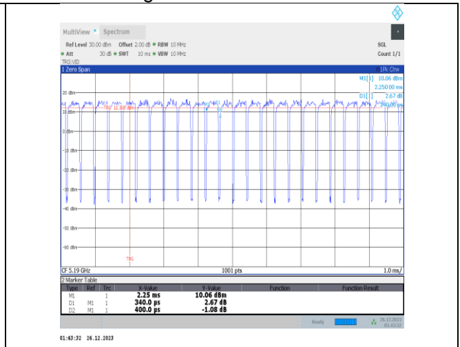
NTNV-11ax40MIMO-Ant4-5190
