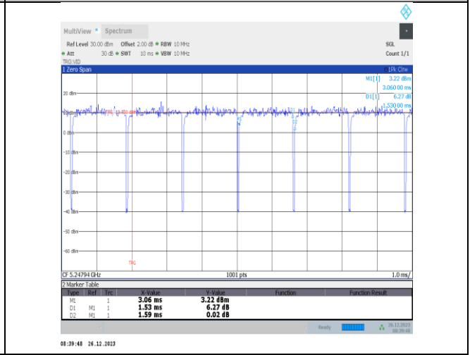
NTNV-11ax20MIMO-Ant2-5240-26Tone-RU8
