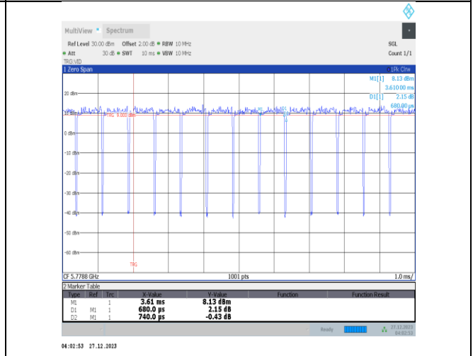
NTVN-11ax80MIMO-Ant1-5775-484Tone-RU66
