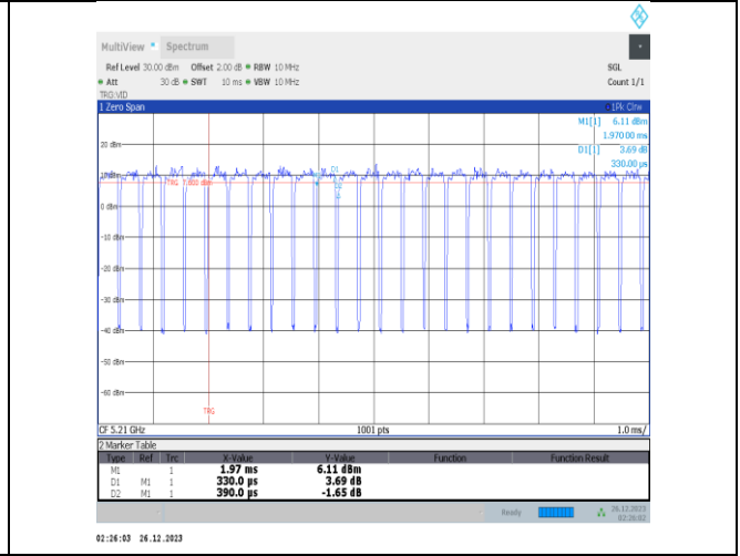
NTNV-11ax80MIMO-Ant4-5210
