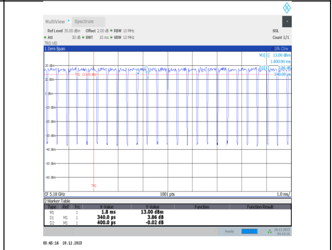
NTNV-11ax20MIMO-Ant4-5180
