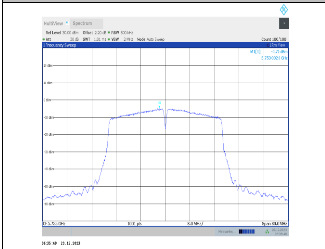
11n40SISO-Ant3-5755-PASS
