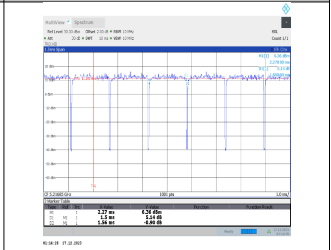
NTNV-11ax20MIMO-Ant2-5220-52Tone-RU38
