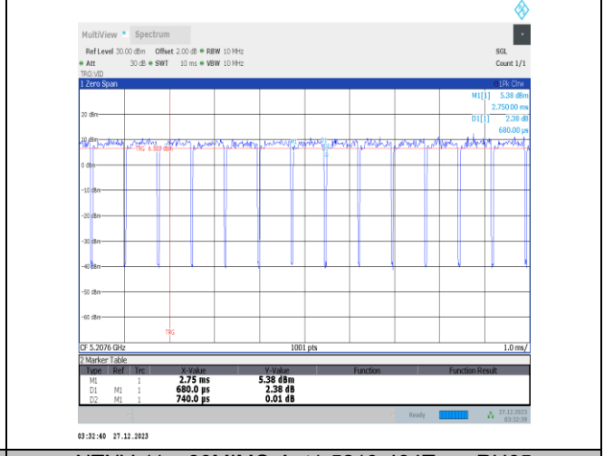
NTVN-11ax80MIMO-Ant1-5210-484Tone-RU65
