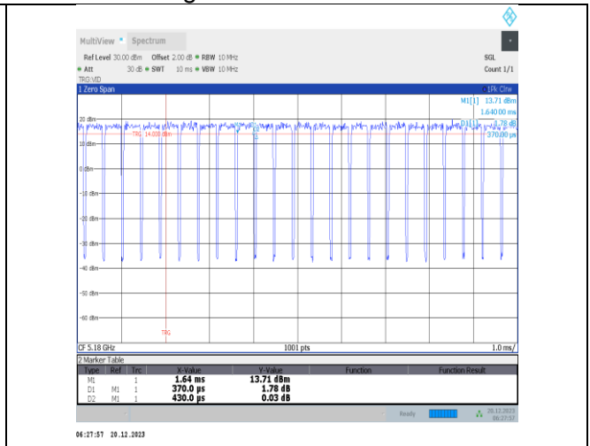
NTNV-11ac20MIMO-Ant2-5180
