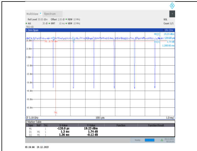
NTNV-11n20SISO-Ant3-5180
