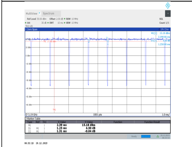
NTNV-11n40SISO-Ant3-5190
