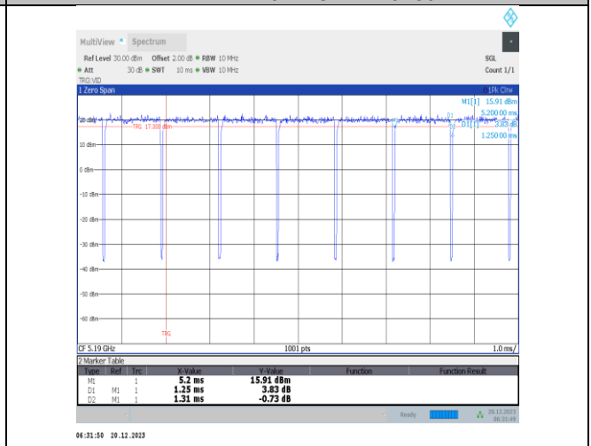
NTNV-11n40SISO-Ant2-5190
