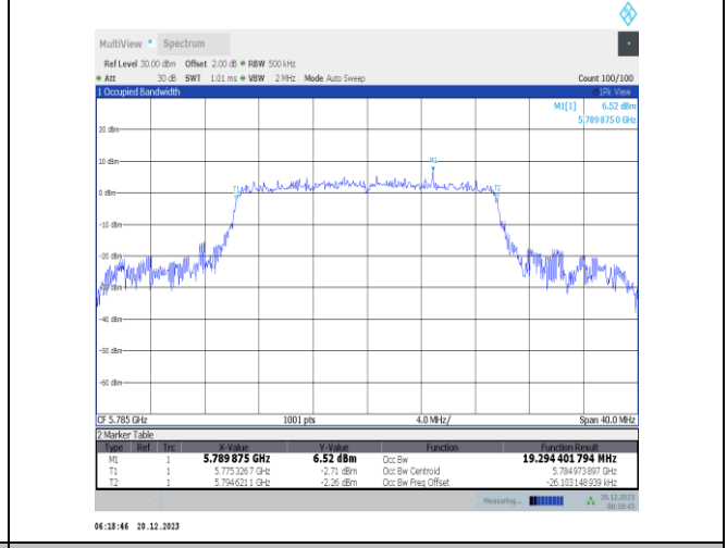
11ax20MIMO-Ant4-5785
