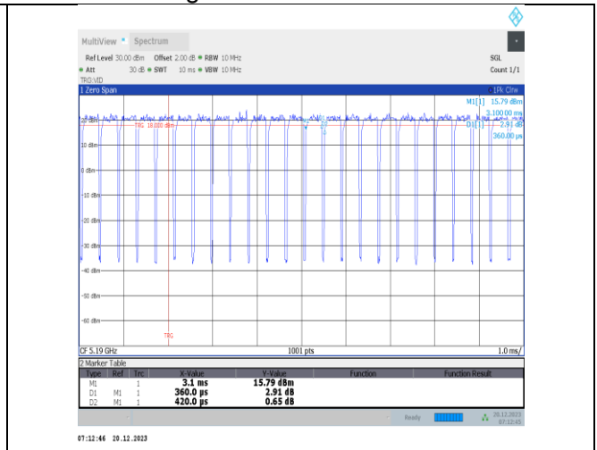
NTNV-11ac40MIMO-Ant4-5190
