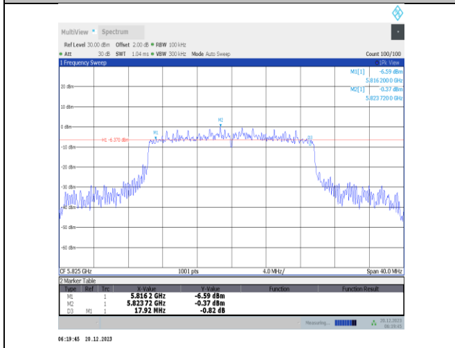
11ax20MIMO-Ant1-5825-PASS
