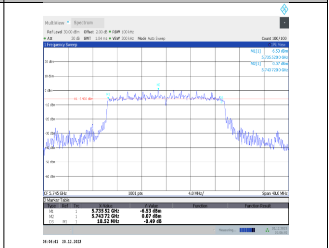
11ax20MIMO-Ant4-5745-PASS
