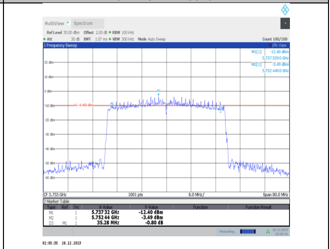
11ax40MIMO-Ant2-5755-PASS
