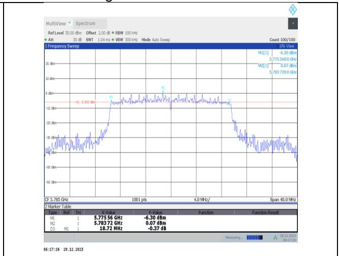
11ax20MIMO-Ant2-5785-PASS
