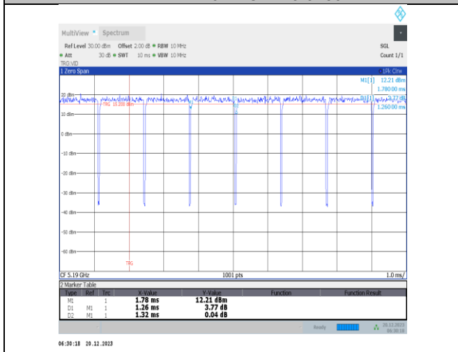
NTNV-11n40SISO-Ant1-5190
