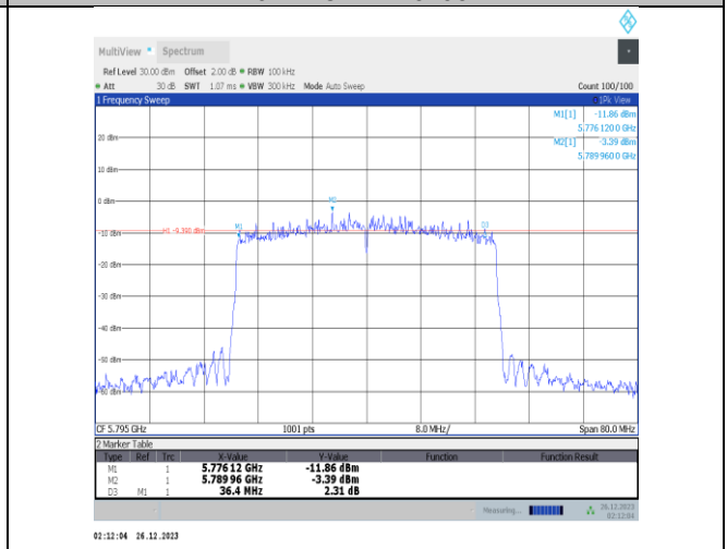
11ax40MIMO-Ant4-5795-PASS
