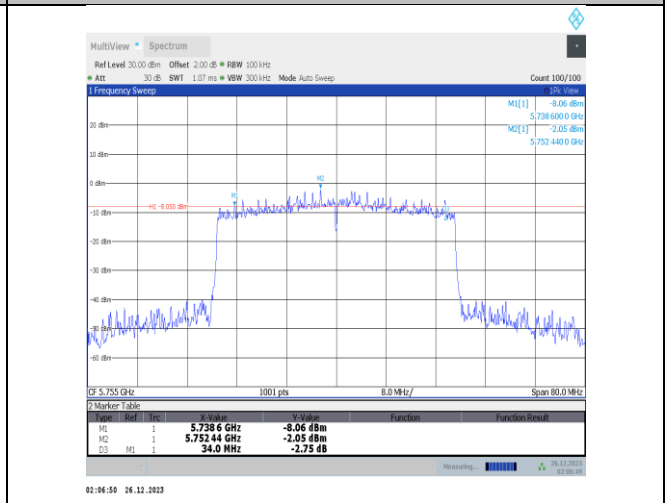
11ax40MIMO-Ant4-5755-PASS
