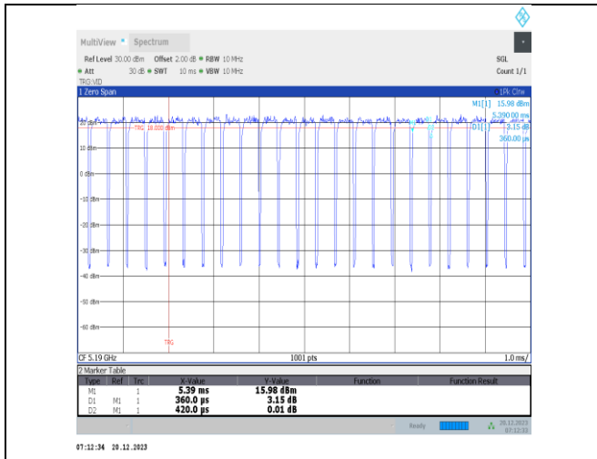
NTNV-11ac40MIMO-Ant3-5190
