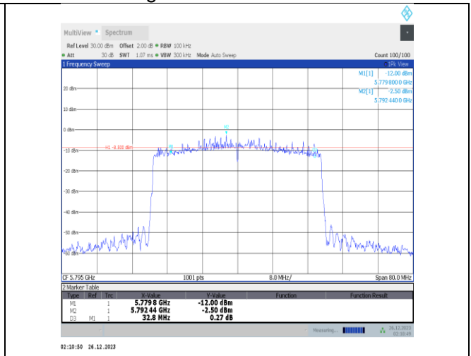
11ax40MIMO-Ant2-5795-PASS
