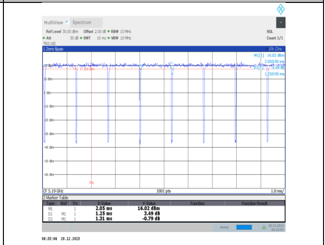
NTNV-11n40SISO-Ant4-5190
