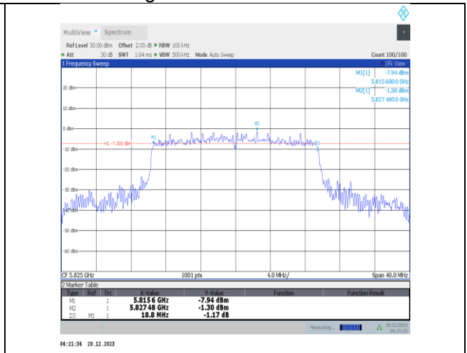
11ax20MIMO-Ant4-5825-PASS
