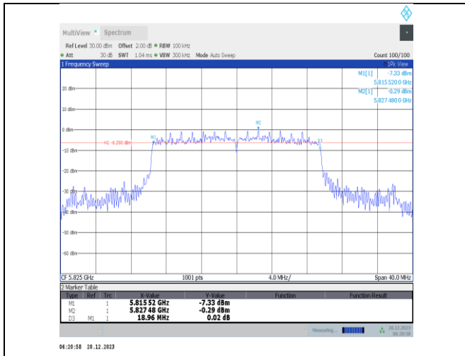
11ax20MIMO-Ant3-5825-PASS
