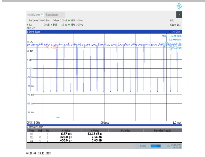
NTNV-11ac20MIMO-Ant3-5180
