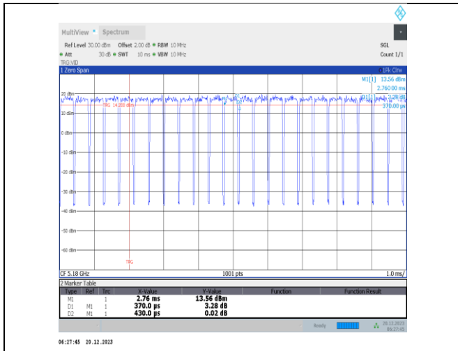
NTNV-11ac20MIMO-Ant1-5180
