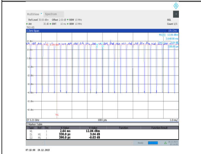
NTNV-11ac80MIMO-Ant3-5210
