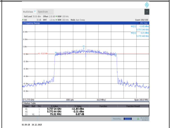
11ax80MIMO-Ant2-5775-PASS
