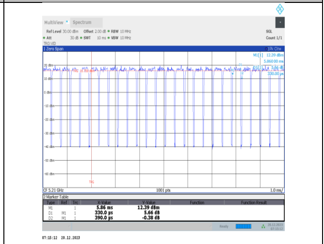
NTNV-11ac80MIMO-Ant4-5210
