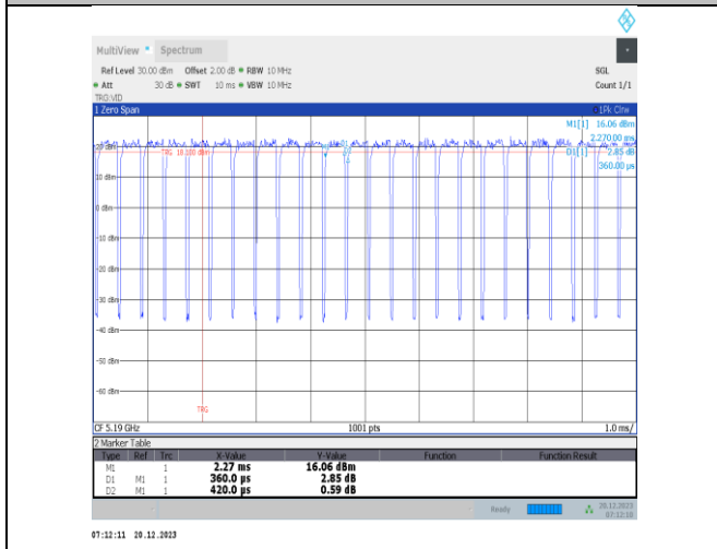
NTNV-11ac40MIMO-Ant1-5190
