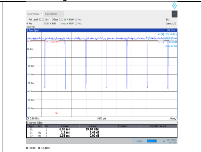
NTNV-11n20SISO-Ant4-5180
