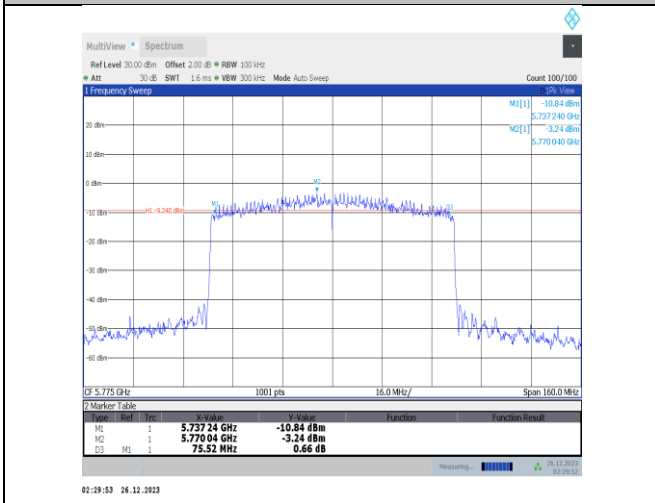
11ax80MIMO-Ant1-5775-PASS
