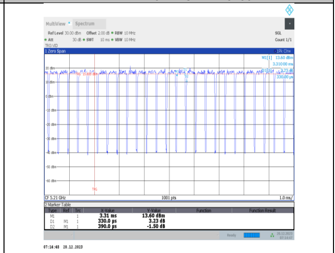
NTNV-11ac80MIMO-Ant2-5210
