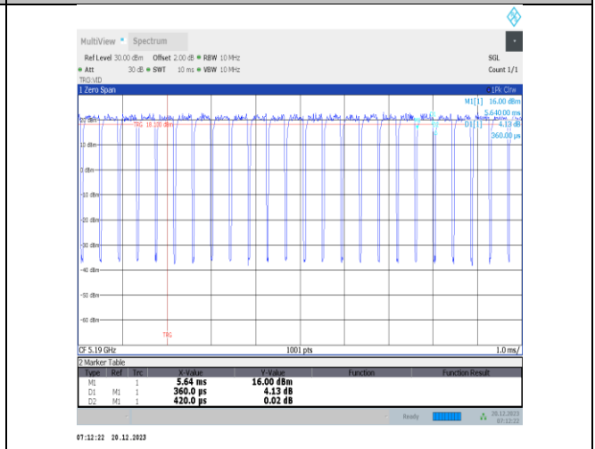
NTNV-11ac40MIMO-Ant2-5190
