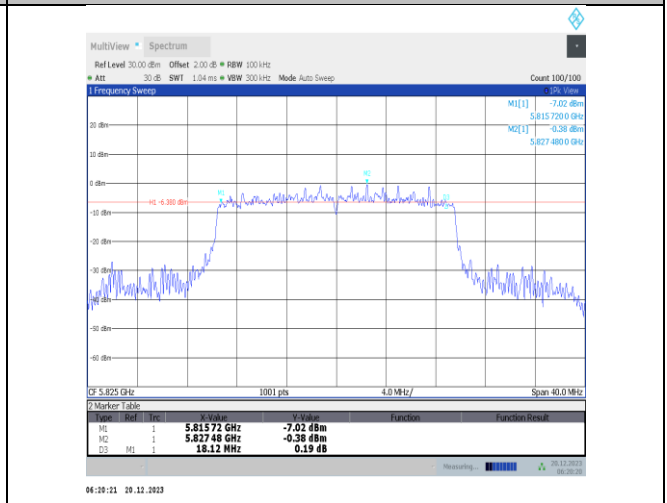
11ax20MIMO-Ant2-5825-PASS
