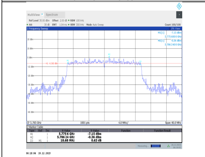
11ax20MIMO-Ant3-5785-PASS
