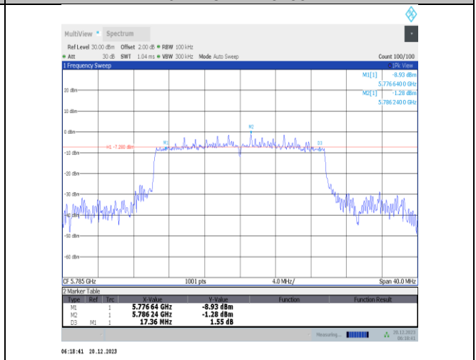
11ax20MIMO-Ant4-5785-PASS
