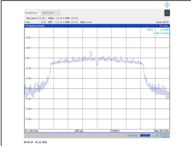
11ax20MIMO-Ant2-2462-0~Reference-PASS
