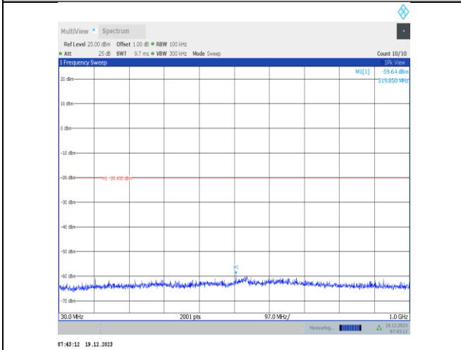
11n40SISO-Ant2-2437-30~1000-PASS
