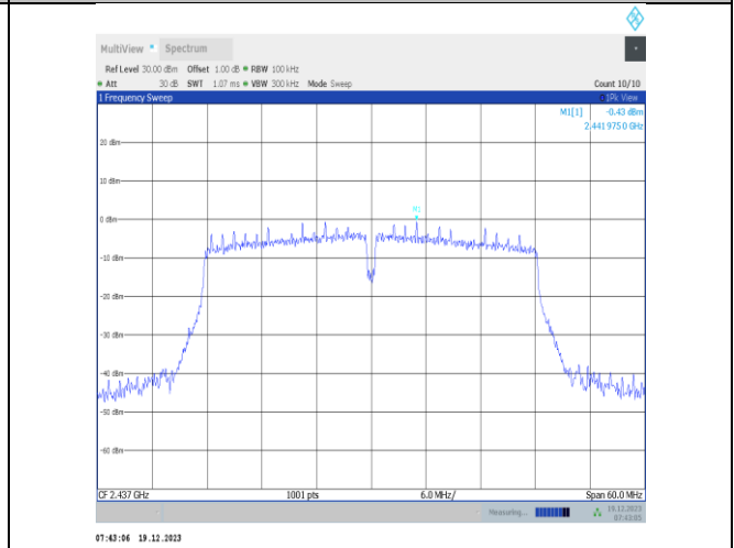
11n40SISO-Ant2-2437-0~Reference-PASS
