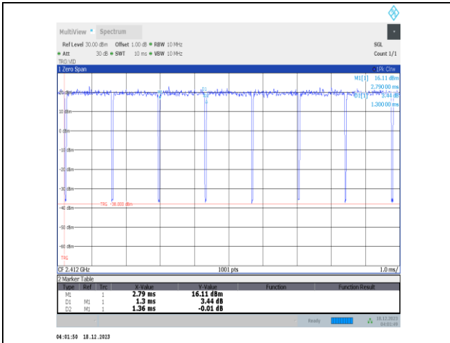
NTVN-11n20SISO-Ant2-2412
