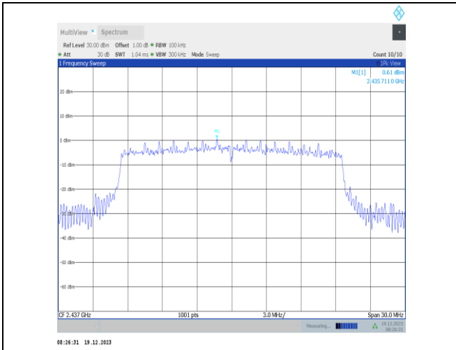
11ax20MIMO-Ant2-2437-0~Reference-PASS
