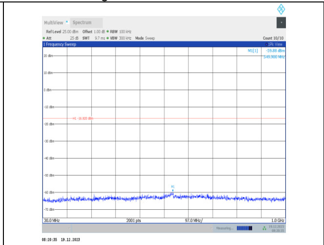
11ax20MIMO-Ant2-2412-30~1000-PASS
