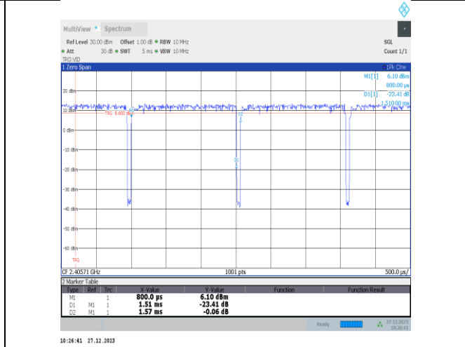
NTVN-11ax20MIMO-Ant3-2412-52Tone-RU37
