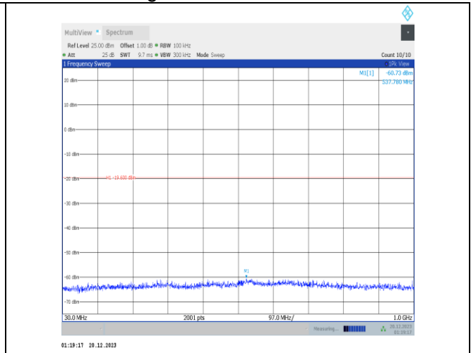
11ax40MIMO-Ant2-2452-30~1000-PASS
