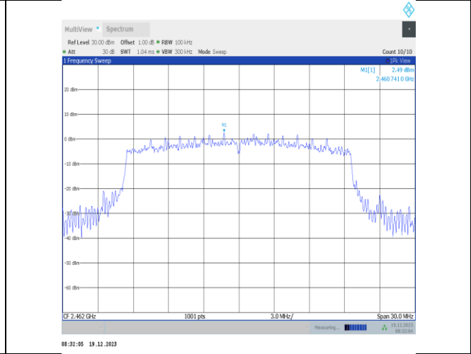
11ax20MIMO-Ant1-2462-0~Reference-PASS
