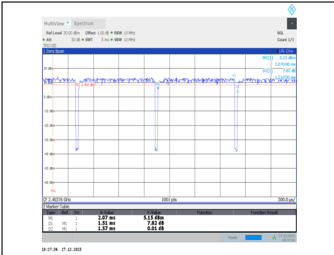
NTVN-11ax20MIMO-Ant4-2412-52Tone-RU37
