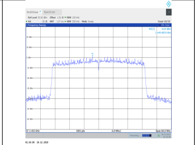
11ax40MIMO-Ant3-2452-0~Reference-PASS
