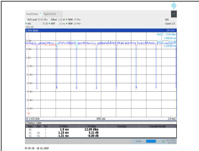
NTVN-11n40SISO-Ant4-2422
