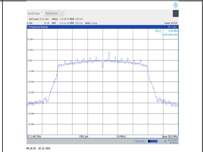
11n20SISO-Ant2-2462-0~Reference-PASS
