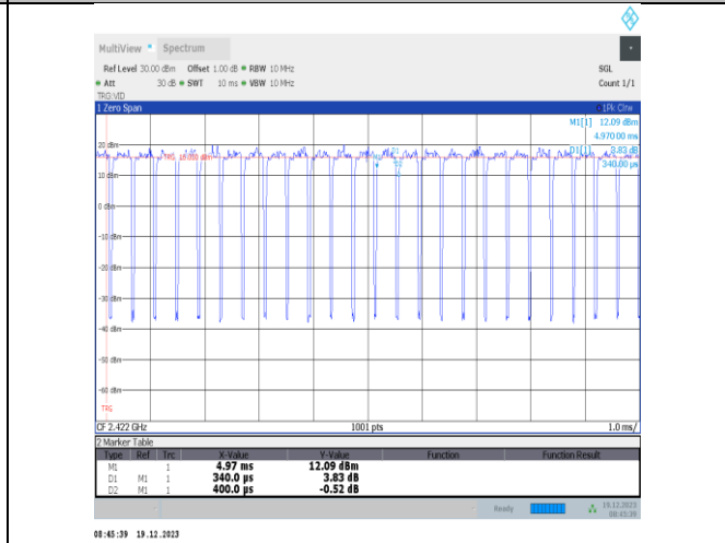
NTVN-11ax40MIMO-Ant1-2422
