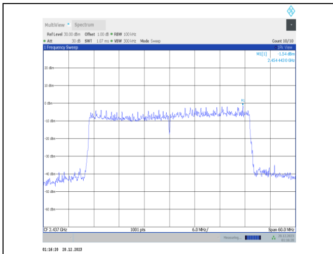
11ax40MIMO-Ant4-2437-0~Reference-PASS
