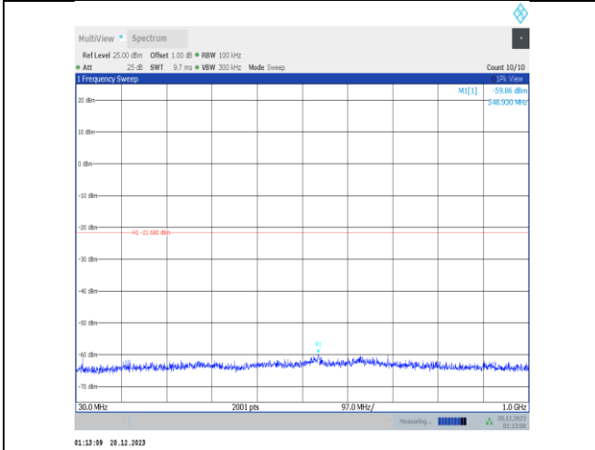
11ax40MIMO-Ant1-2437-30~1000-PASS
