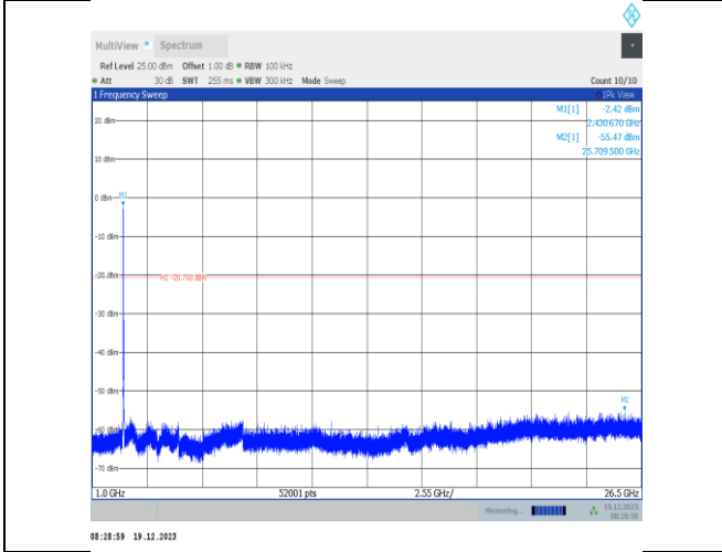
11ax20MIMO-Ant4-2437-1000~26500-PASS
