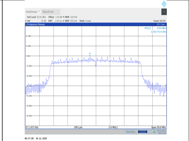
11ax20MIMO-Ant3-2437-0~Reference-PASS
