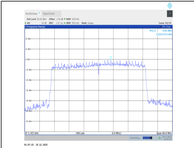
11ax40MIMO-Ant2-2422-0~Reference-PASS
