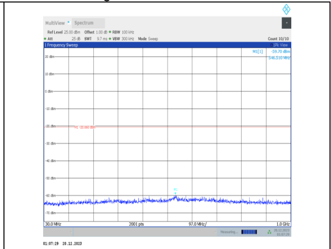
11ax40MIMO-Ant2-2422-30~1000-PASS
