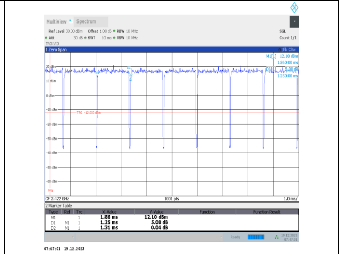
NTVN-11n40SISO-Ant3-2422
