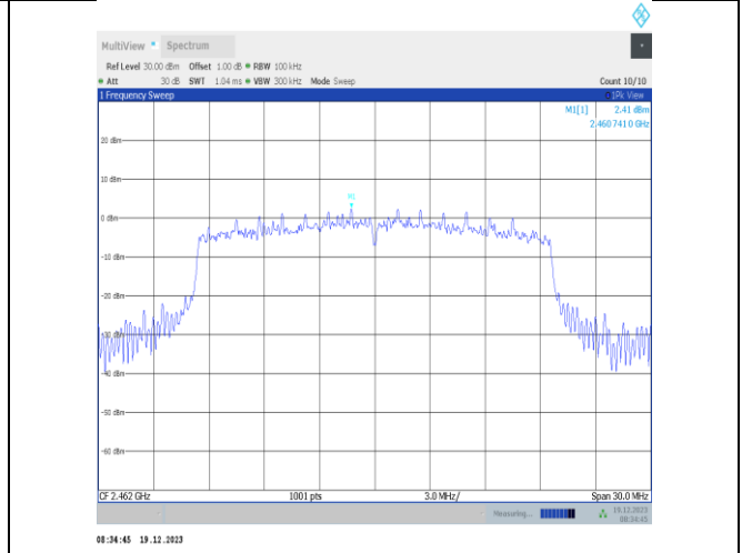
11ax20MIMO-Ant3-2462-0~Reference-PASS
