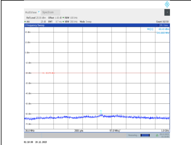
11ax40MIMO-Ant3-2422-30~1000-PASS
