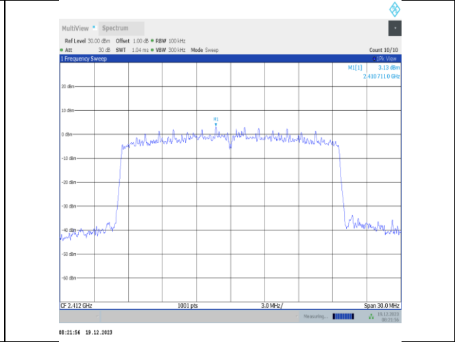
11ax20MIMO-Ant3-2412-0~Reference-PASS
