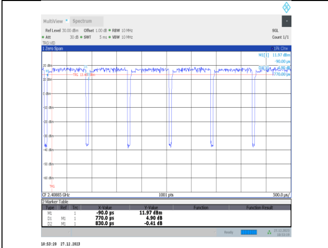
NTVN-11ax20MIMO-Ant3-2412-106Tone-RU53
