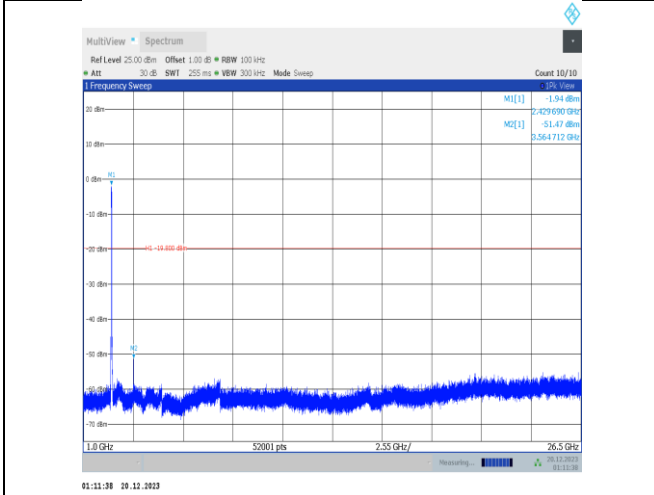
11ax40MIMO-Ant4-2422-1000~26500-PASS
