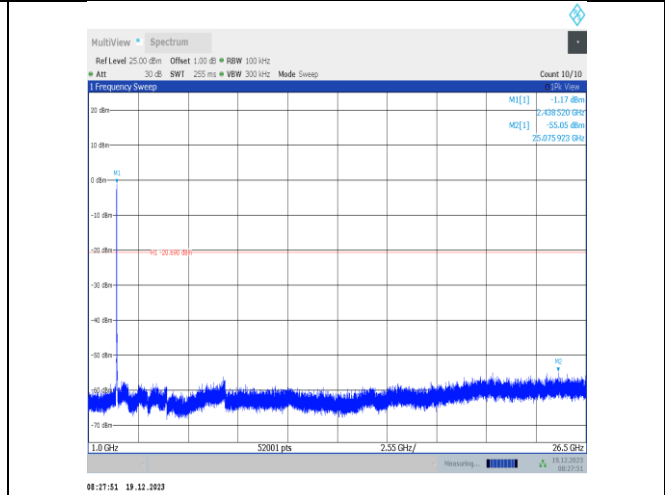
11ax20MIMO-Ant3-2437-1000~26500-PASS
