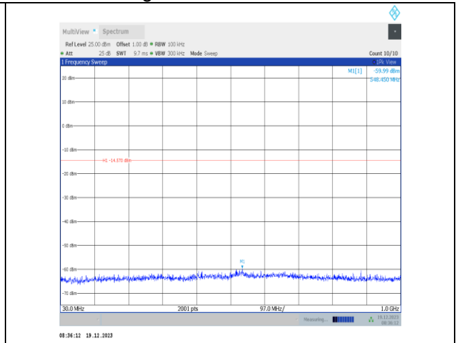
11ax20MIMO-Ant4-2462-30~1000-PASS
