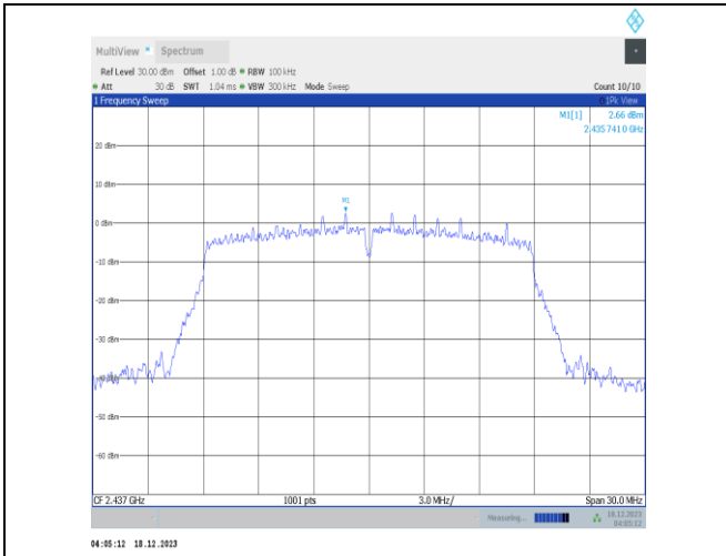
11n20SISO-Ant2-2437-0~Reference-PASS
