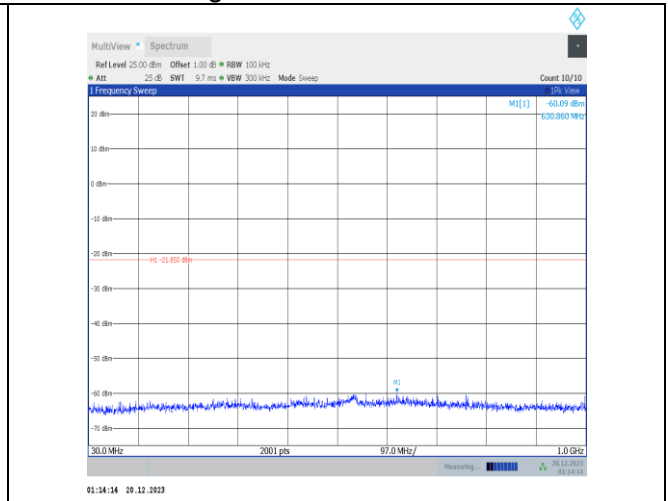
11ax40MIMO-Ant2-2437-30~1000-PASS
