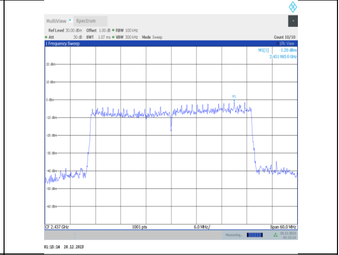
11ax40MIMO-Ant3-2437-0~Reference-PASS
