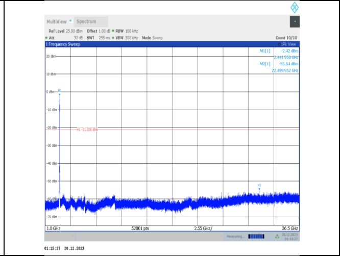
11ax40MIMO-Ant3-2437-1000~26500-PASS
