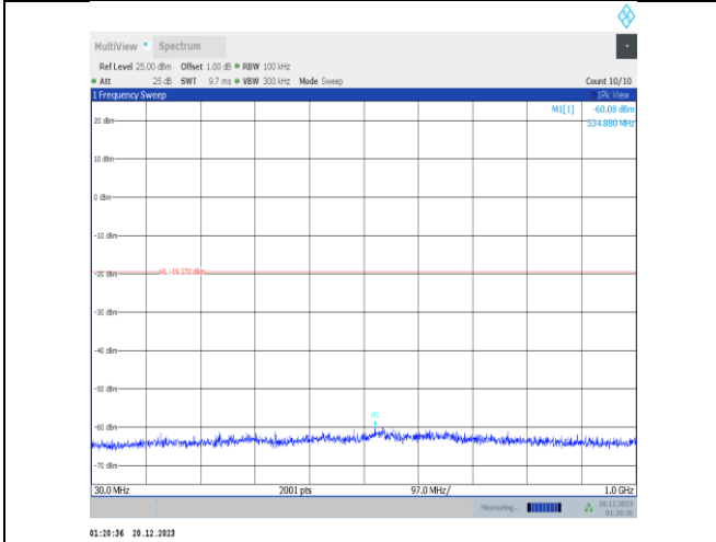
11ax40MIMO-Ant3-2452-30~1000-PASS
