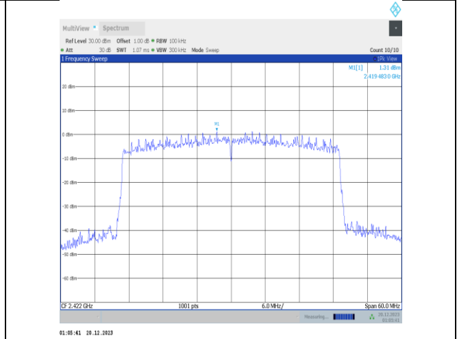
11ax40MIMO-Ant1-2422-0~Reference-PASS
