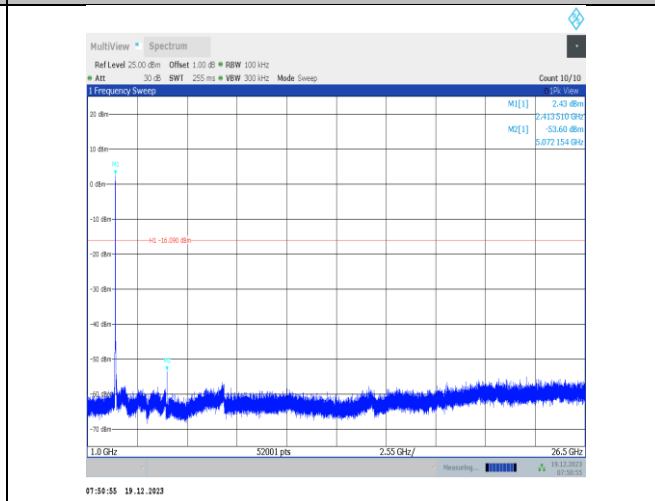
11ax20MIMO-Ant1-2412-1000~26500-PASS
