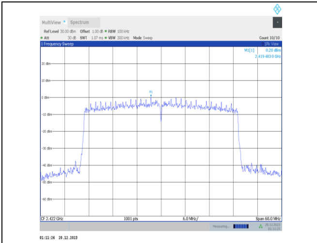
11ax40MIMO-Ant4-2422-0~Reference-PASS
