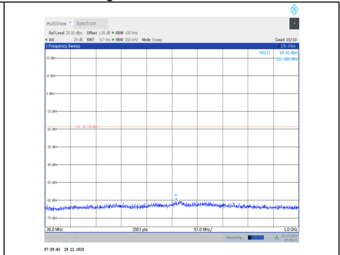
11n40SISO-Ant2-2422-30~1000-PASS
