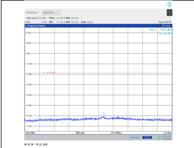
11ax20MIMO-Ant1-2437-30~1000-PASS
