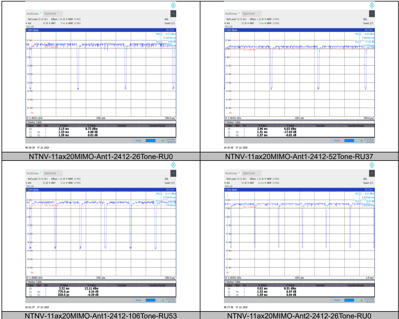
NTVN-11ax20MIMO-Ant1-2412-106Tone-RU53
