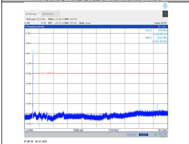
11n40SISO-Ant2-2452-1000~26500-PASS
