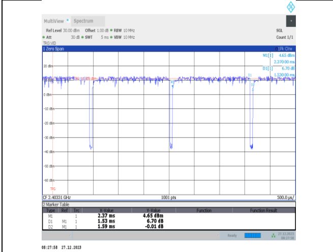
NTVN-11ax20MIMO-Ant3-2412-26Tone-RU0
