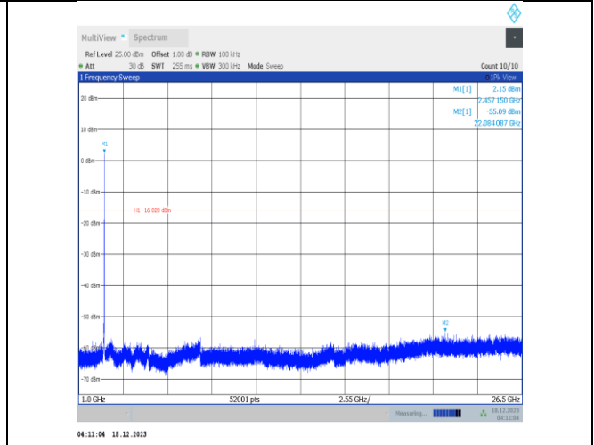
11n20SISO-Ant2-2462-1000~26500-PASS
