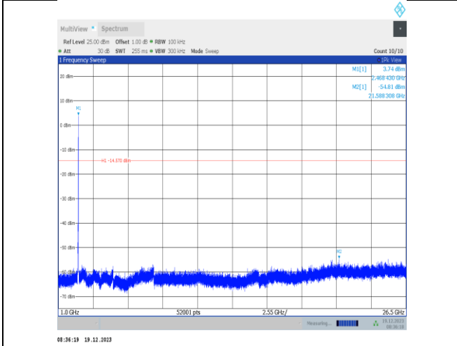
11ax20MIMO-Ant4-2462-1000~26500-PASS
