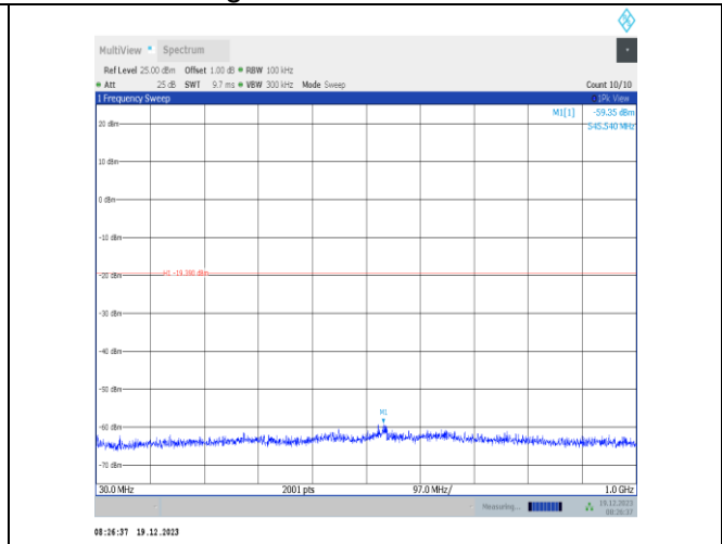
11ax20MIMO-Ant2-2437-30~1000-PASS
