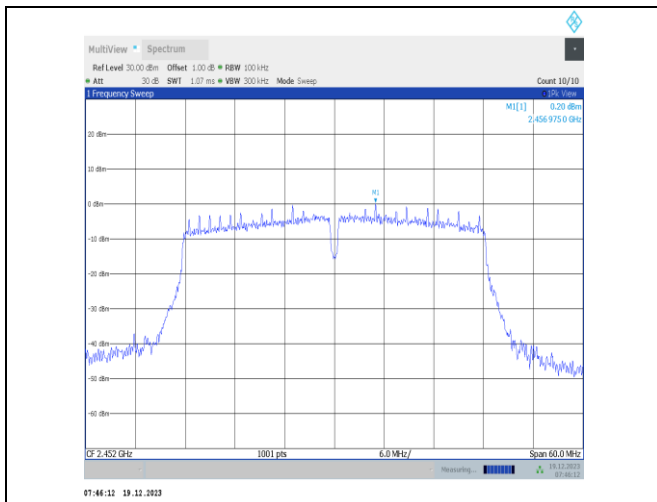
11n40SISO-Ant2-2452-0~Reference-PASS
