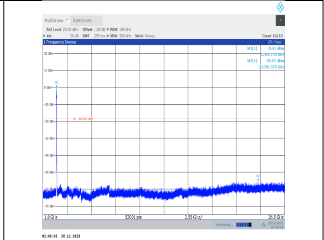
11ax40MIMO-Ant1-2422-1000~26500-PASS
