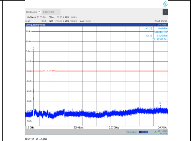
11ax40MIMO-Ant3-2452-1000~26500-PASS
