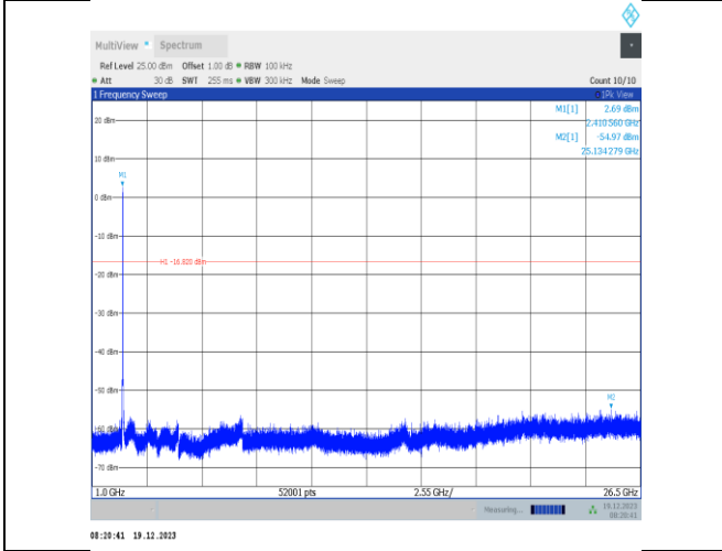
11ax20MIMO-Ant2-2412-1000~26500-PASS
