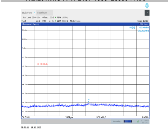
11ax20MIMO-Ant1-2462-30~1000-PASS
