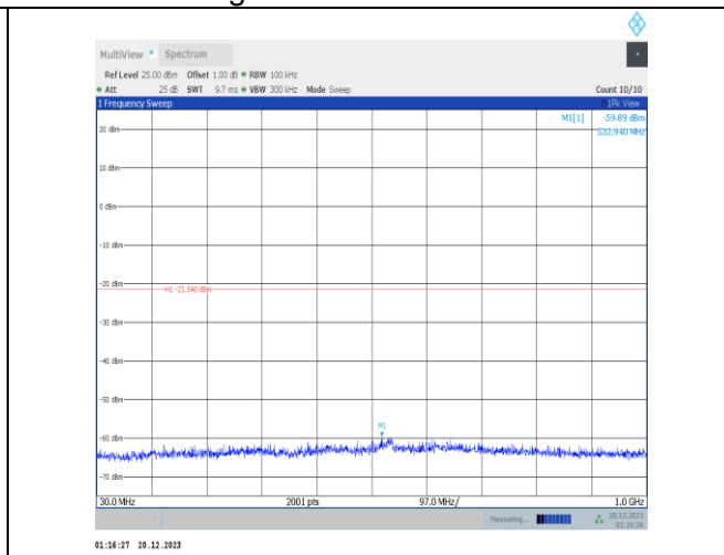
11ax40MIMO-Ant4-2437-30~1000-PASS
