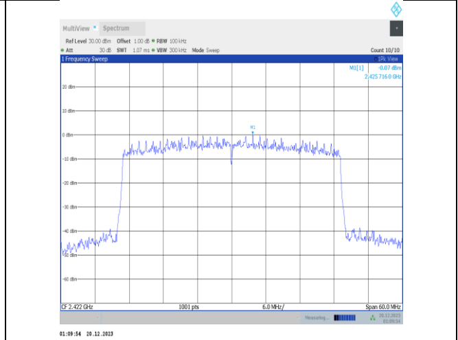
11ax40MIMO-Ant3-2422-0~Reference-PASS
