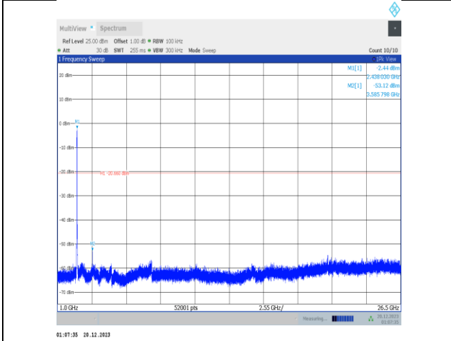
11ax40MIMO-Ant2-2422-1000~26500-PASS
