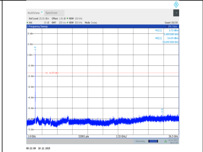
11ax20MIMO-Ant3-2412-1000~26500-PASS
