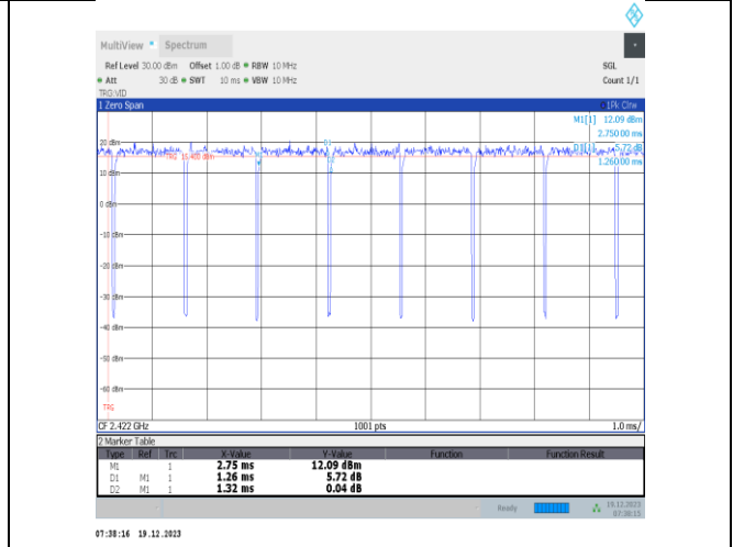
NTVN-11n40SISO-Ant1-2422
