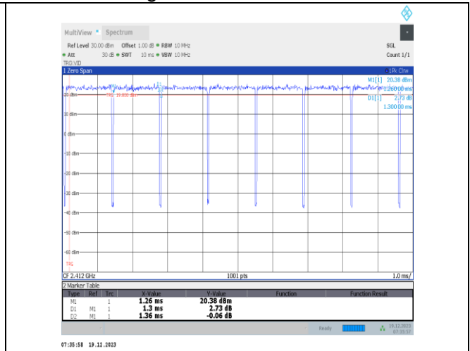
NTVN-11n20SISO-Ant3-2412
