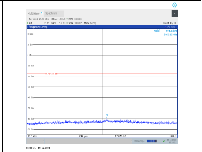
11ax20MIMO-Ant2-2462-30~1000-PASS
