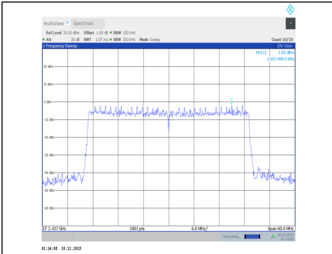
11ax40MIMO-Ant2-2437-0~Reference-PASS
