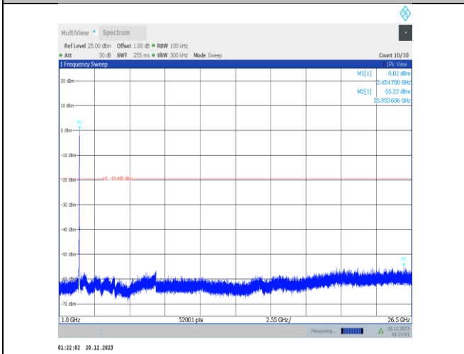
11ax40MIMO-Ant4-2452-1000~26500-PASS
