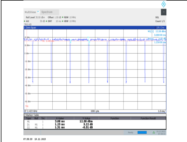
NTVN-11n40SISO-Ant2-2422
