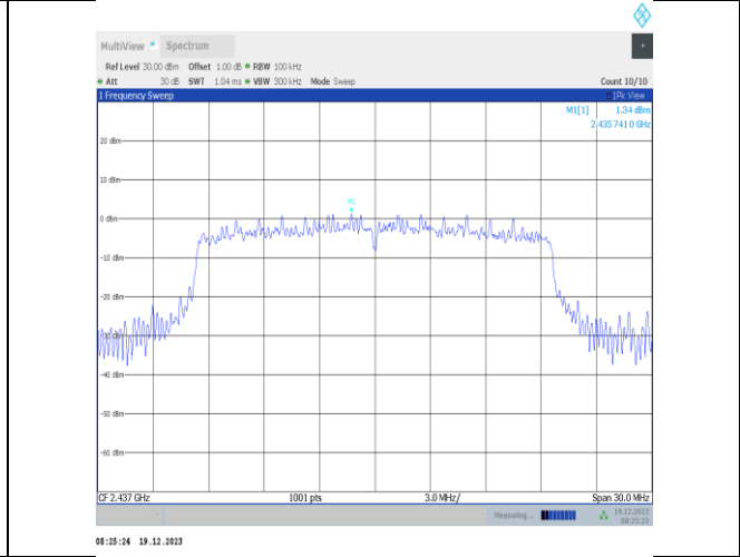
11ax20MIMO-Ant1-2437-0~Reference-PASS
