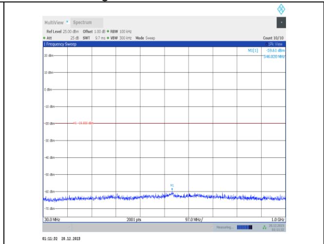
11ax40MIMO-Ant4-2422-30~1000-PASS
