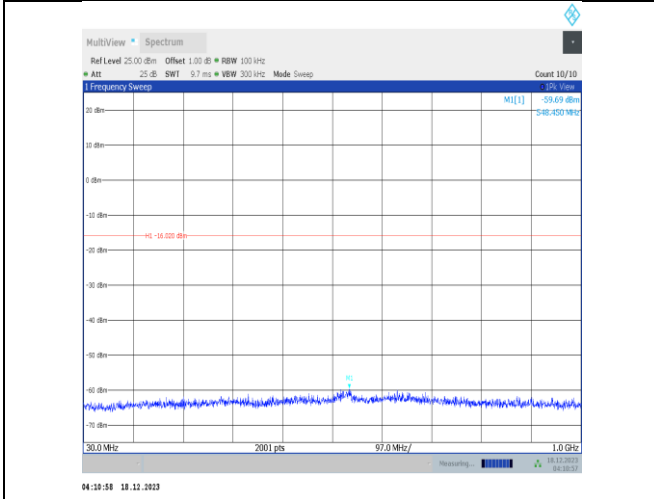
11n20SISO-Ant2-2462-30~1000-PASS
