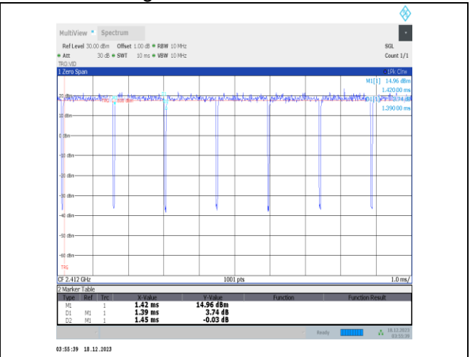
NTVN-11g-Ant1-2412
