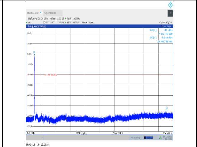
11n40SISO-Ant2-2437-1000~26500-PASS
