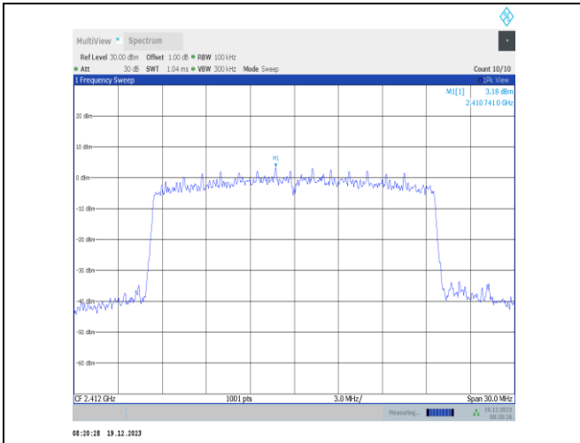
11ax20MIMO-Ant2-2412-0~Reference-PASS
