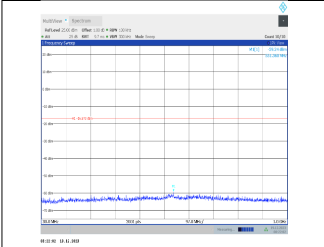
11ax20MIMO-Ant3-2412-30~1000-PASS
