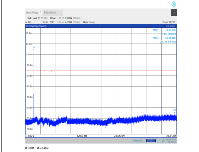
11ax20MIMO-Ant4-2412-1000~26500-PASS
