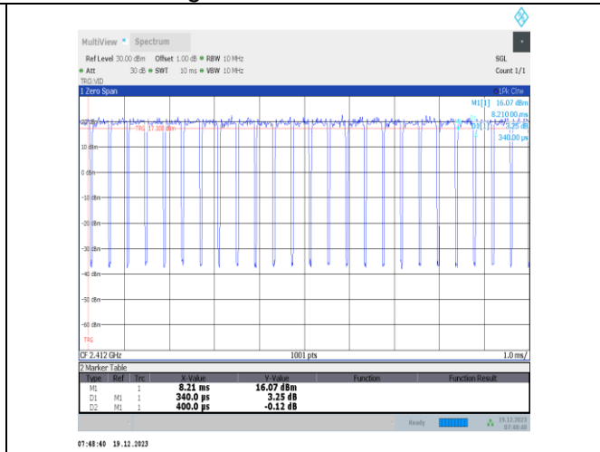
NTVN-11ax20MIMO-Ant1-2412
