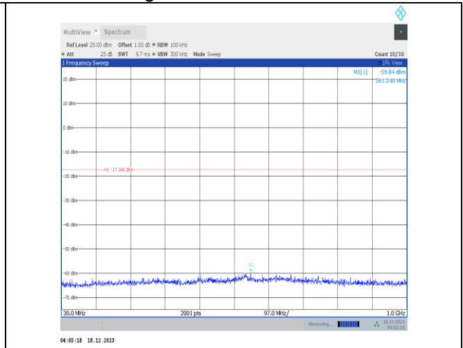
11n20SISO-Ant2-2437-30~1000-PASS
