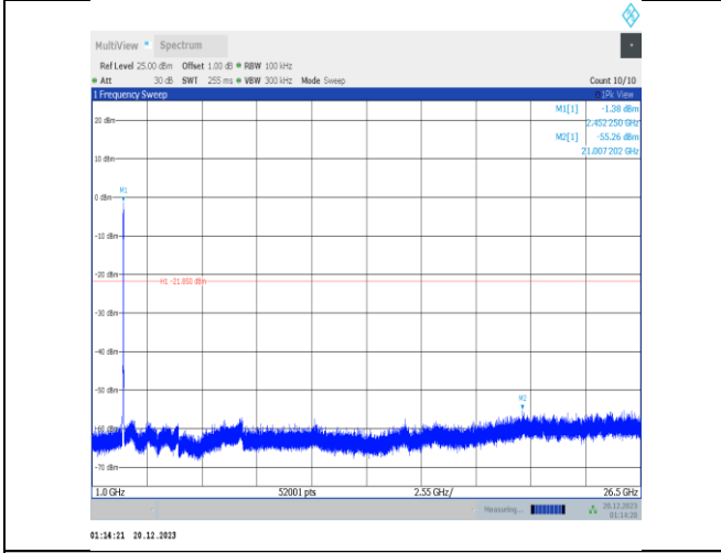
11ax40MIMO-Ant2-2437-1000~26500-PASS
