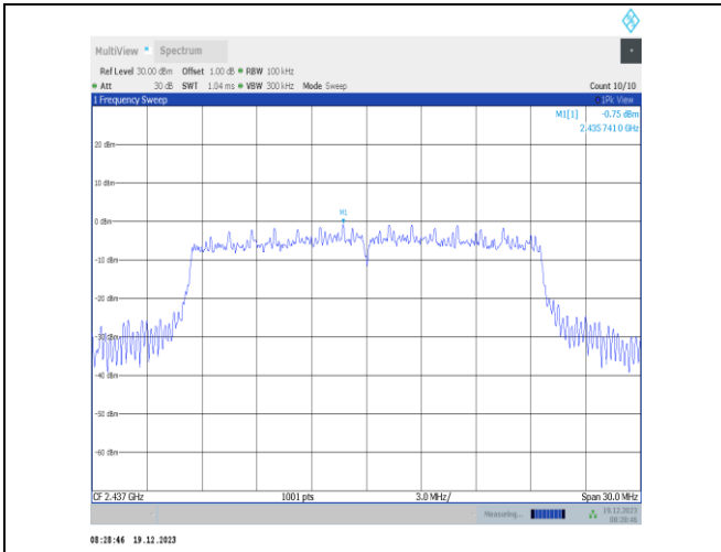
11ax20MIMO-Ant4-2437-0~Reference-PASS
