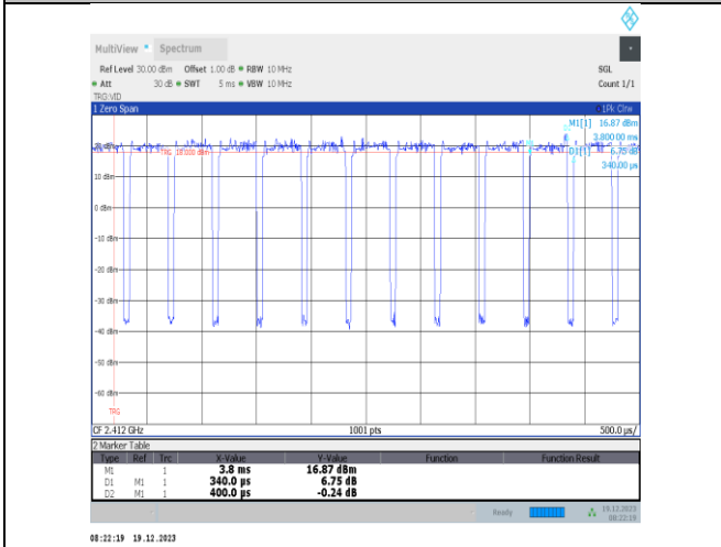
NTVN-11ax20MIMO-Ant4-2412
