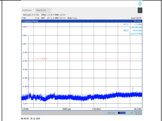
11ax20MIMO-Ant3-2462-1000~26500-PASS
