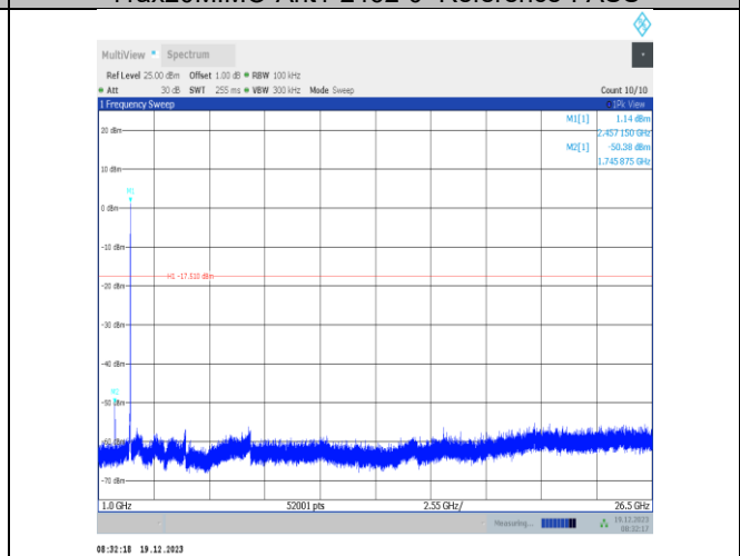
11ax20MIMO-Ant1-2462-1000~26500-PASS
