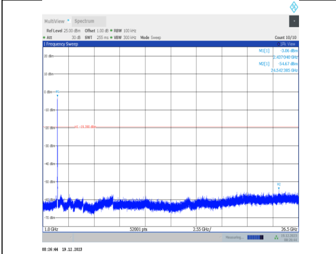
11ax20MIMO-Ant2-2437-1000~26500-PASS
