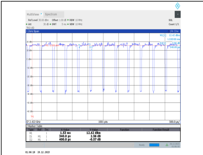
NTNV-11ax40MIMO-Ant2-2422
