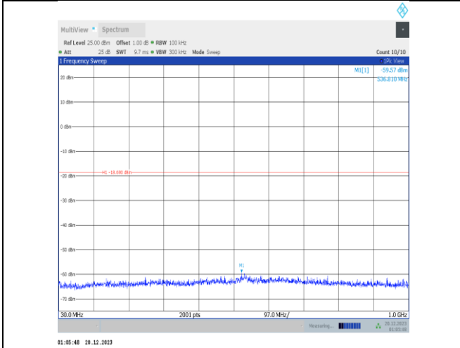
11ax40MIMO-Ant1-2422-30~1000-PASS
