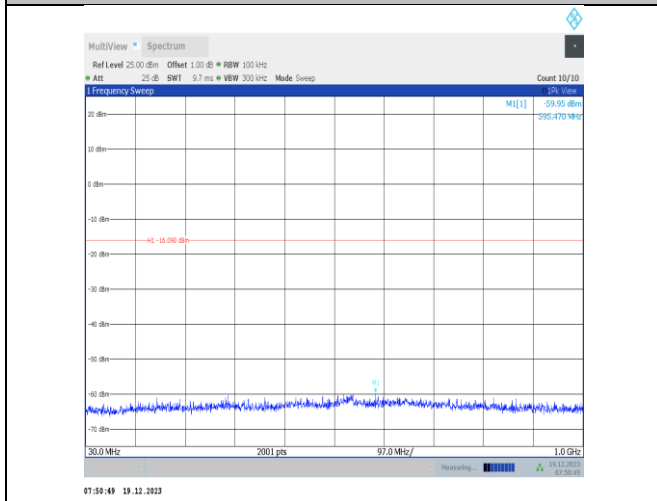
11ax20MIMO-Ant1-2412-30~1000-PASS
