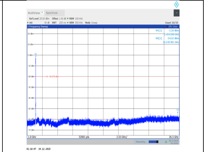
11ax40MIMO-Ant3-2422-1000~26500-PASS
