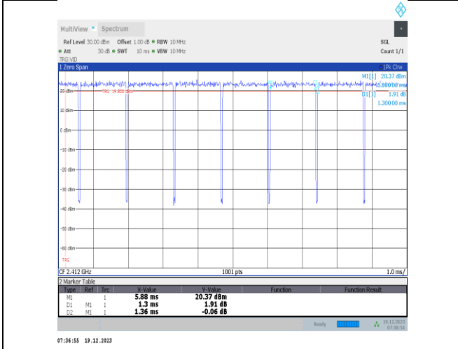
NTVN-11n20SISO-Ant4-2412
