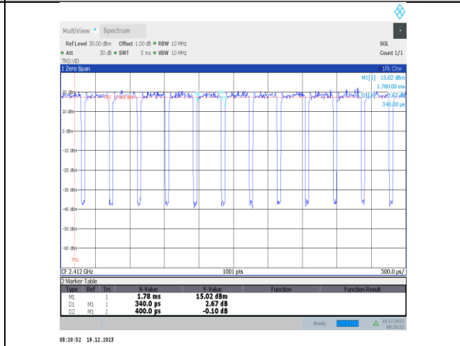
NTVN-11ax20MIMO-Ant3-2412
