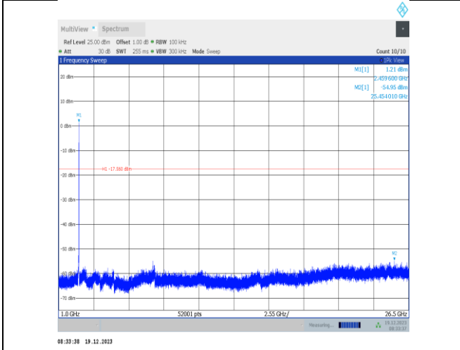
11ax20MIMO-Ant2-2462-1000~26500-PASS
