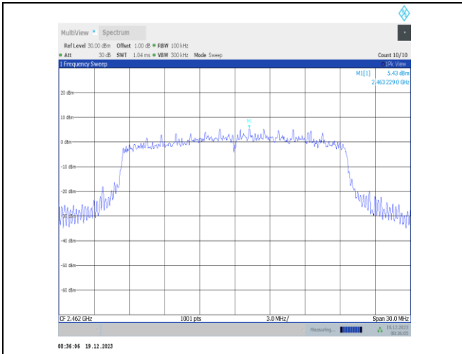
11ax20MIMO-Ant4-2462-0~Reference-PASS
