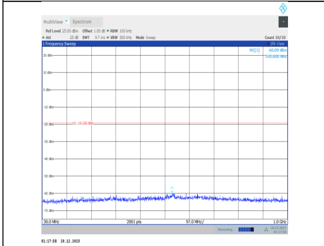
11ax40MIMO-Ant1-2452-30~1000-PASS
