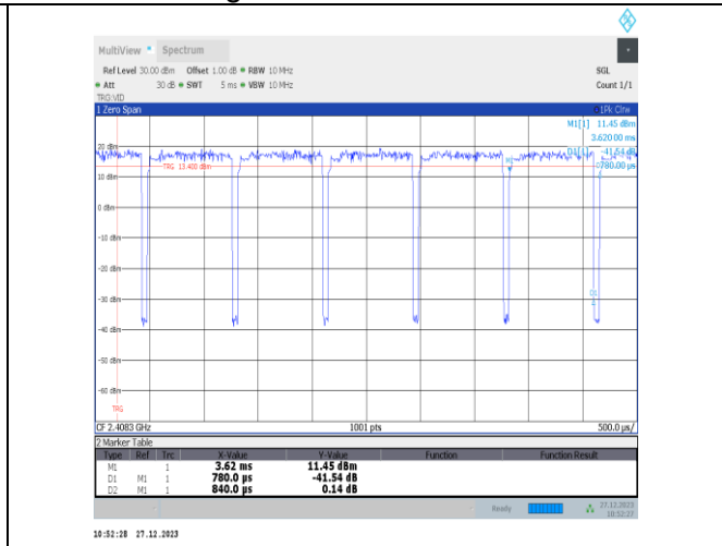
NTVN-11ax20MIMO-Ant2-2412-106Tone-RU53
