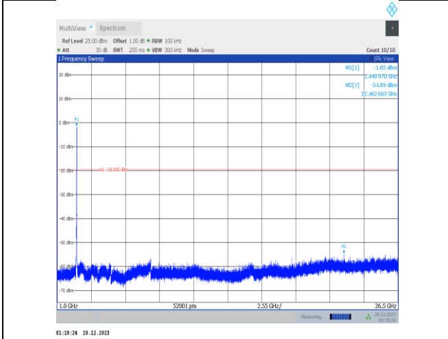
11ax40MIMO-Ant2-2452-1000~26500-PASS
