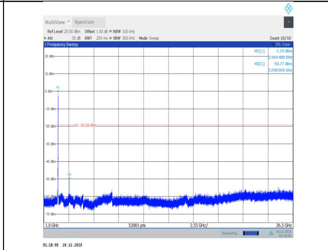
11ax40MIMO-Ant1-2452-1000~26500-PASS
