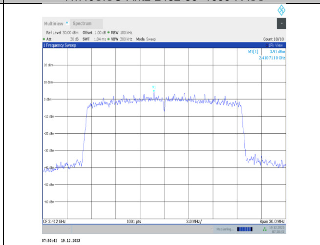
11ax20MIMO-Ant1-2412-0~Reference-PASS
