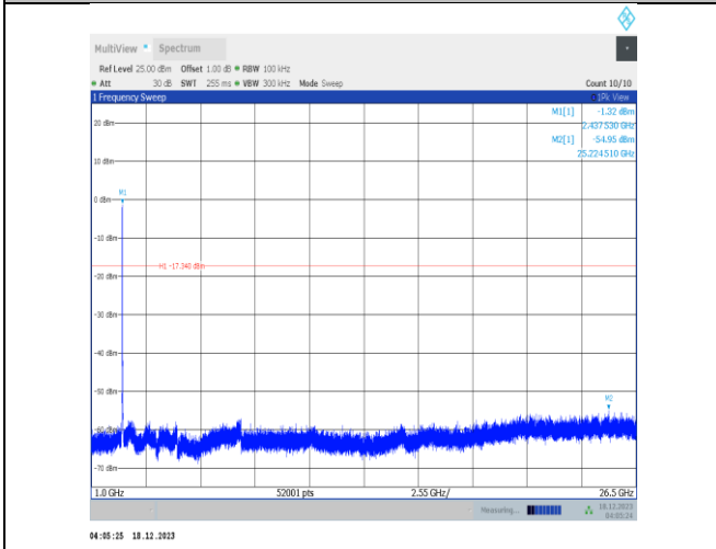
11n20SISO-Ant2-2437-1000~26500-PASS
