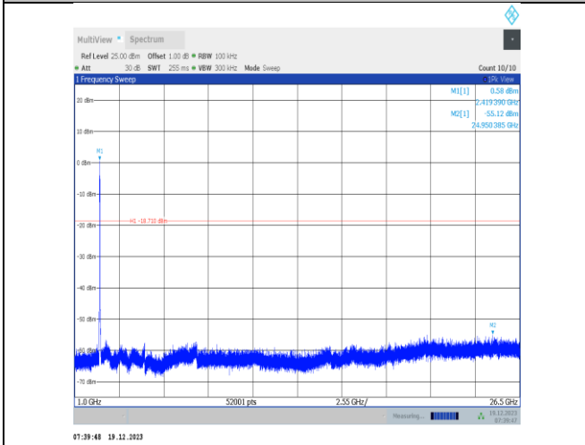
11n40SISO-Ant2-2422-1000~26500-PASS
