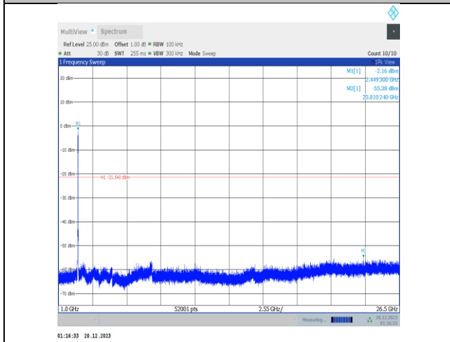
11ax40MIMO-Ant4-2437-1000~26500-PASS
