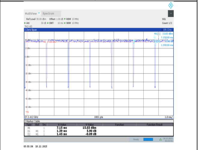
NTVN-11g-Ant3-2412
