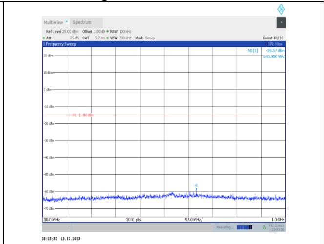
11ax20MIMO-Ant4-2412-30~1000-PASS
