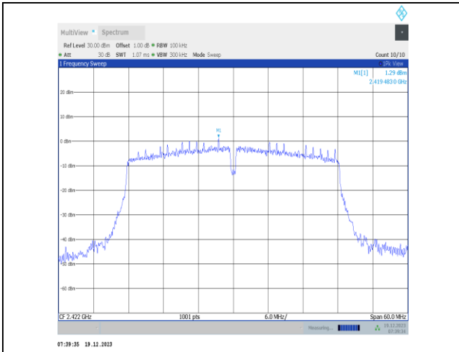
11n40SISO-Ant2-2422-0~Reference-PASS
