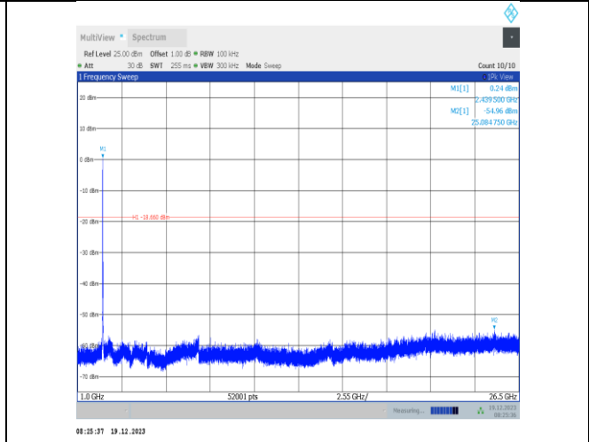
11ax20MIMO-Ant1-2437-1000~26500-PASS
