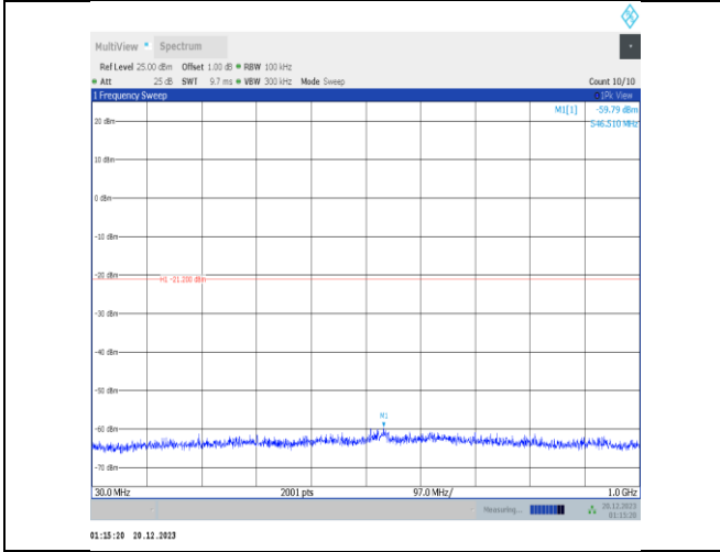
11ax40MIMO-Ant3-2437-30~1000-PASS
