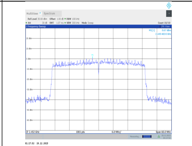
11ax40MIMO-Ant1-2452-0~Reference-PASS
