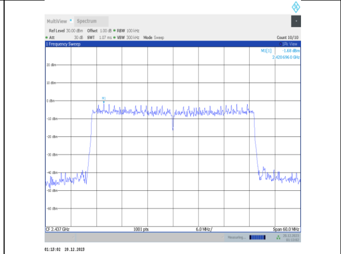
11ax40MIMO-Ant1-2437-0~Reference-PASS
