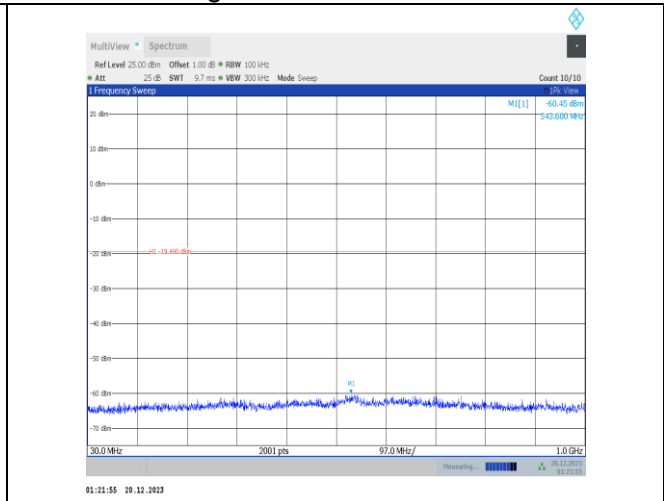
11ax40MIMO-Ant4-2452-30~1000-PASS
