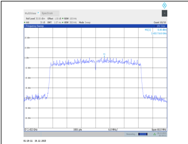
11ax40MIMO-Ant2-2452-0~Reference-PASS
