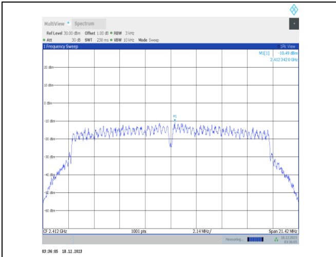
11g-Ant2-2412-PASS
