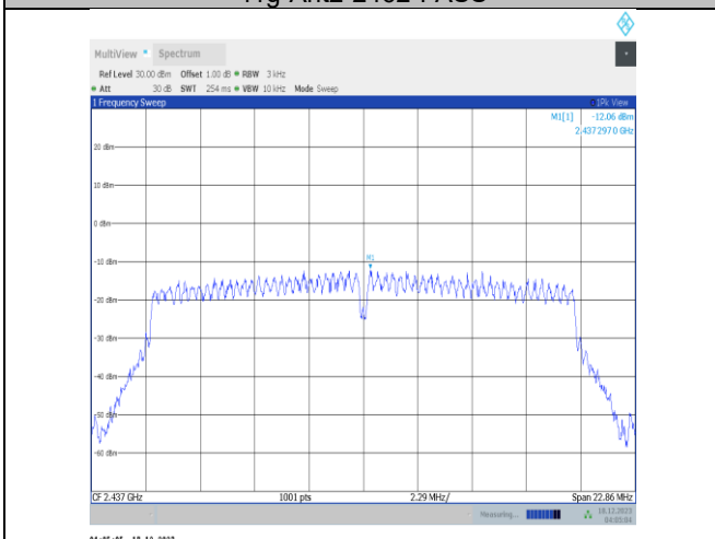
11n20SISO-Ant2-2437-PASS
