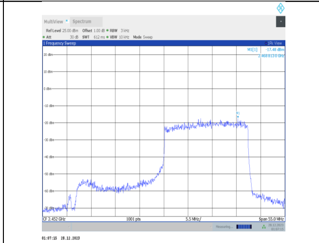
11ax40MIMO-Ant2-2452-242Tone-RU62-PASS
