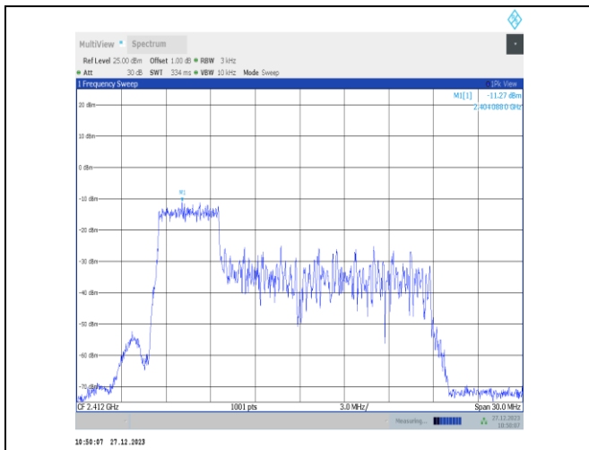
11ax20MIMO-Ant4-2412-52Tone-RU37-PASS
