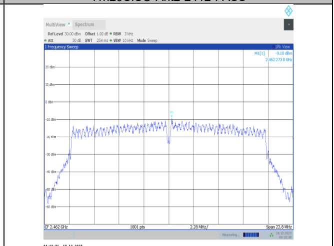
11n20SISO-Ant2-2462-PASS
