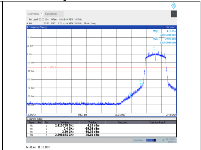
11n20SISO-Ant2-2412-PASS
