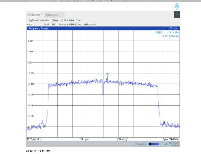
11ax40MIMO-Ant1-2422-PASS
