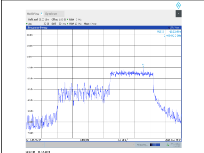
11ax20MIMO-Ant1-2462-106Tone-RU54-PASS
