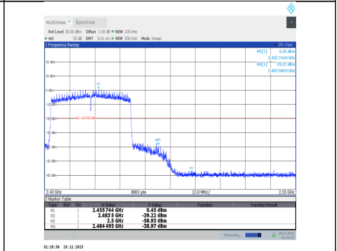
11ax40MIMO-Ant1-2452-PASS
