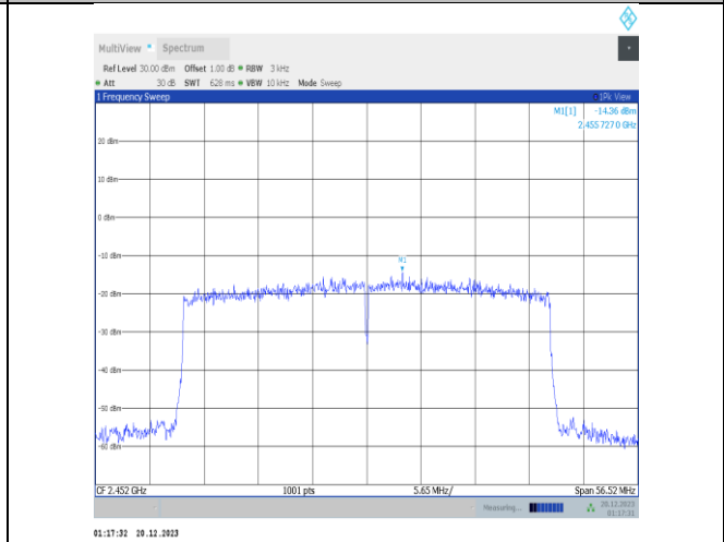
11ax40MIMO-Ant1-2452-PASS
