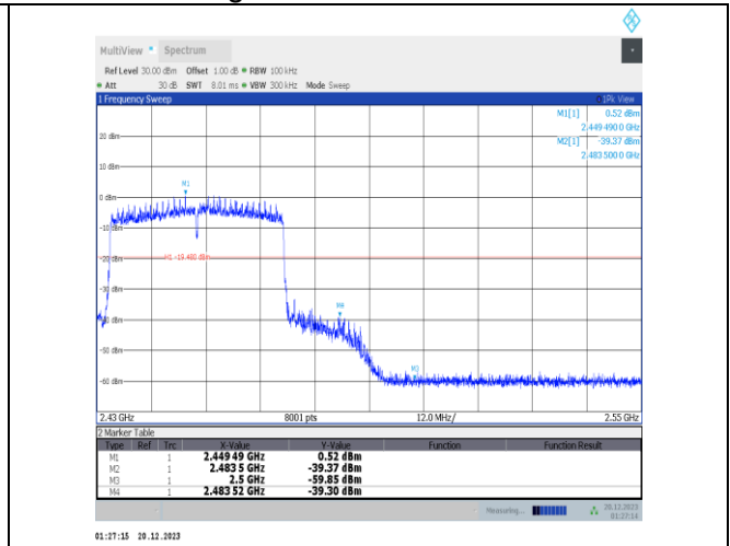
11ax40MIMO-Ant3-2452-PASS
