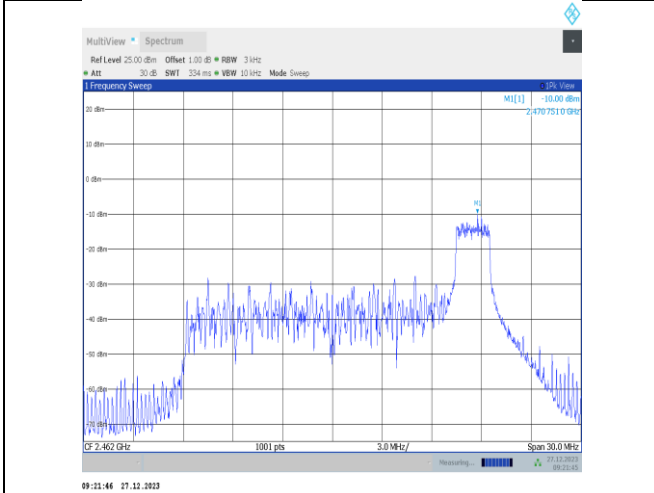
11ax20MIMO-Ant1-2462-26Tone-RU8-PASS
