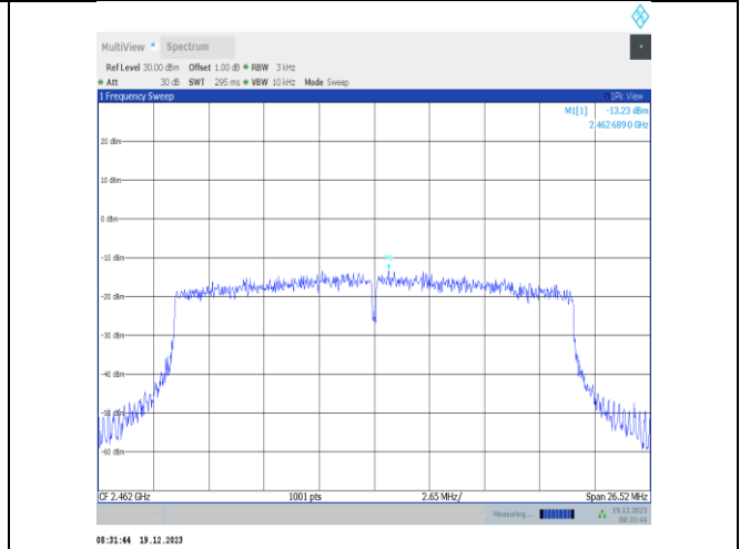
11ax20MIMO-Ant1-2462-PASS
