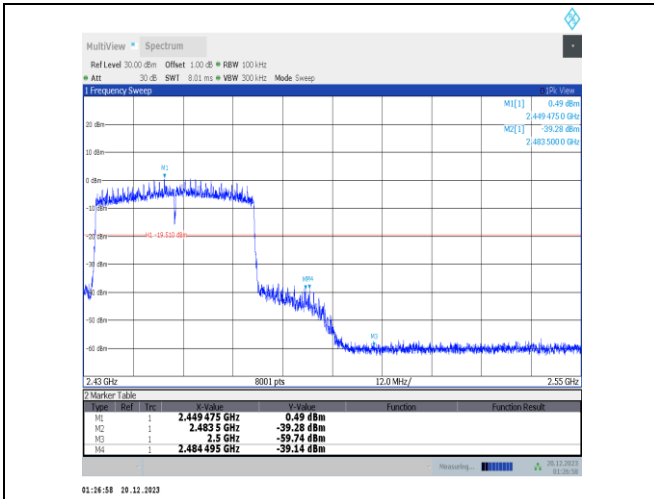
11ax40MIMO-Ant2-2452-PASS
