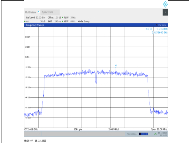
11ax20MIMO-Ant2-2412-PASS
