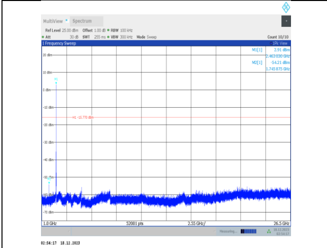
11b-Ant2-2462-1000~26500-PASS
