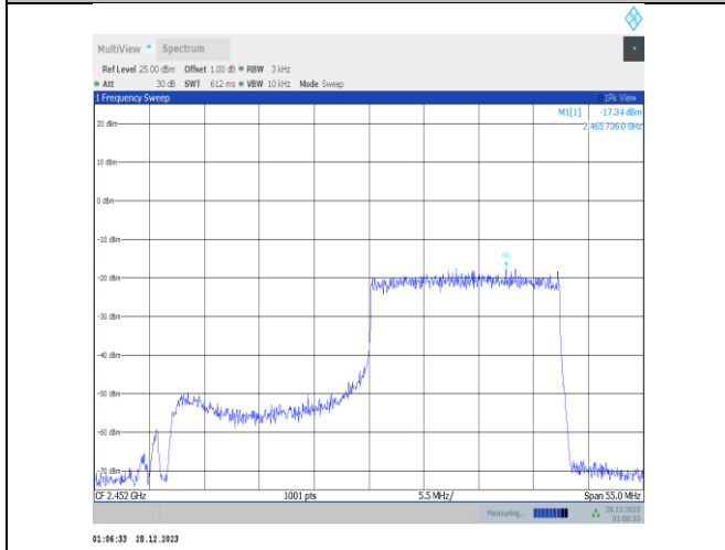
11ax40MIMO-Ant1-2452-242Tone-RU62-PASS
