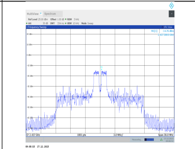
11ax20MIMO-Ant2-2437-26Tone-RU4-PASS
