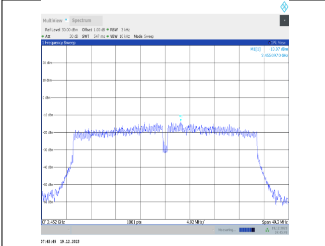
11n40SISO-Ant2-2452-PASS
