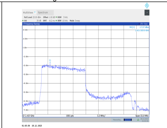
11ax40MIMO-Ant2-2437-242Tone-RU61-PASS
