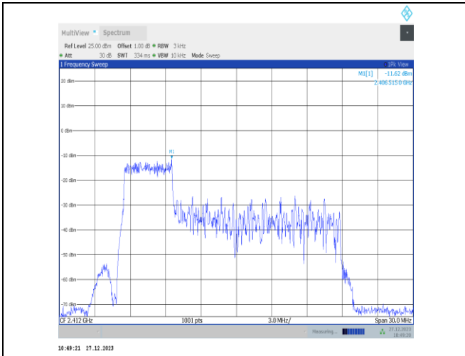
11ax20MIMO-Ant2-2412-52Tone-RU37-PASS
