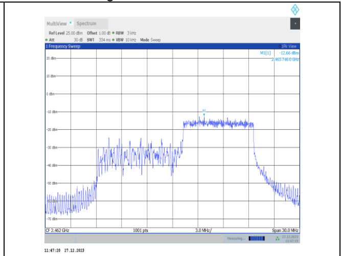
11ax20MIMO-Ant4-2462-106Tone-RU54-PASS
