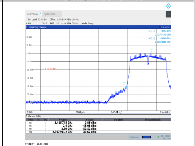
11n40SISO-Ant2-2422-PASS
