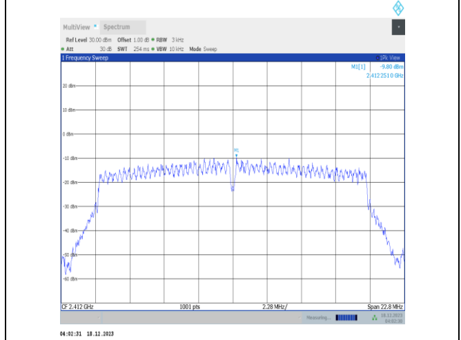
11n20SISO-Ant2-2412-PASS
