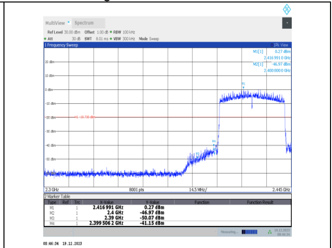
11ax40MIMO-Ant1-2422-PASS
