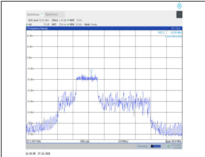
11ax20MIMO-Ant4-2437-52Tone-RU38-PASS
