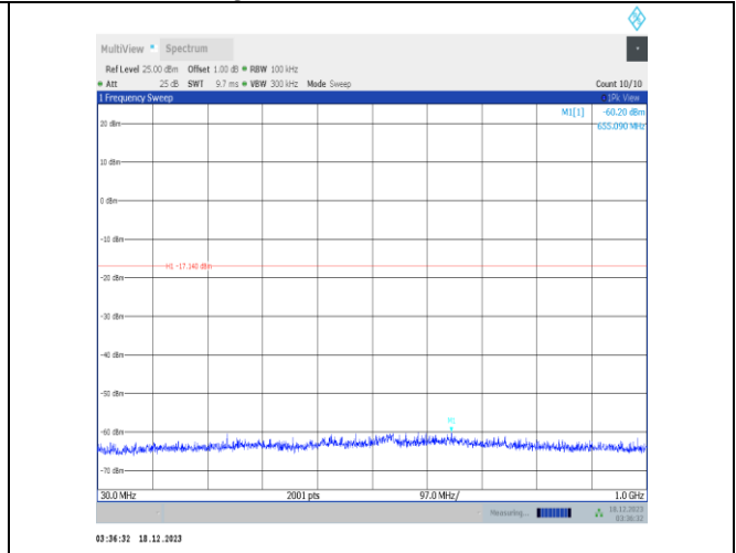
11g-Ant2-2412-30~1000-PASS
