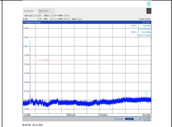
11n20SISO-Ant2-2412-1000~26500-PASS
