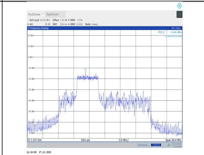
11ax20MIMO-Ant1-2437-52Tone-RU38-PASS
