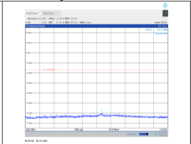
11g-Ant2-2462-30~1000-PASS
