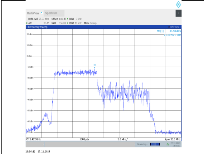
11ax20MIMO-Ant3-2412-106Tone-RU53-PASS
