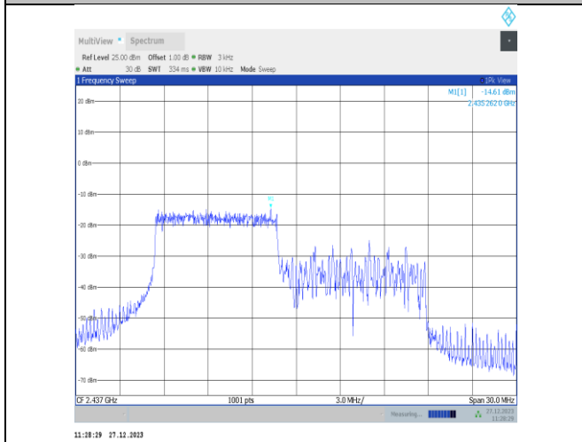
11ax20MIMO-Ant1-2437-106Tone-RU53-PASS
