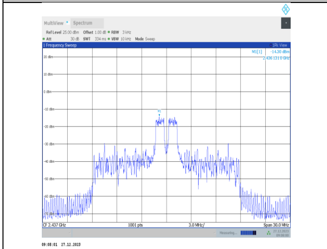
11ax20MIMO-Ant1-2437-26Tone-RU4-PASS
