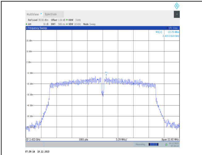
11n40SISO-Ant2-2422-PASS
