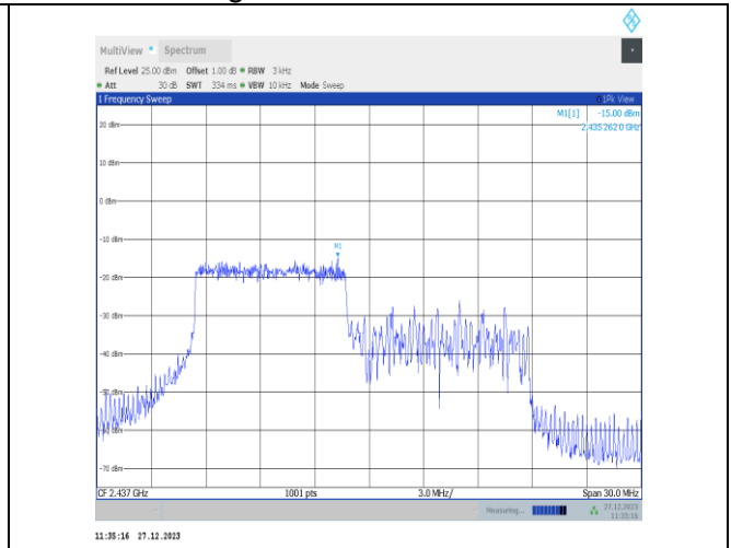
11ax20MIMO-Ant4-2437-106Tone-RU53-PASS
