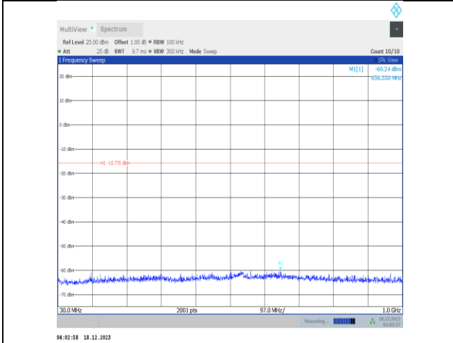
11n20SISO-Ant2-2412-30~1000-PASS
