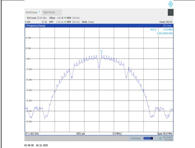
11b-Ant2-2462-0~Reference-PASS
