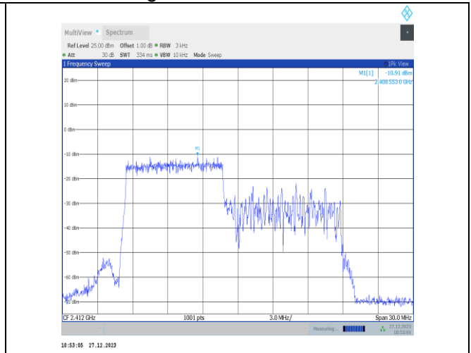
11ax20MIMO-Ant2-2412-106Tone-RU53-PASS
