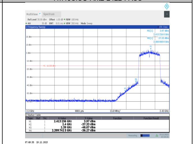
11x20MIMO-Ant1-2412-PASS
