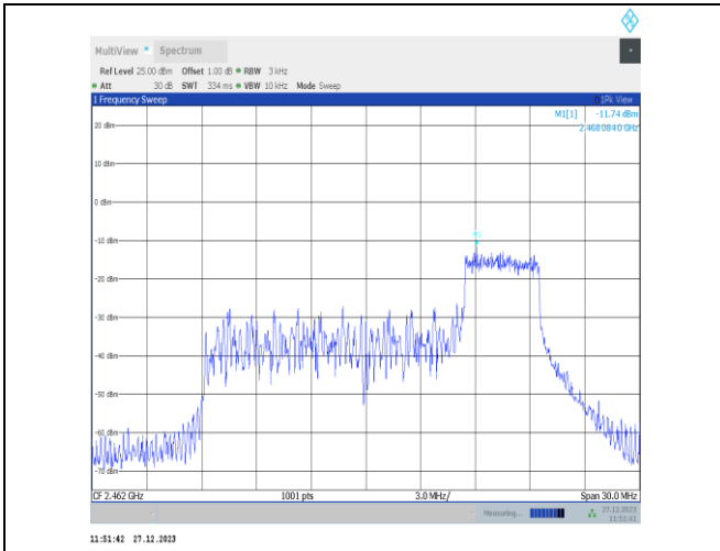
11ax20MIMO-Ant4-2462-52Tone-RU40-PASS
