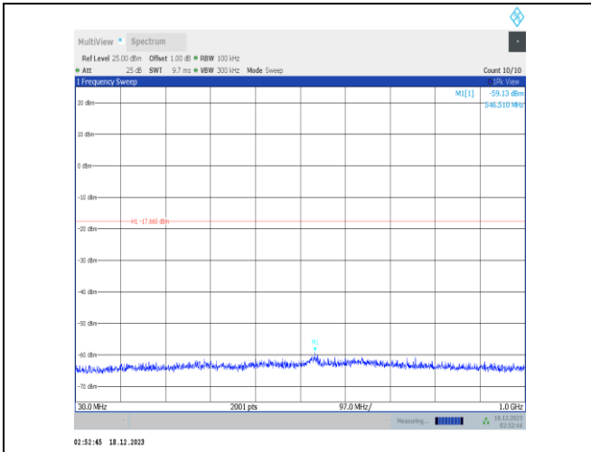
11b-Ant2-2437-30~1000-PASS
