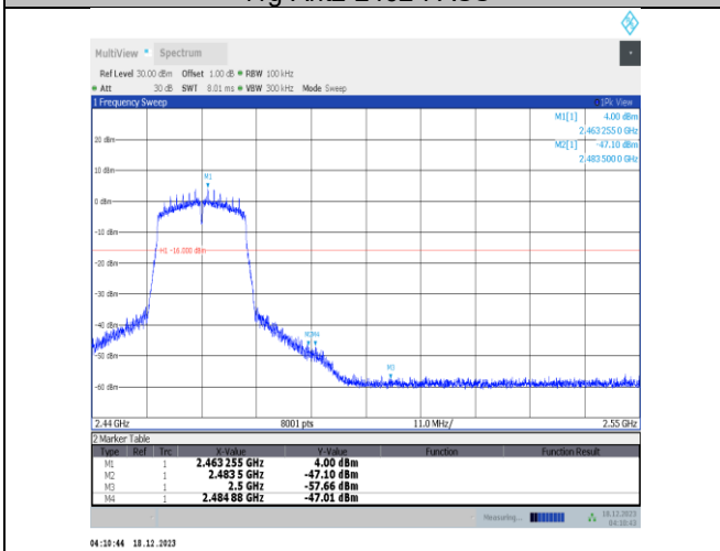
11n20SISO-Ant2-2462-PASS
